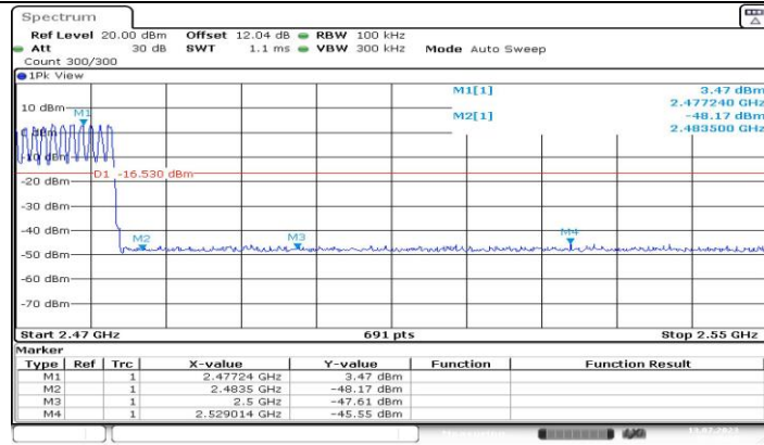
DH5_Ant1_High_Hop_2480
