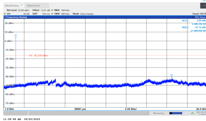
3DH5_Ant1_2480_1000~26500
