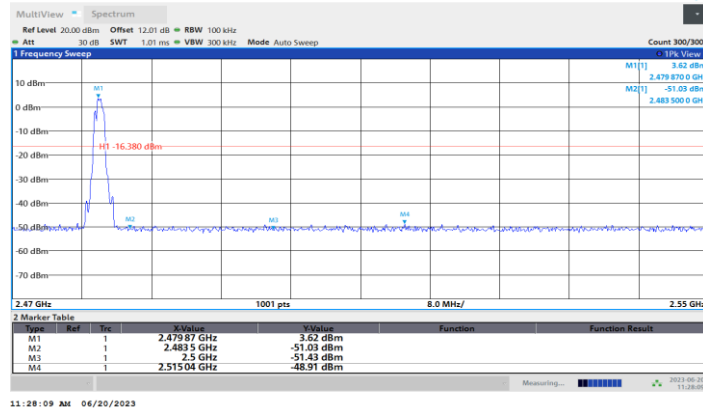
3DH5_Ant1_High_2480
