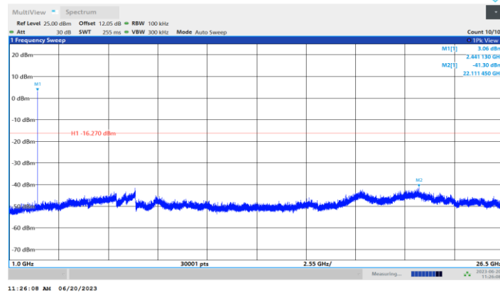
3DH5_Ant1_2441_1000~26500
