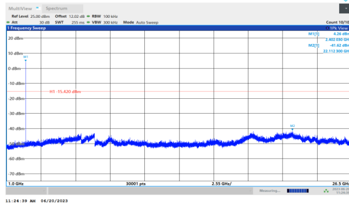
3DH5_Ant1_2402_1000~26500
