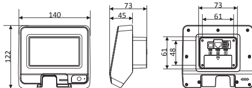
Figure 5: device dimensions (mm)
