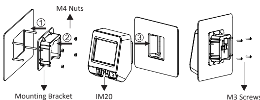
Figure 6: installation and mounting
