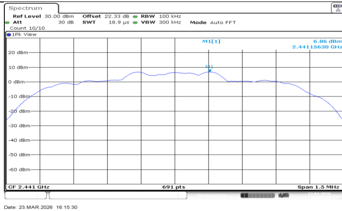
3DH5_Ant1_2441_0~Reference
