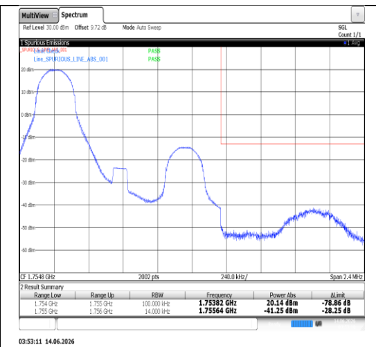
Band4-1.4MHz-QPSK-20393-6RB#0-PASS
