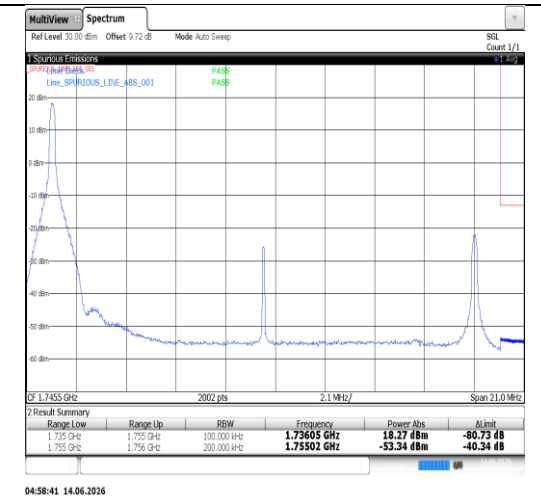
Band4-20MHz-16QAM-20300-100RB#0-PASS
