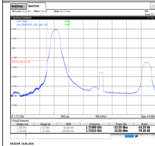
Band4-3MHz-QPSK-19965-15RB#0-PASS
