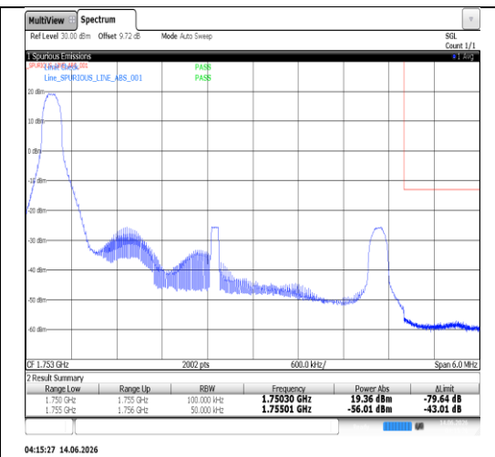
Band4-5MHz-QPSK-20375-25RB#0-PASS
