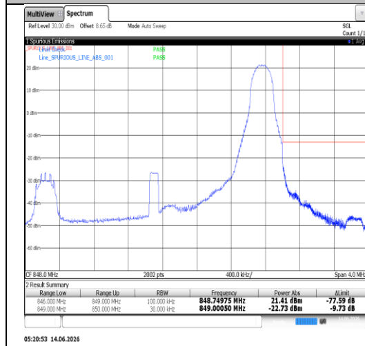
Band5-3MHz-16QAM-20415-1RB#0-PASS
