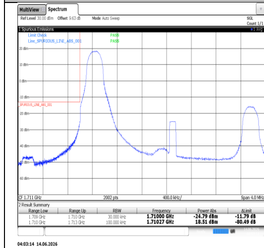
Band4-3MHz-16QAM-19965-15RB#0-PASS
