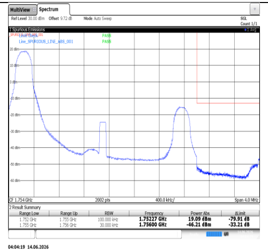
Band4-3MHz-16QAM-20385-15RB#0-PASS
