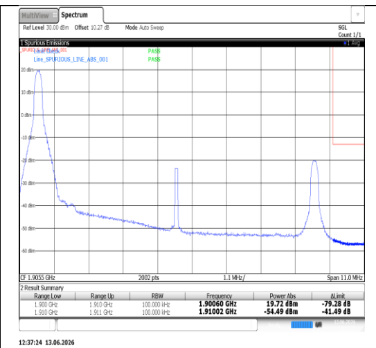
Band2-10MHz-16QAM-19150-50RB#0-PASS
