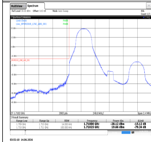
Band4-1.4MHz-QPSK-19957-6RB#0-PASS
