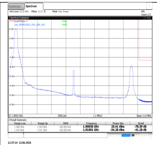
Band2-10MHz-QPSK-19150-50RB#0-PASS
