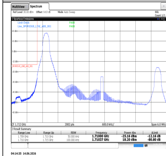
Band4-5MHz-16QAM-19975-25RB#0-PASS
