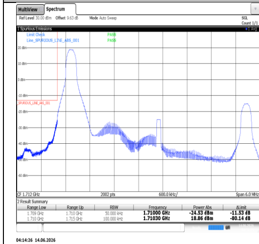
Band4-5MHz-QPSK-19975-25RB#0-PASS
