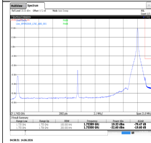
Band4-20MHz-16QAM-20050-1RB#0-PASS
