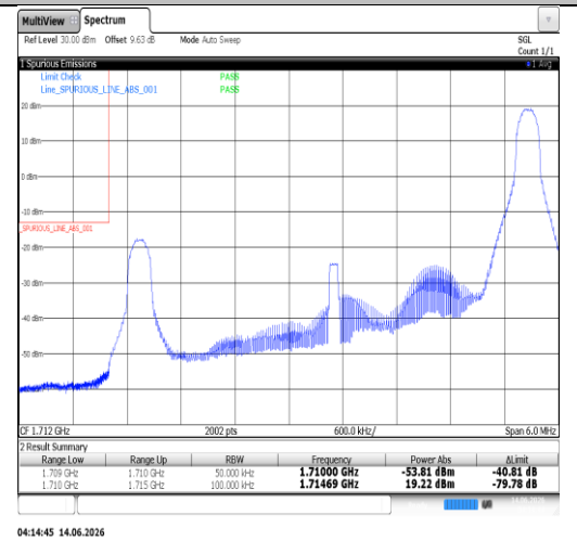
Band4-5MHz-QPSK-20375-1RB#0-PASS
