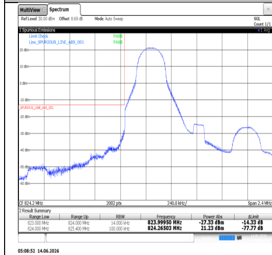
Band5-1.4MHz-QPSK-20407-6RB#0-PASS
