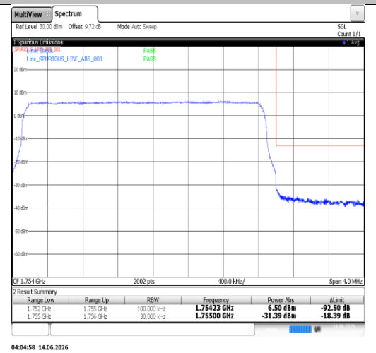
Band4-5MHz-QPSK-19975-1RB#24-PASS
