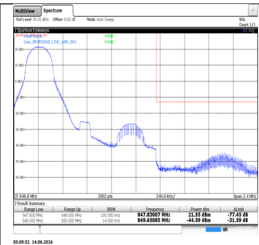
Band5-1.4MHz-QPSK-20643-6RB#0-PASS
