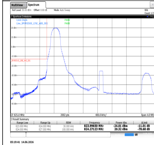
Band5-3MHz-16QAM-20415-15RB#0-PASS
