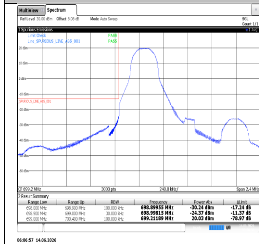
Band12-1.4MHz-16QAM-23017-6RB#0-PASS
