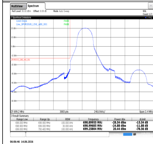
Band12-1.4MHz-QPSK-23017-6RB#0-PASS
