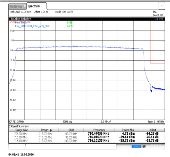
Band17-10MHz-16QAM-23780-1RB#49-PASS
