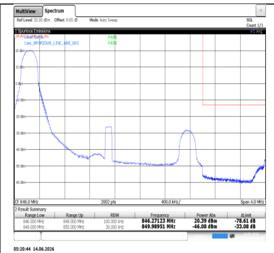
Band5-3MHz-16QAM-20635-15RB#0-PASS
