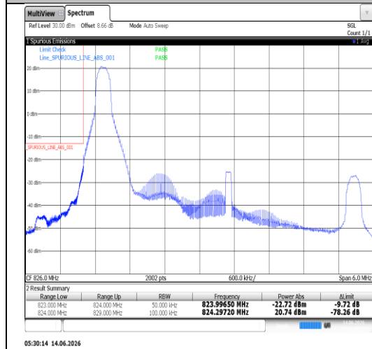
Band5-5MHz-QPSK-20425-25RB#0-PASS
