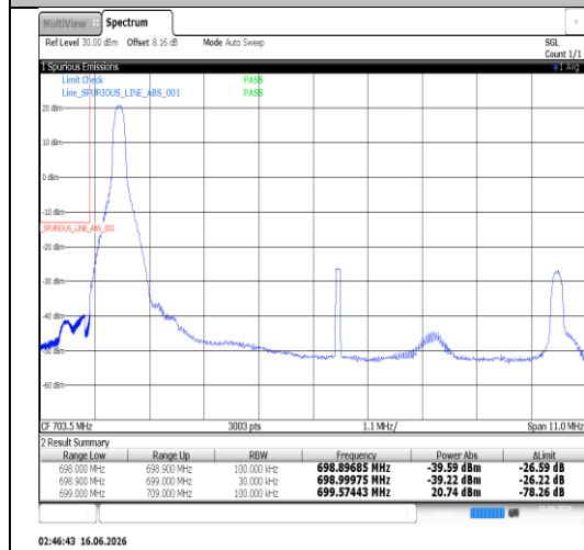
Band12-10MHz-QPSK-23060-50RB#0-PASS
