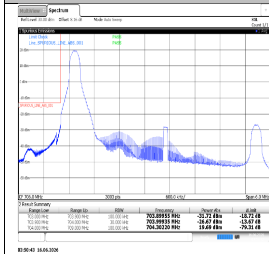
Band17-5MHz-16QAM-23755-25RB#0-PASS
