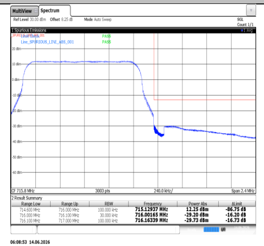
Band12-3MHz-QPSK-23025-1RB#14-PASS
