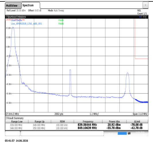
Band5-10MHz-16QAM-20600-50RB#0-PASS
