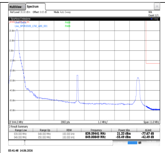
Band5-10MHz-QPSK-20600-50RB#0-PASS
