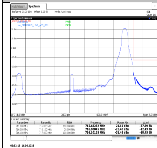
Band17-10MHz-QPSK-23780-1RB#0-PASS
