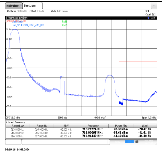
Band12-3MHz-16QAM-23165-15RB#0-PASS
