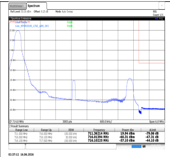
Band12-5MHz-16QAM-23155-25RB#0-PASS
