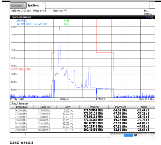
Band13-5MHz-QPSK-23205-25RB#0-PASS
