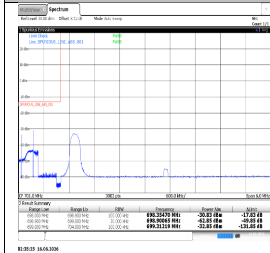
Band12-5MHz-QPSK-23035-25RB#0-PASS
