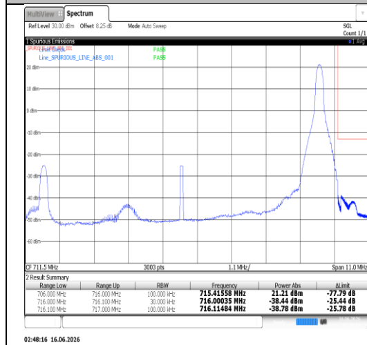
Band12-10MHz-16QAM-23060-1RB#0-PASS
