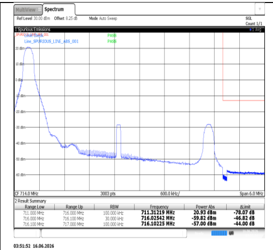
Band17-5MHz-16QAM-23825-25RB#0-PASS
