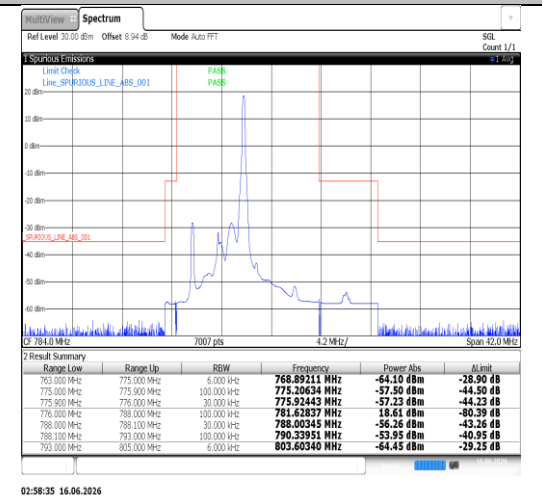
Band13-5MHz-QPSK-23255-1RB#0-PASS
