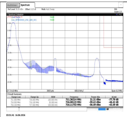
Band17-5MHz-QPSK-23825-25RB#0-PASS
