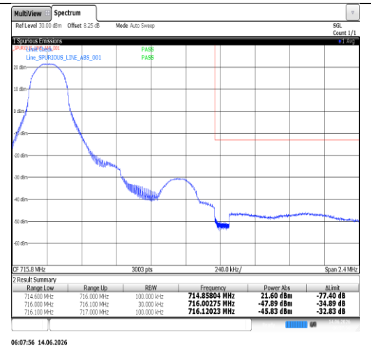
Band12-1.4MHz-QPSK-23173-6RB#0-PASS
