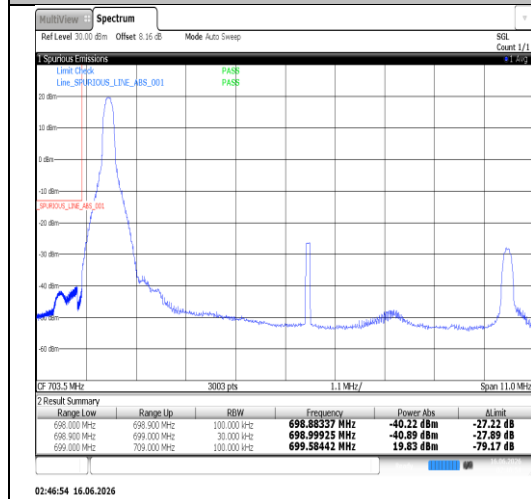
Band12-10MHz-16QAM-23060-50RB#0-PASS
