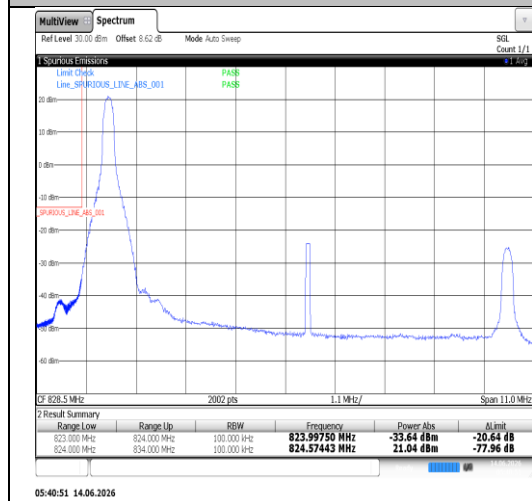
Band5-10MHz-QPSK-20450-50RB#0-PASS
