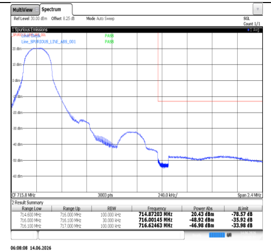
Band12-1.4MHz-16QAM-23173-6RB#0-PASS
