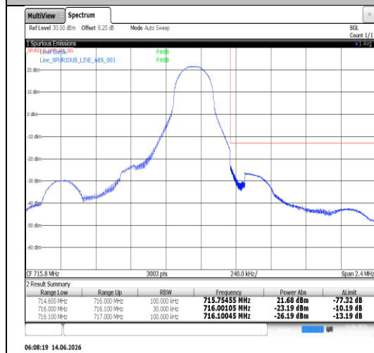
Band12-1.4MHz-16QAM-23017-1RB#0-PASS
