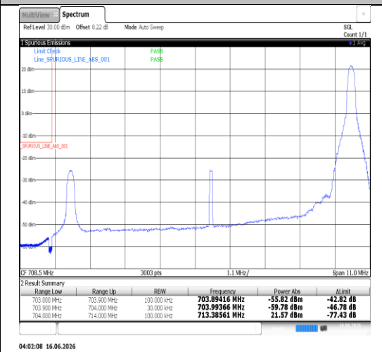
Band17-10MHz-QPSK-23800-1RB#0-PASS
