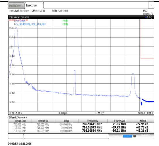
Band17-10MHz-QPSK-23800-50RB#0-PASS
