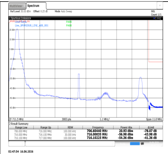
Band12-10MHz-QPSK-23130-50RB#0-PASS
