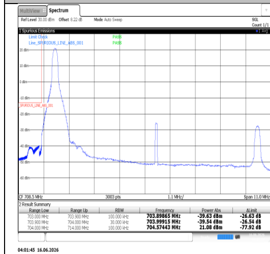
Band17-10MHz-QPSK-23780-50RB#0-PASS
