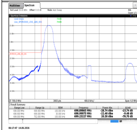
Band12-3MHz-QPSK-23025-15RB#0-PASS
