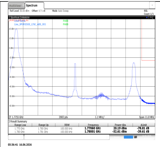
Band66-10MHz-16QAM-132622-50RB#0- PASS
