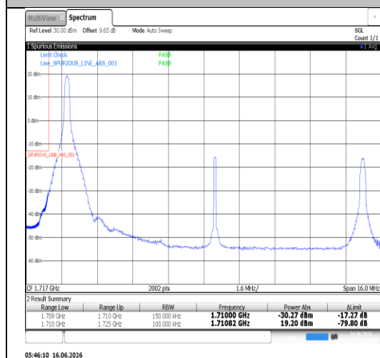
Band66-15MHz-16QAM-132047-75RB#0-PASS
