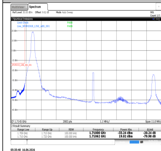
Band66-10MHz-16QAM-132022-50RB#0-PASS
