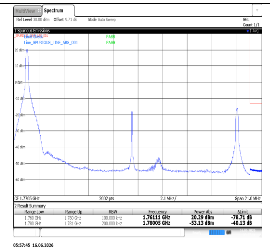
Band66-20MHz-QPSK-132572-100RB#0-PASS
