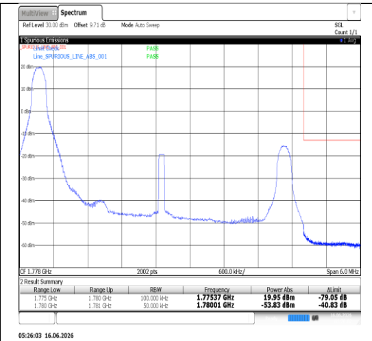
Band66-5MHz-16QAM-132647-25RB#0-PASS
