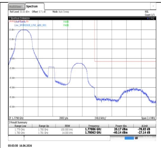
Band66-1.4MHz-16QAM-132665-6RB#0-PASS
