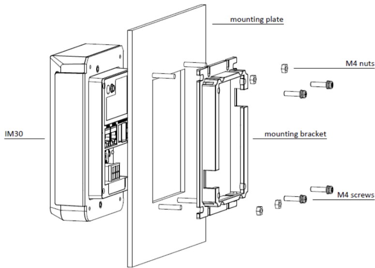
Figure 9: device installation
