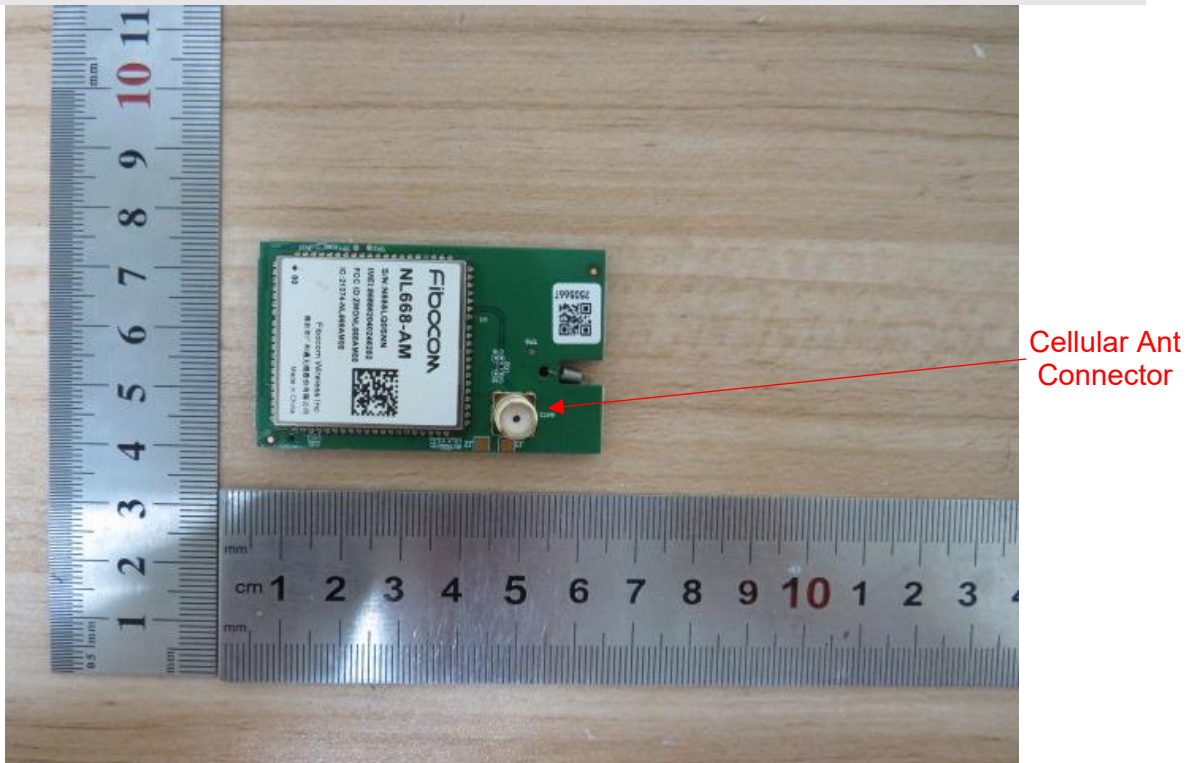
Internal View of EUT-19
