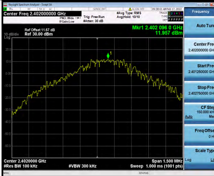
DH5_Ant1_2402_0~Reference
