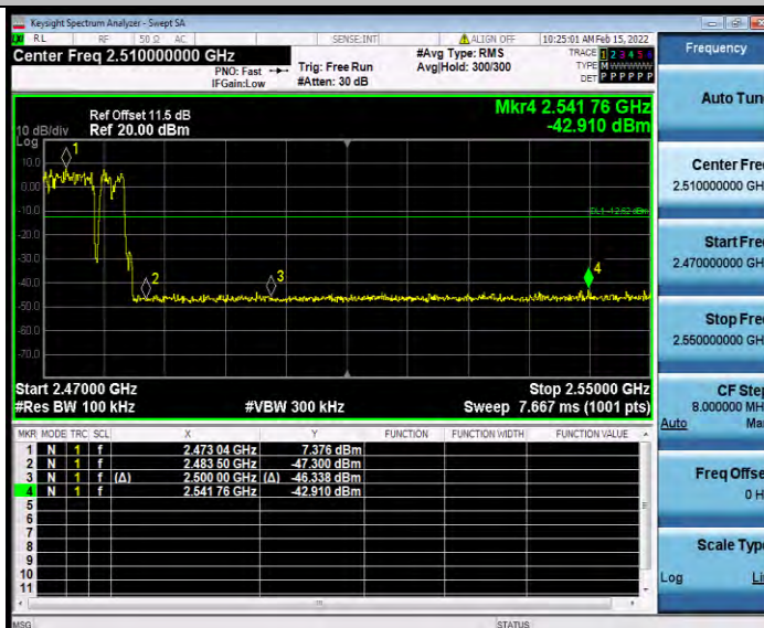
2DH5_Ant1_High_Hop_2480
