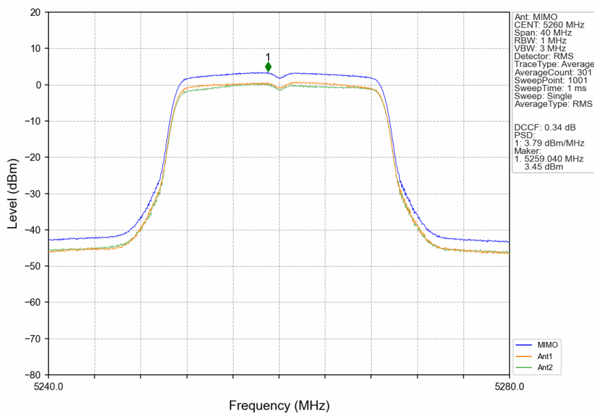
802.11ac(VHT20)_LCH_5260MHz_MIMO_NTNV
