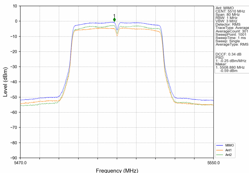
802.11n(HT40)_LCH_5510MHz_MIMO_NTNV
