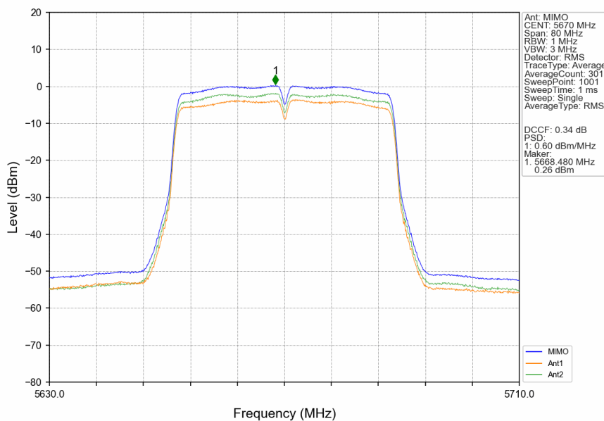
802.11n(HT40)_HCH_5670MHz_MIMO_NTNV
