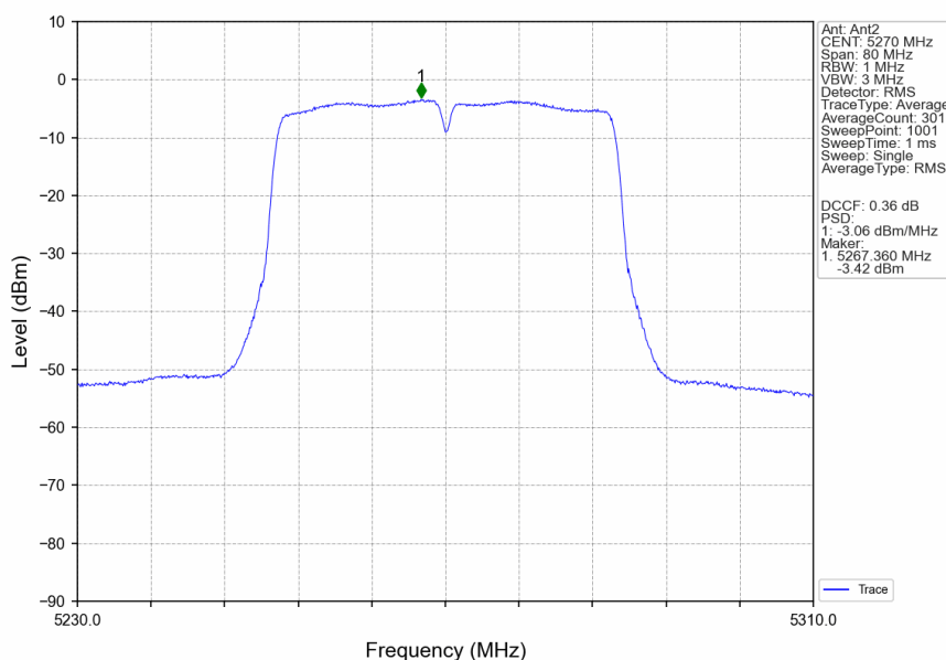
802.11ac(VHT40)_LCH_5270MHz_MIMO_NTNV
