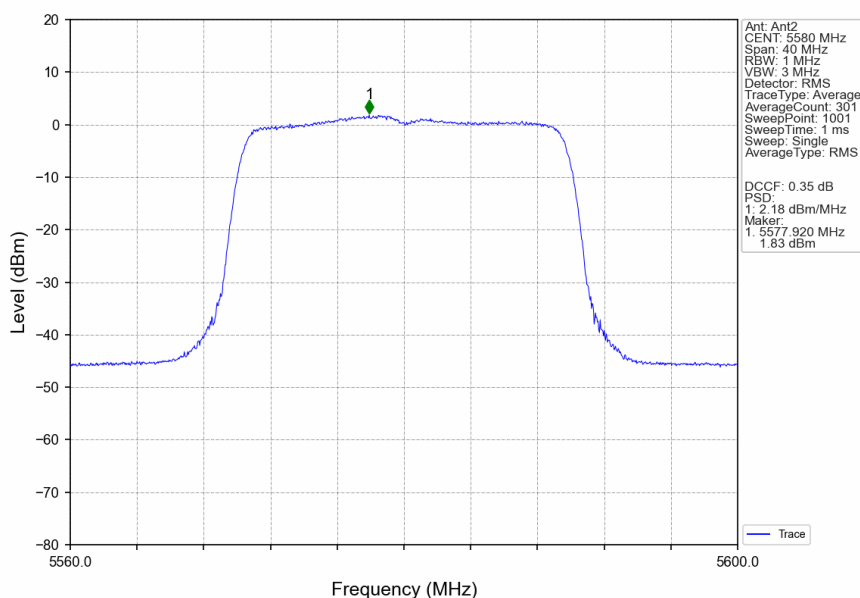
802.11ax(HEW20)_MCH_5580MHz_SU_/_MIMO_NTNV
