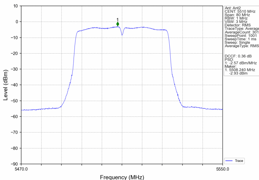
802.11ac(VHT40)_LCH_5510MHz_MIMO_NTNV
