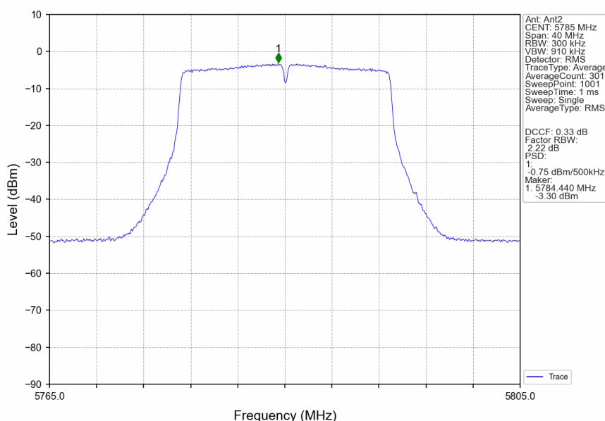
802.11ac(VHT20)_MCH_5785MHz_Ant2_NTNV
