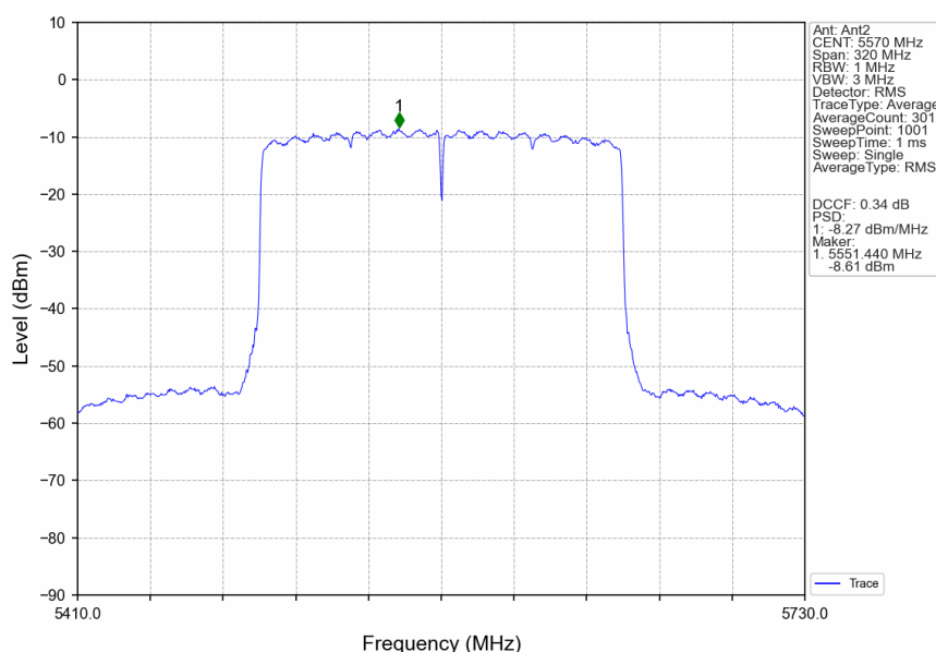
802.11ax(HEW160)_MCH_5570MHz_SU_/_Ant2_NTNV
