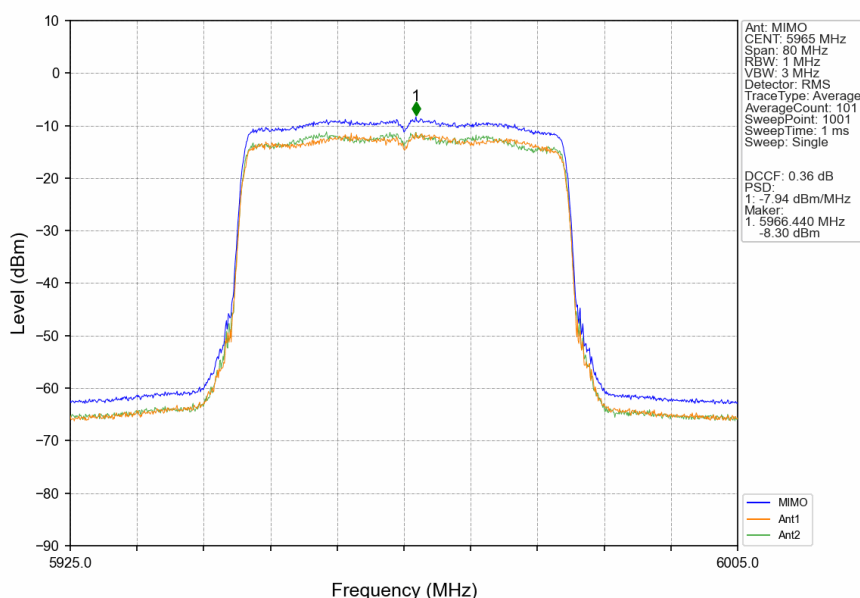
802.11ax(HEW40)_LCH_5965MHz_RU484_Left_MIMO_NTNV
