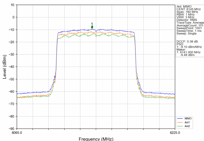
802.11ax(HEW80)_MCH_6145MHz_RU996_Left_MIMO_NTNV
