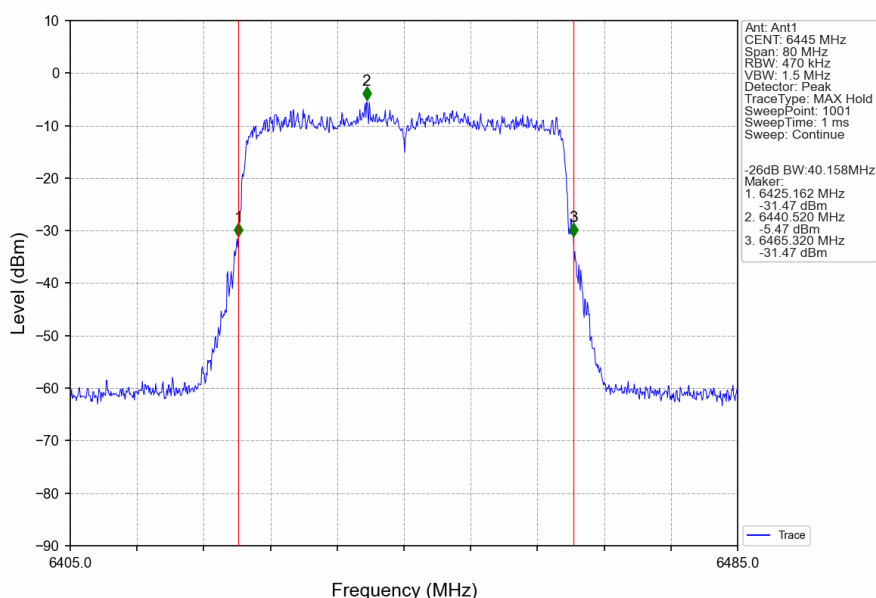
802.11ax(HEW40)_LCH_6445MHz_RU484_Left_Ant1_NTNV
