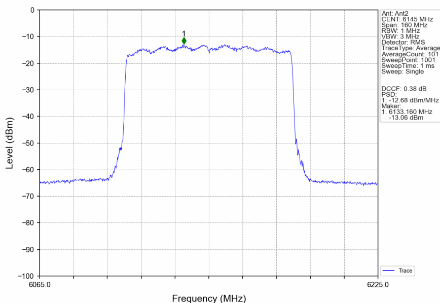
802.11ax(HEW80)_MCH_6145MHz_RU996_Left_MIMO_NTNV
