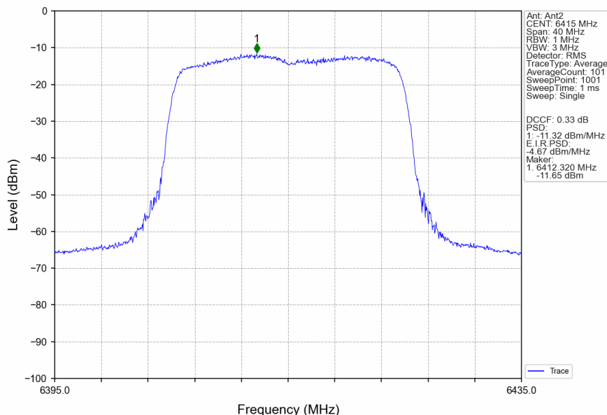
802.11ax(HEW20)_HCH_6415MHz_RU242_Left_Ant2_NTNV
