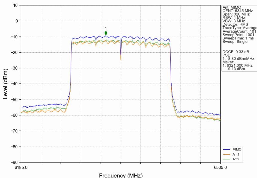
802.11ax(HEW160)_HCH_6345MHz_2xRU996_Left_MIMO_NTNV
