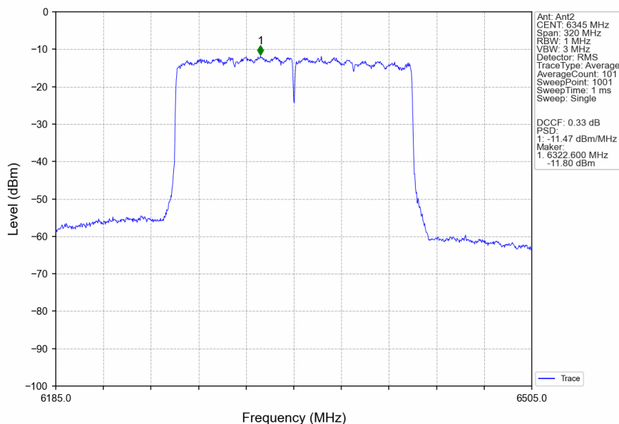
802.11ax(HEW160)_HCH_6345MHz_2xRU996_Left_MIMO_NTNV
