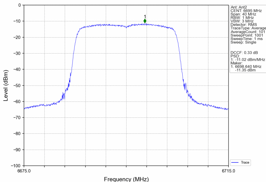
802.11ax(HEW20)_MCH_6695MHz_RU242_Left_MIMO_NTNV
