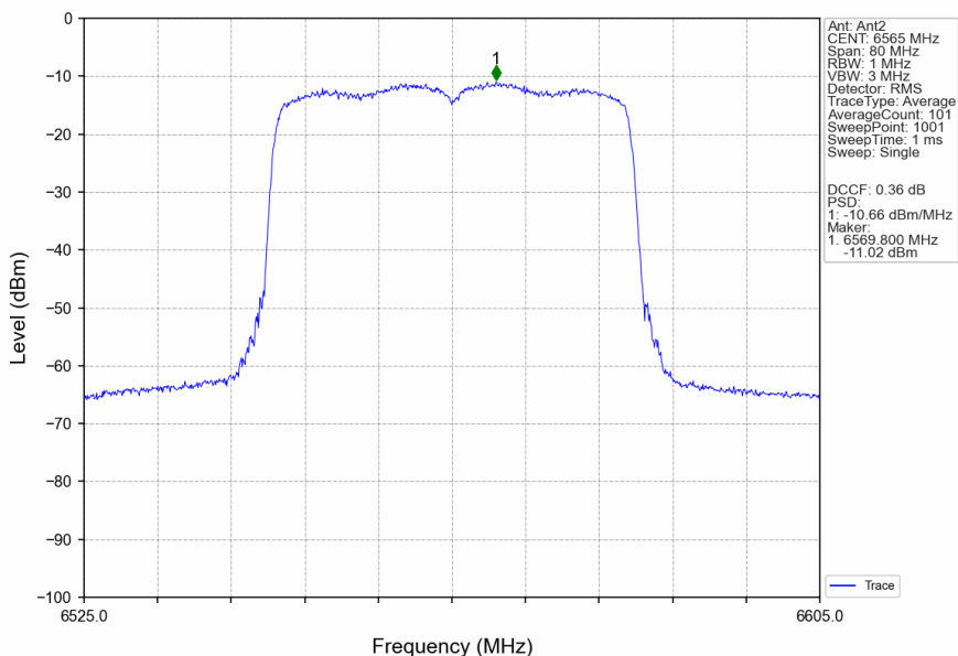
802.11ax(HEW40)_LCH_6565MHz_RU484_Left_MIMO_NTNV
