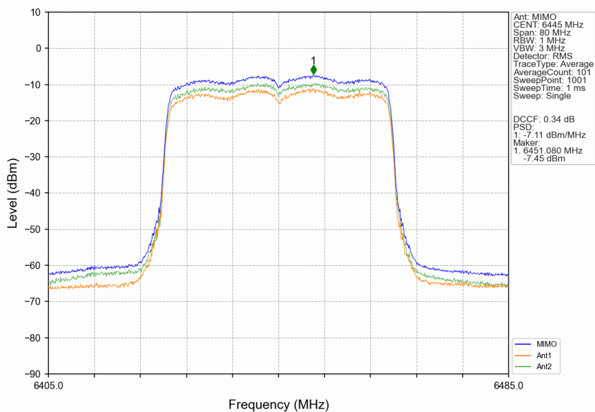
802.11ax(HEW40)_LCH_6445MHz_RU484_Left_MIMO_NTNV
