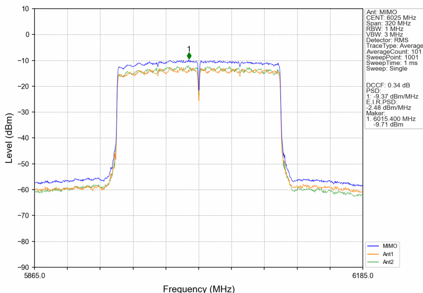
802.11ax(HEW160)_LCH_6025MHz_2xRU996_Left_MIMO_NTNV
