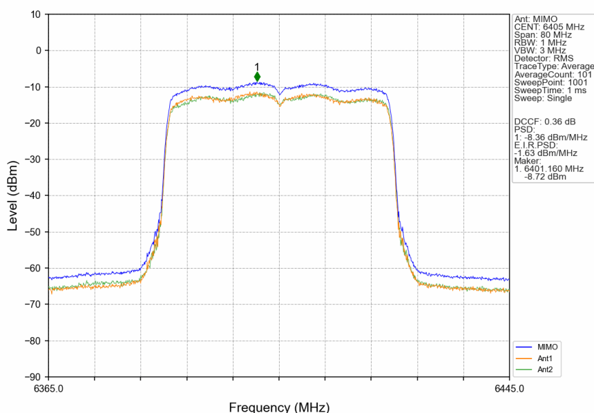
802.11ax(HEW40)_HCH_6405MHz_RU484_Left_MIMO_NTNV
