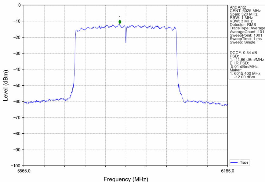
802.11ax(HEW160)_LCH_6025MHz_2xRU996_Left_MIMO_NTNV
