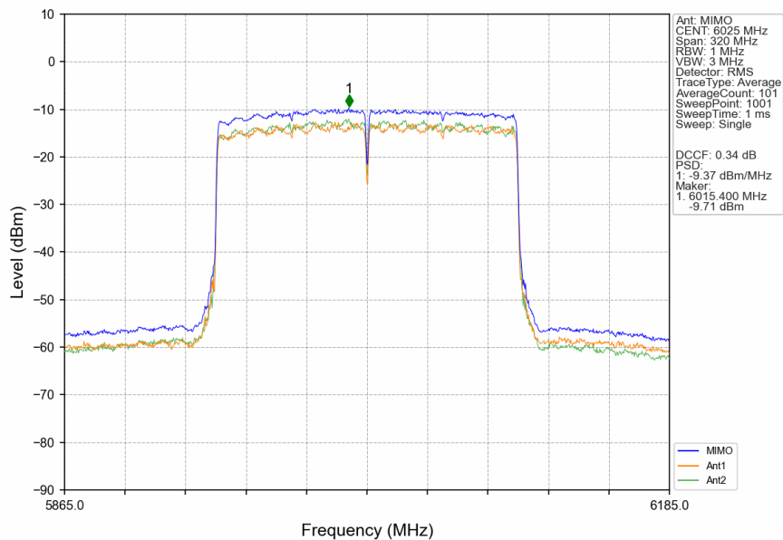
802.11ax(HEW160)_LCH_6025MHz_2xRU996_Left_MIMO_NTNV
