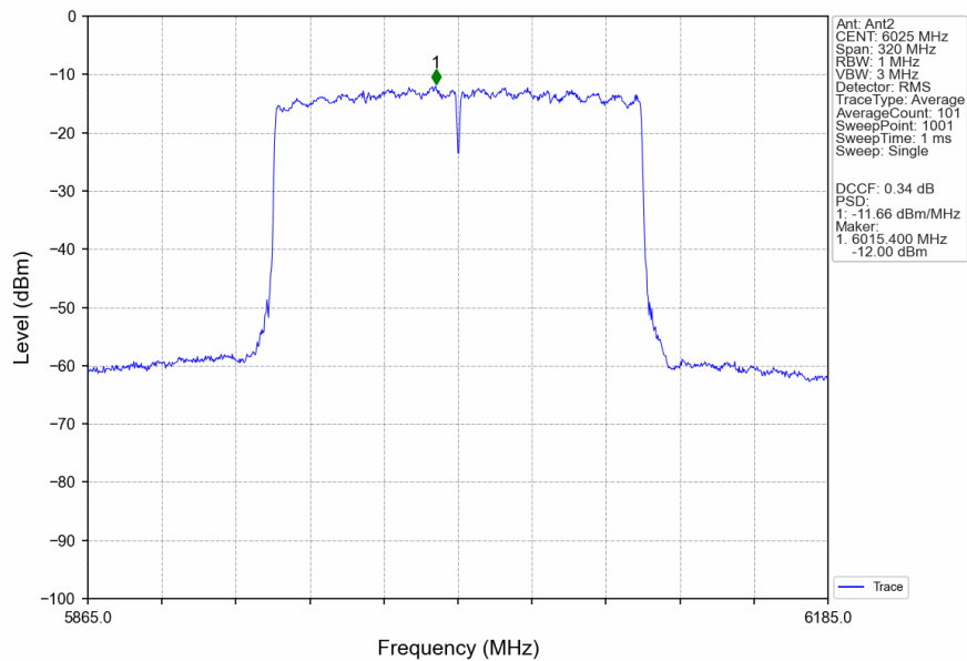
802.11ax(HEW160)_LCH_6025MHz_2xRU996_Left_MIMO_NTNV
