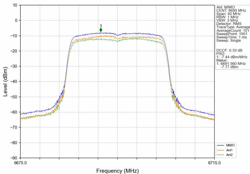
802.11ax(HEW20)_MCH_6695MHz_RU242_Left_MIMO_NTNV
