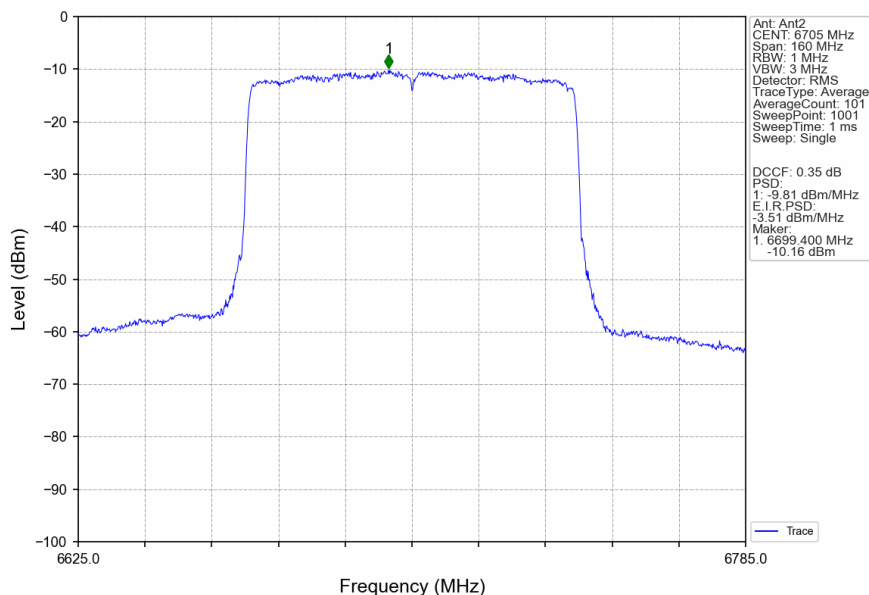
802.11ax(HEW80)_MCH_6705MHz_RU996_Left_MIMO_NTNV
