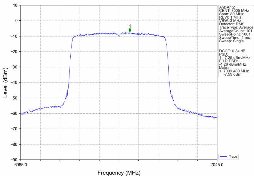
802.11ax(HEW40)_MCH_7005MHz_RU484_Left_Ant2_NTNV
