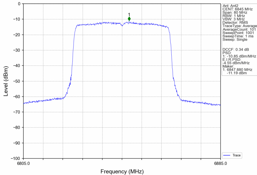
802.11ax(HEW40)_HCH_6845MHz_RU484_Left_MIMO_NTNV
