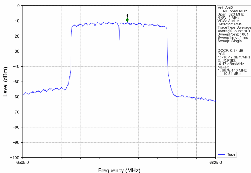
802.11ax(HEW160)_MCH_6665MHz_2xRU996_Left_MIMO_NTNV
