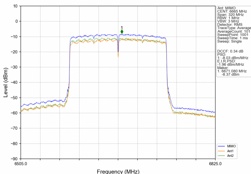
802.11ax(HEW160)_MCH_6665MHz_2xRU996_Left_MIMO_NTNV
