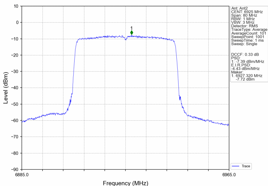
802.11ax(HEW40)_LCH_6925MHz_RU484_Left_MIMO_NTNV
