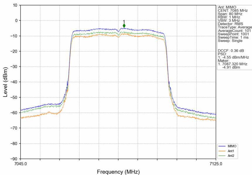
802.11ax(HEW40)_HCH_7085MHz_RU484_Left_MIMO_NTNV
