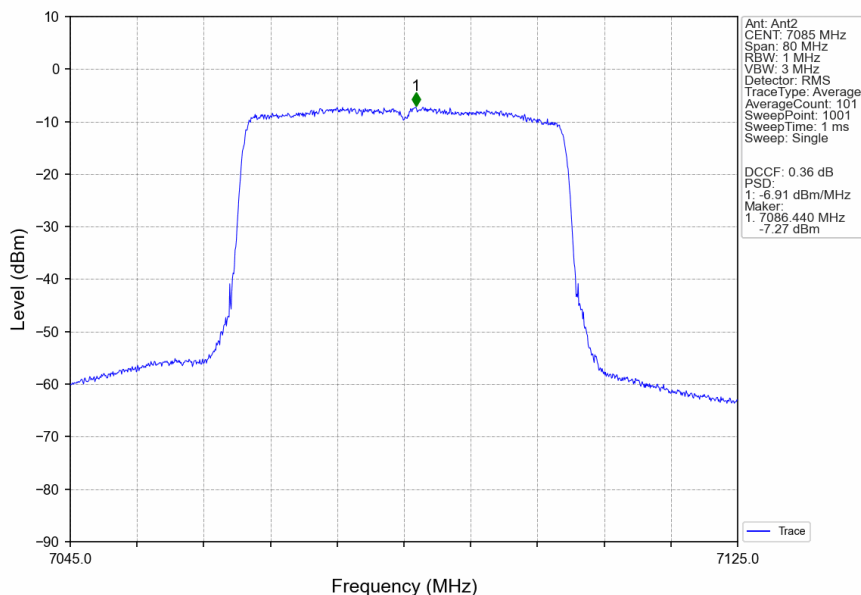
802.11ax(HEW40)_HCH_7085MHz_RU484_Left_MIMO_NTNV
