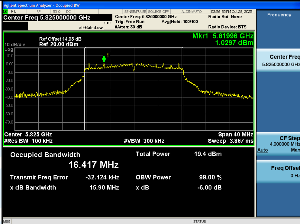
11A-Ant1-5825-PASS
