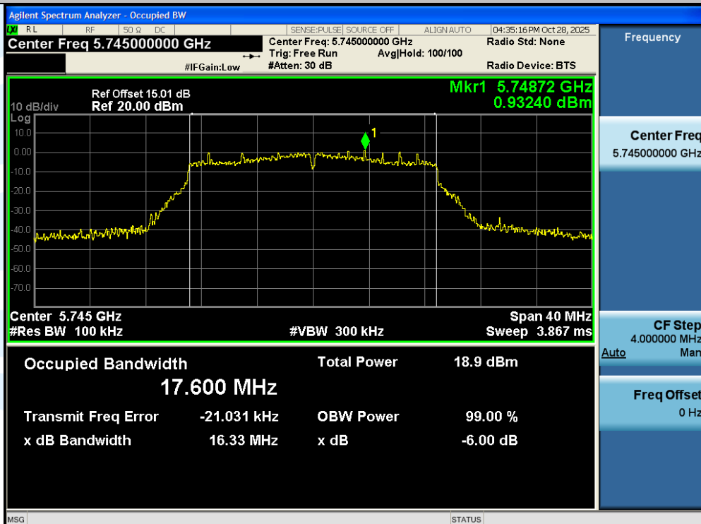
11N20SISO-Ant1-5745-PASS
