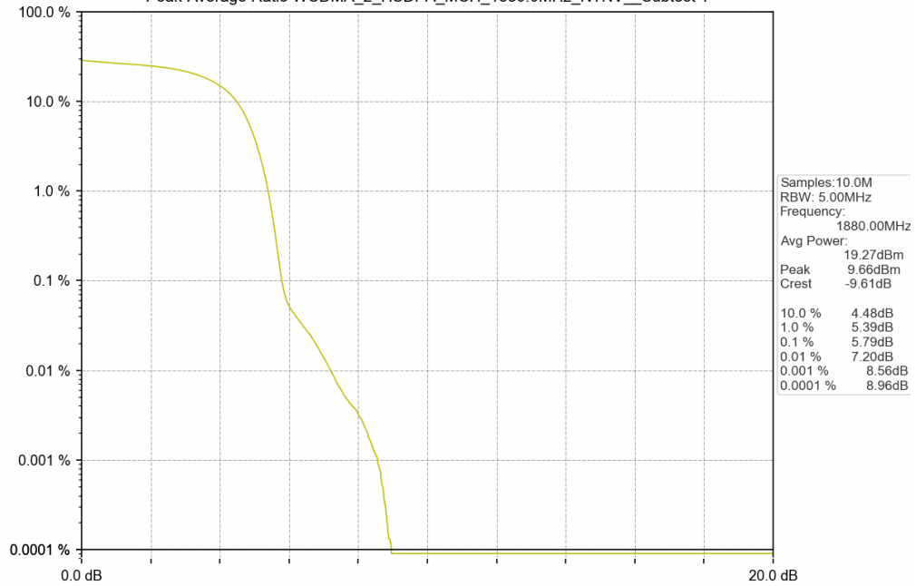
Peak-Average Ratio WCDMA_2_HSDPA_MCH_1880.0MHz_NTNV__Subtest 1
