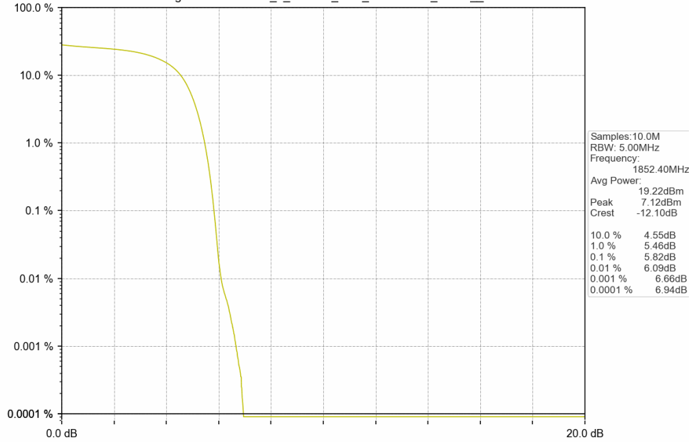
Peak-Average Ratio WCDMA_2_HSDPA_LCH_1852.4MHz_NTNV__Subtest 1
