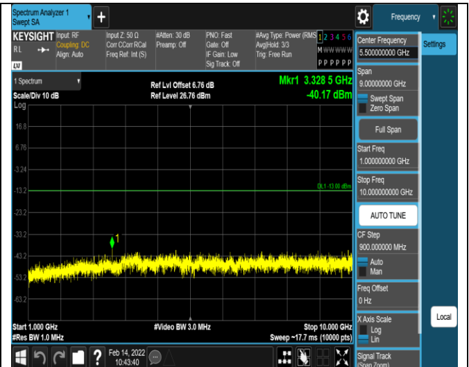
Band5-10MHz-16QAM-20600-1RB#0- Range2:1000~10000MHz
