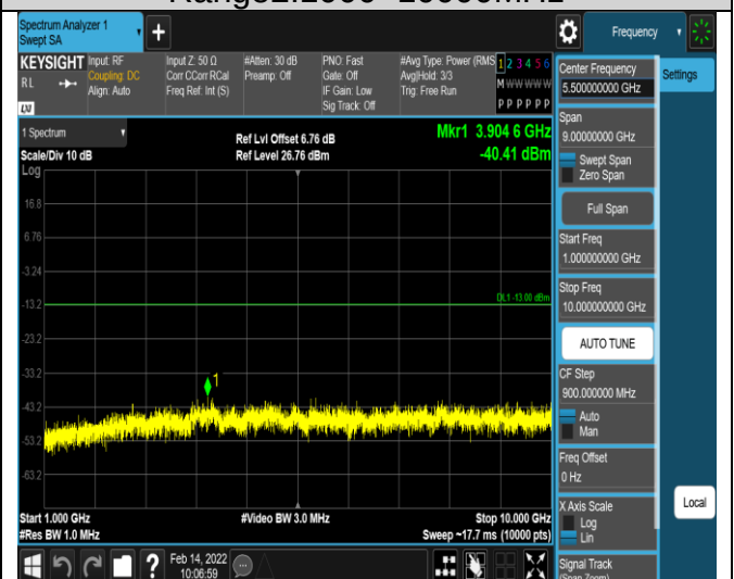
Band5-1.4MHz-16QAM-20525-1RB#0- Range2:1000~10000MHz
