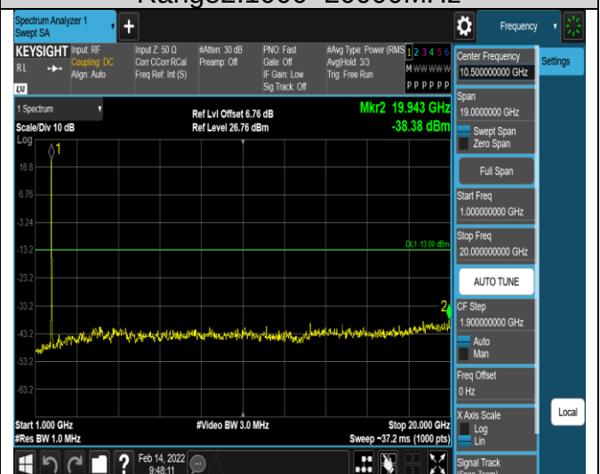
Band4-20MHz-16QAM-20050-1RB#0-
