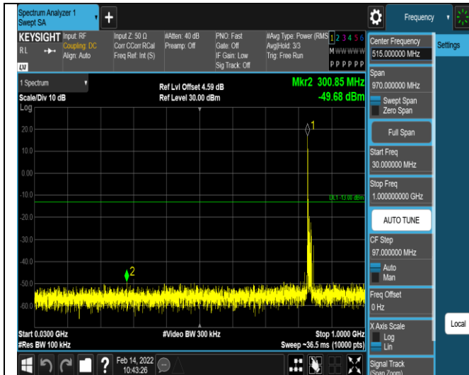
Band5-10MHz-16QAM-20600-1RB#0- Range1:30~1000MHz
