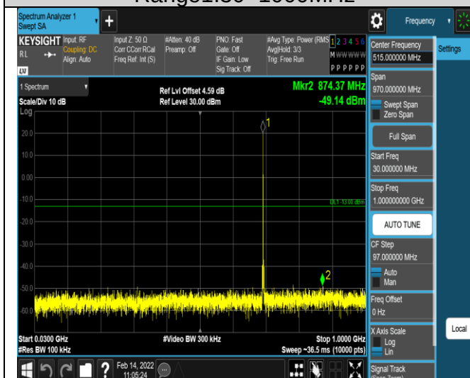
Band12-1.4MHz-QPSK-23095-1RB#0-
