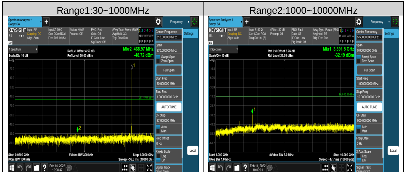
Band5-10MHz-QPSK-20450-1RB#0- Range1:30~1000MHz
