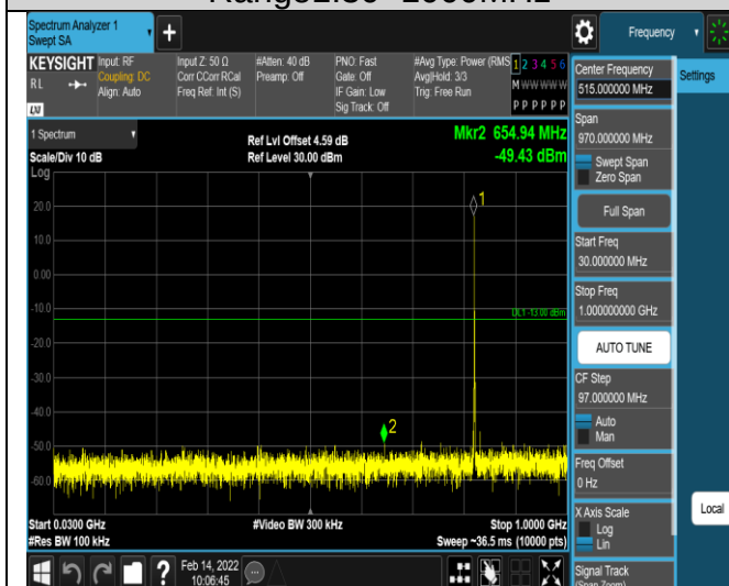
Band5-1.4MHz-16QAM-20525-1RB#0- Range1:30~1000MHz
