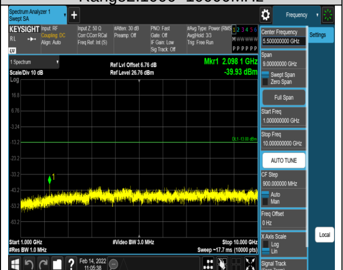
Band12-1.4MHz-QPSK-23095-1RB#0-
