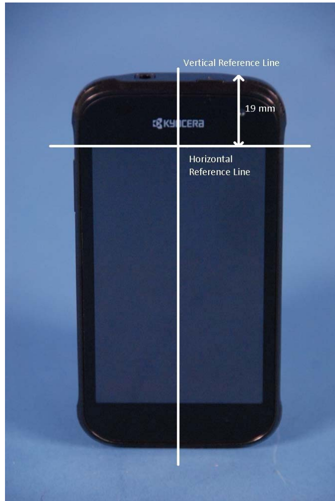
SAR Test Setup Photo 11: Vertical and Horizontal Reference Lines
