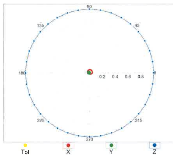
f=1800 MHz,R22,90°
