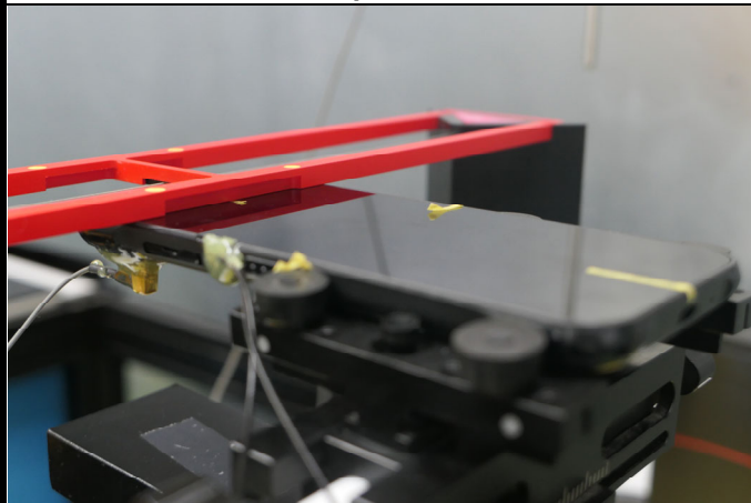
Left View
