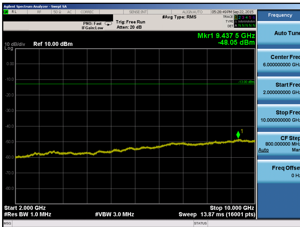
Plot 6-5. Conducted Spurious Plot (Cellular CDMA Mode – Ch. 1013)
