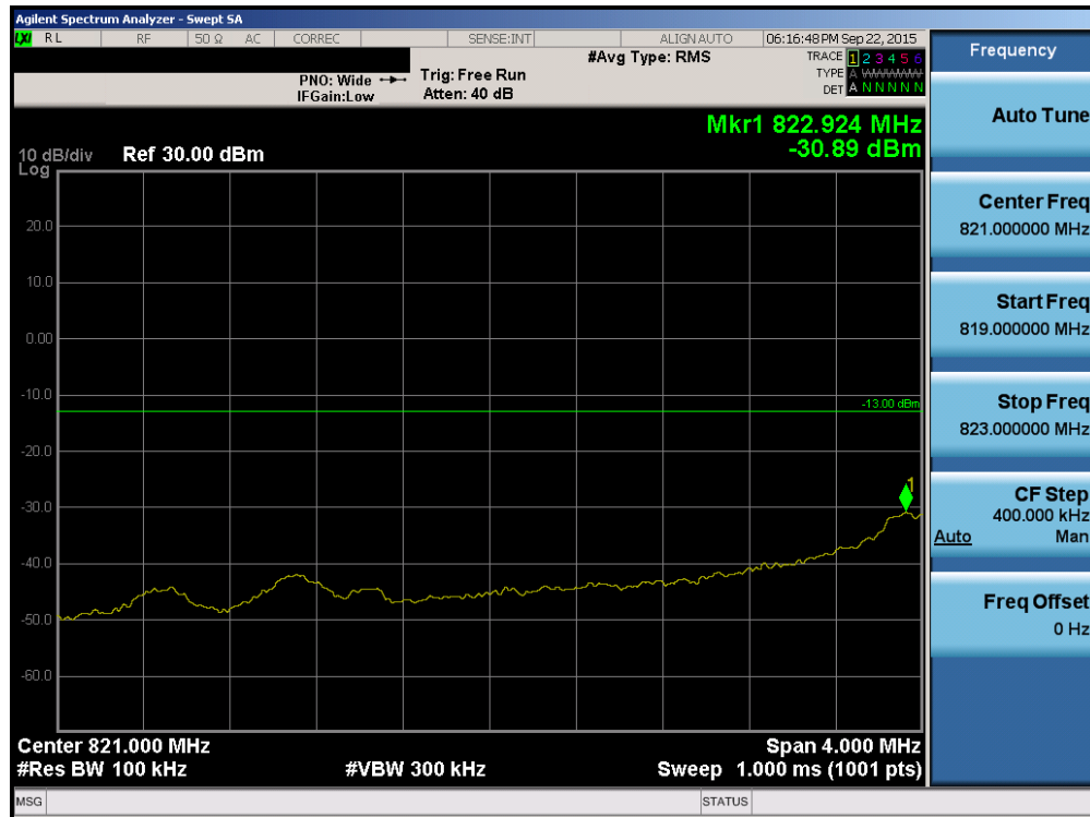
Plot 6-22. 4MHz Span Plot (Cellular CDMA Mode – Ch. 1013)
