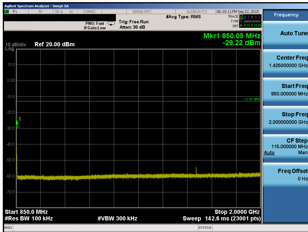
Plot 6-10. Conducted Spurious Plot (Cellular CDMA Mode – Ch. 777)
