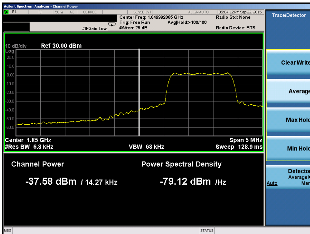
Plot 6-25. Band Edge Plot (PCS CDMA Mode – Ch. 25)
