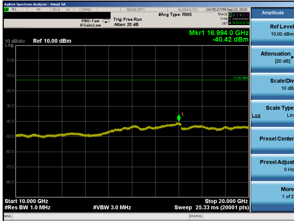
Plot 6-17. Conducted Spurious Plot (PCS CDMA Mode – Ch. 600)
