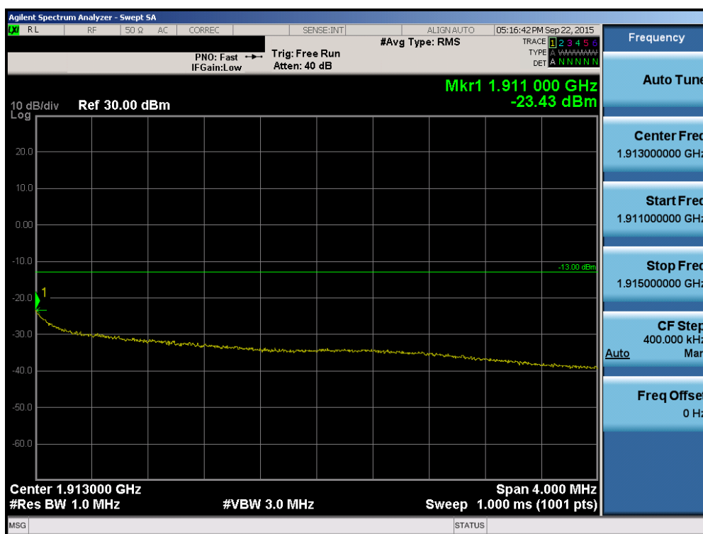
Plot 6-28. 4MHz Span Plot (PCS CDMA Mode – Ch. 1175)
