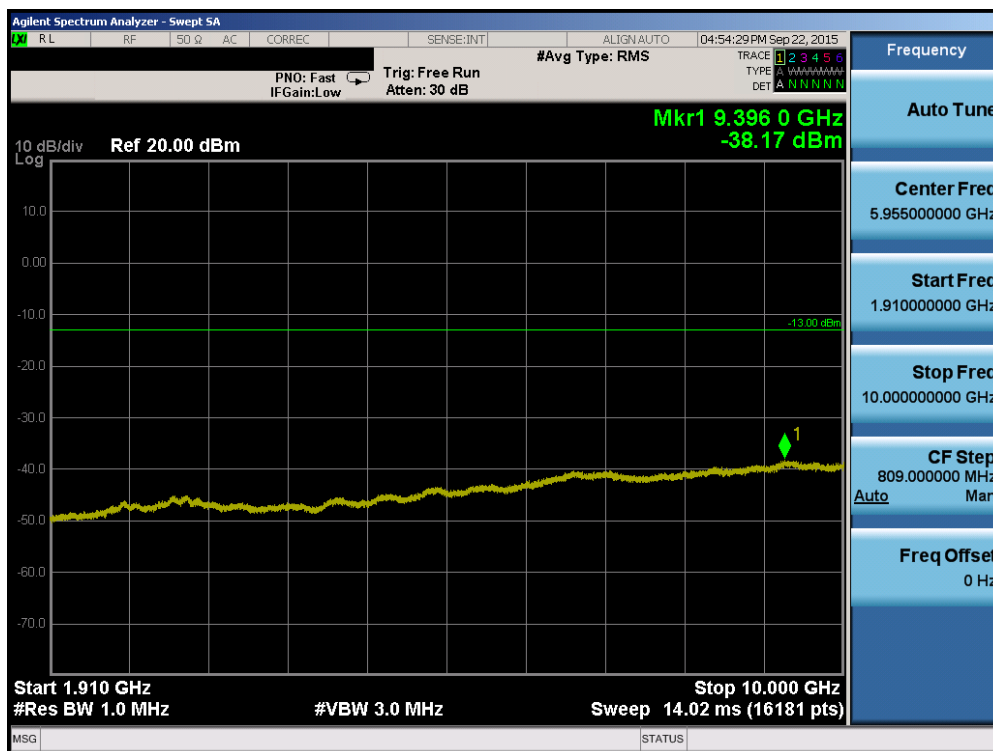
Plot 6-16. Conducted Spurious Plot (PCS CDMA Mode – Ch. 600)
