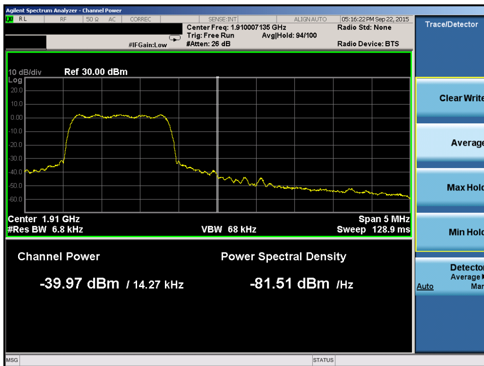
Plot 6-27. Band Edge Plot (PCS CDMA Mode – Ch. 1175)
