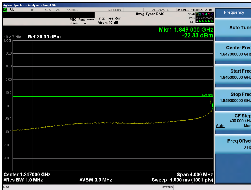
Plot 6-26. 4MHz Span Plot (PCS CDMA Mode – Ch. 25)
