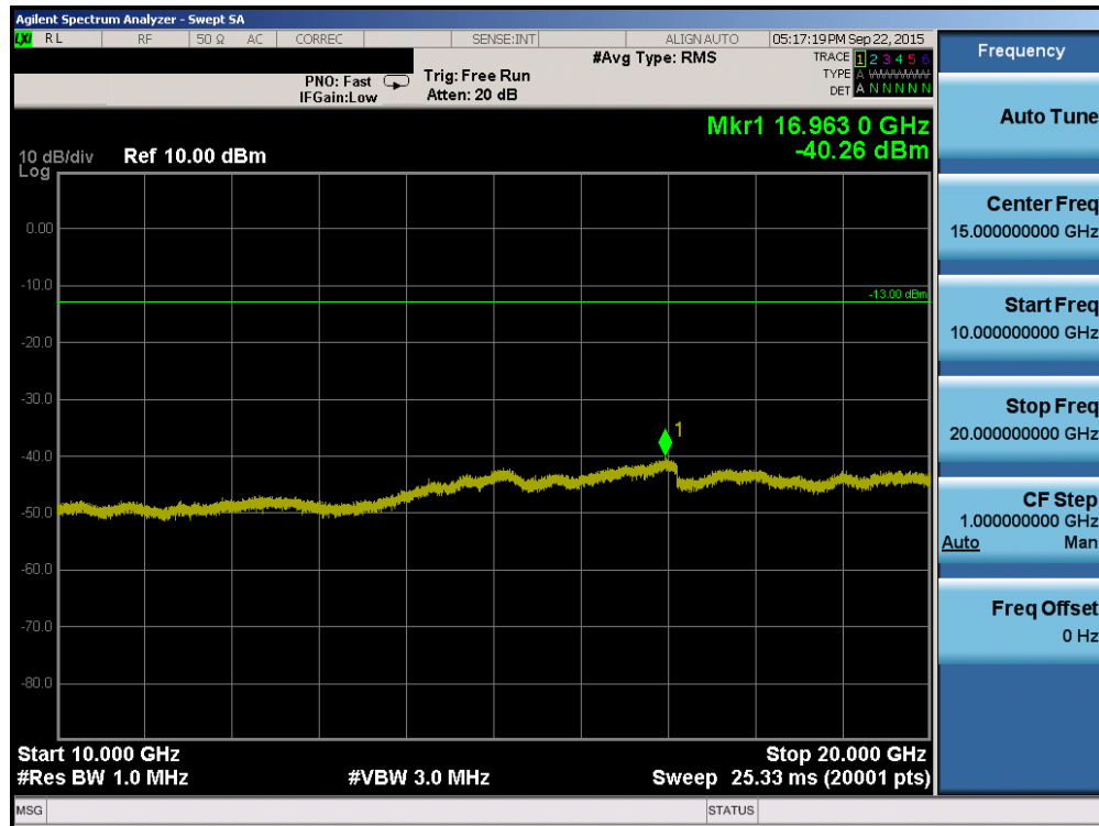
Plot 6-20. Conducted Spurious Plot (PCS CDMA Mode – Ch. 1175)
