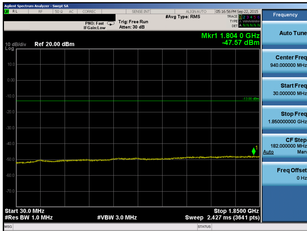
Plot 6-18. Conducted Spurious Plot (PCS CDMA Mode – Ch. 1175)
