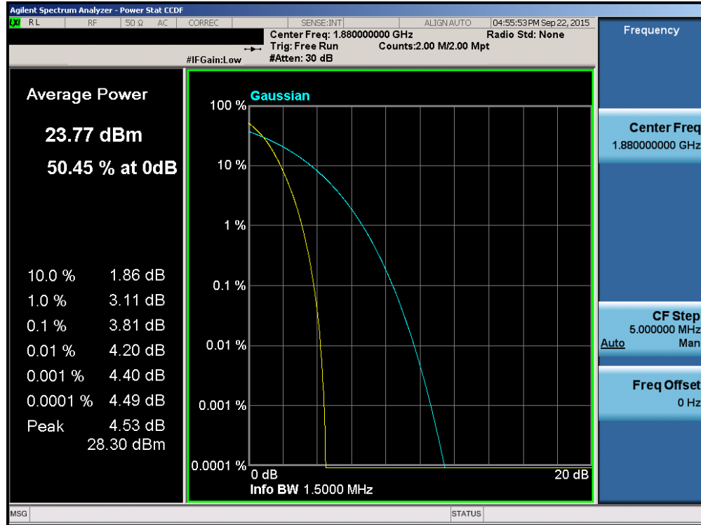
Plot 6-29. Peak-Average Ratio Plot (PCS CDMA Mode – Ch. 600)
