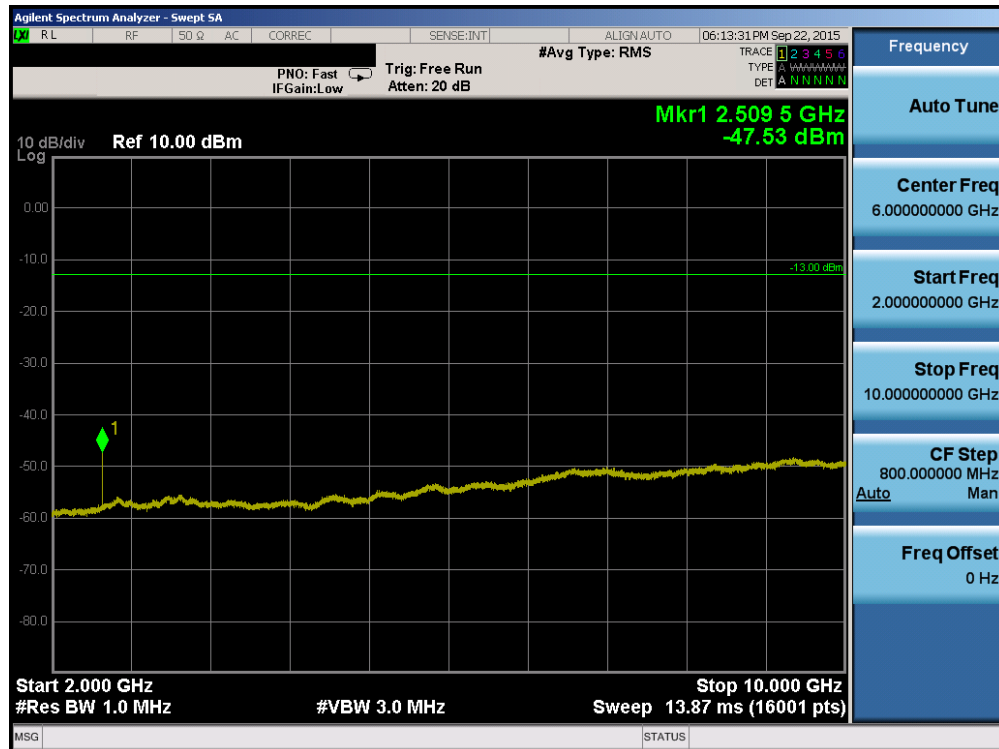
Plot 6-8. Conducted Spurious Plot (Cellular CDMA Mode – Ch. 384)
