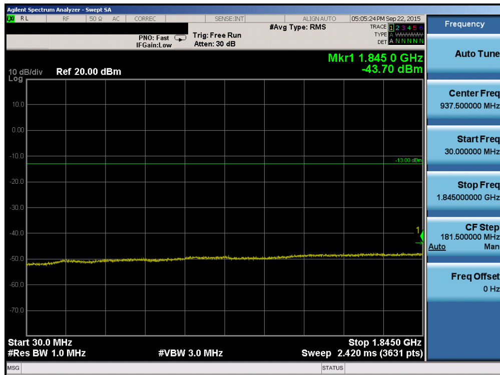
Plot 6-12. Conducted Spurious Plot (PCS CDMA Mode – Ch. 25)
