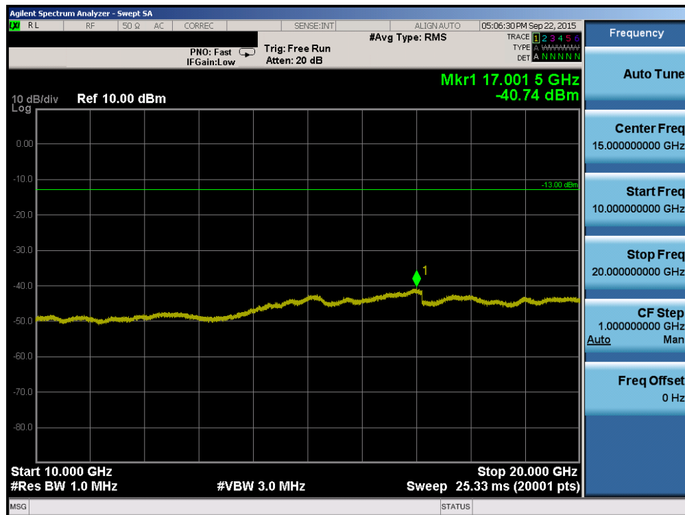
Plot 6-14. Conducted Spurious Plot (PCS CDMA Mode – Ch. 25)
