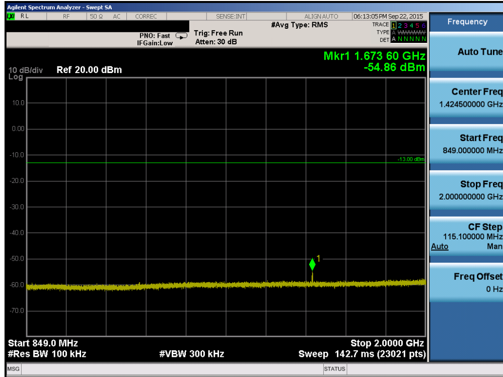
Plot 6-7. Conducted Spurious Plot (Cellular CDMA Mode – Ch. 384)
