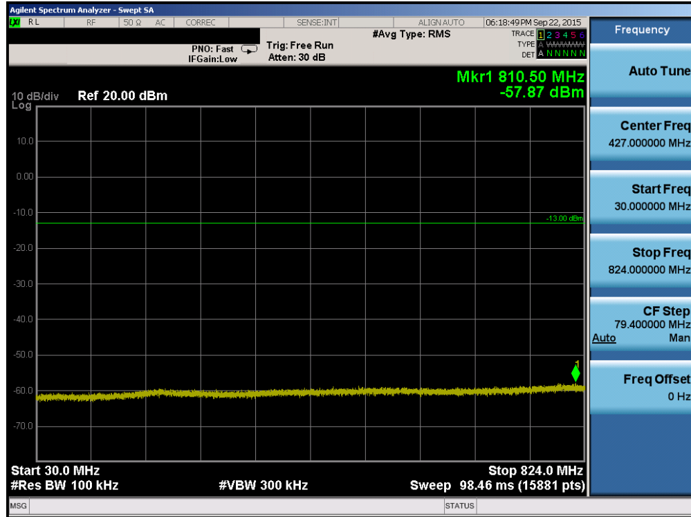
Plot 6-9. Conducted Spurious Plot (Cellular CDMA Mode – Ch. 777)
