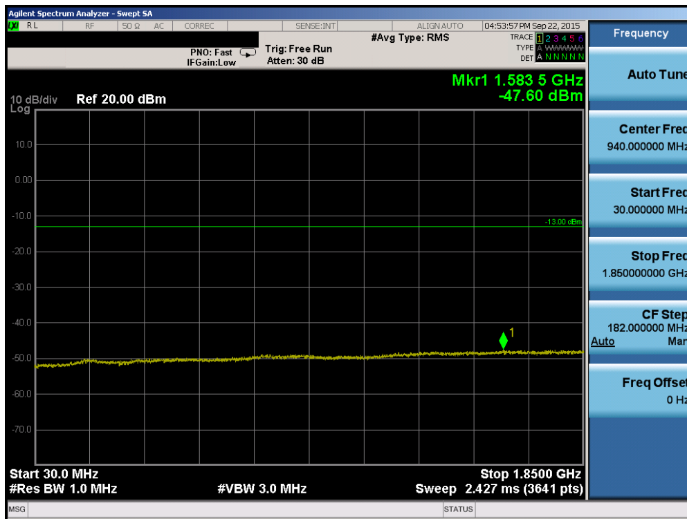
Plot 6-15. Conducted Spurious Plot (PCS CDMA Mode – Ch. 600)
