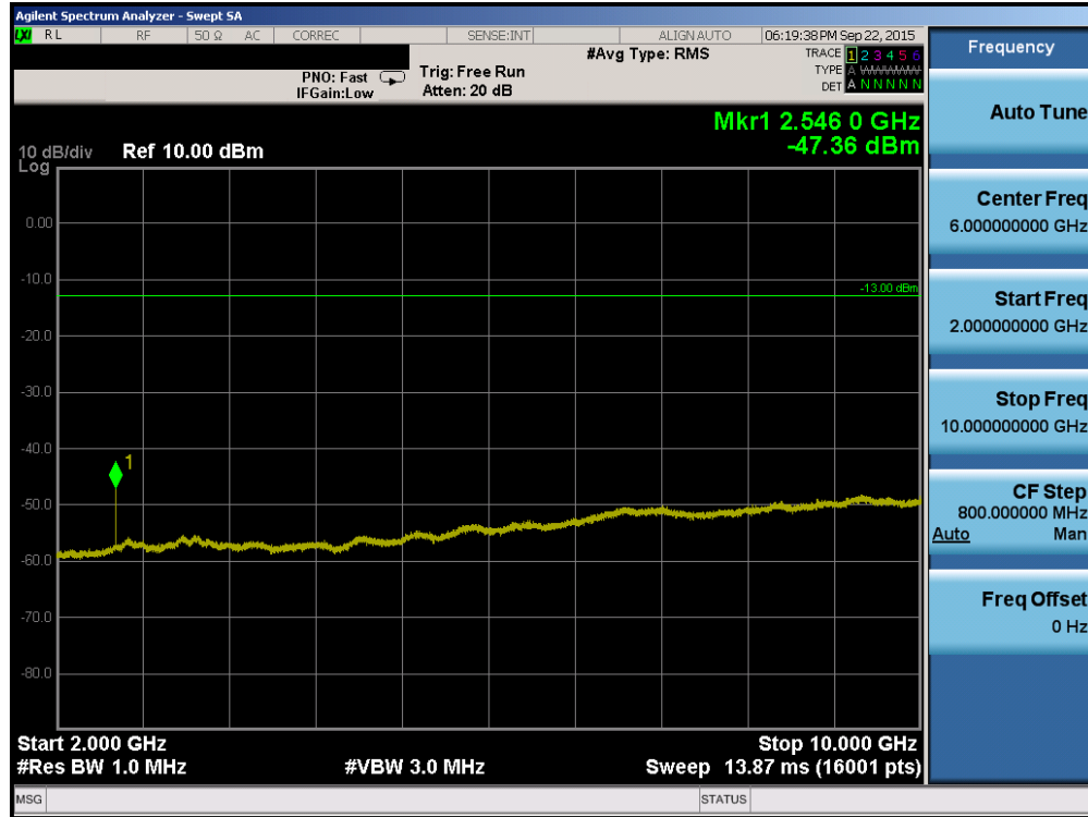
Plot 6-11. Conducted Spurious Plot (Cellular CDMA Mode – Ch. 777)
