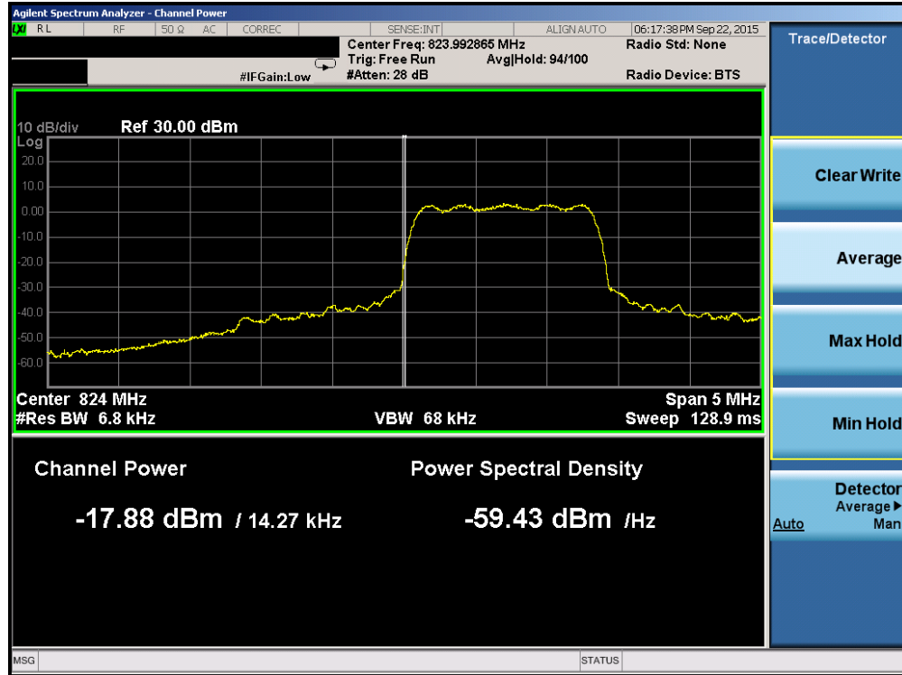
Plot 6-21. Band Edge Plot (Cellular CDMA Mode – Ch. 1013)
