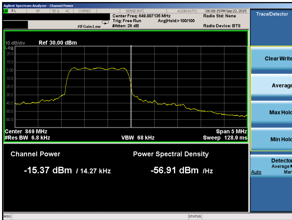
Plot 6-23. Band Edge Plot (Cellular CDMA Mode – Ch. 777)
