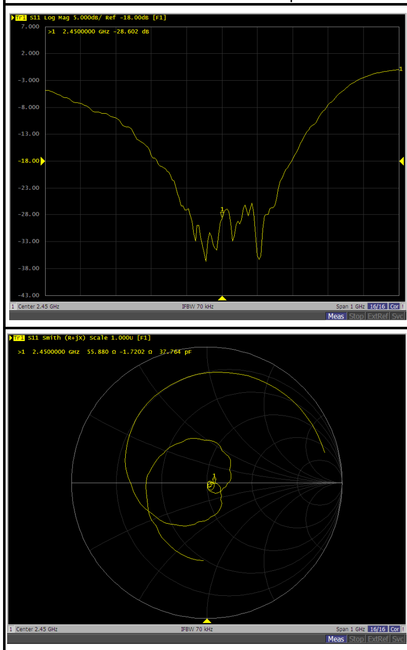
2450 MHz , Free Space
