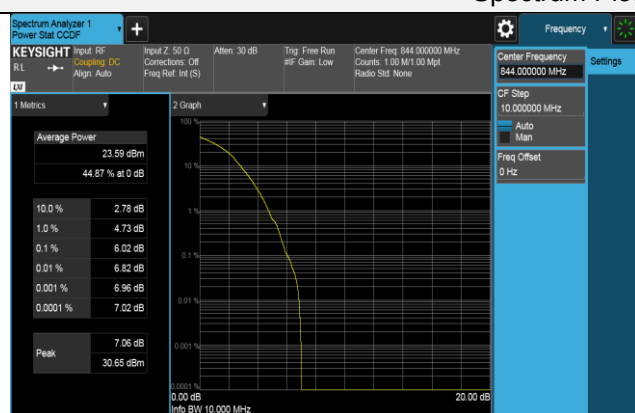
16QAM CH 20600 (844MHz)
