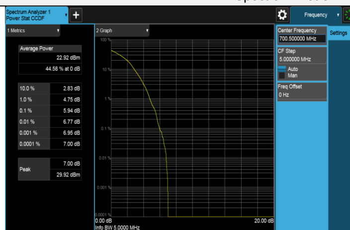
16QAM CH 23025 (700.5MHz)
