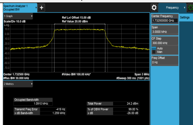
Occupied bandwidth
