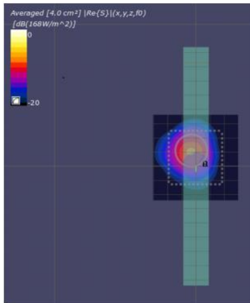
(a) Measurement
