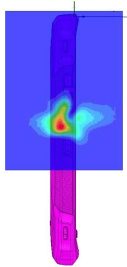
(b) Simulation
