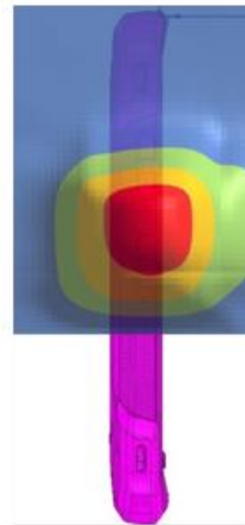
(b) Simulation
