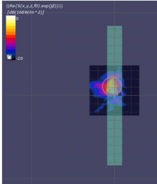
(a) Measurement
