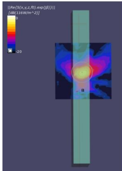
(a) Measurement
