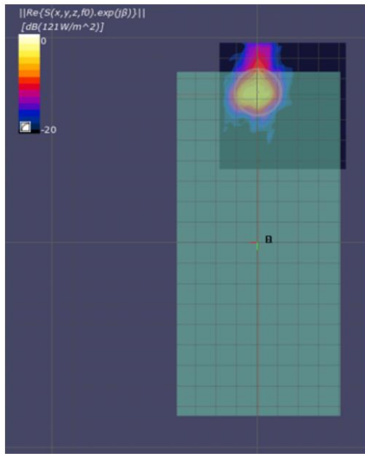
(a) Measurement
