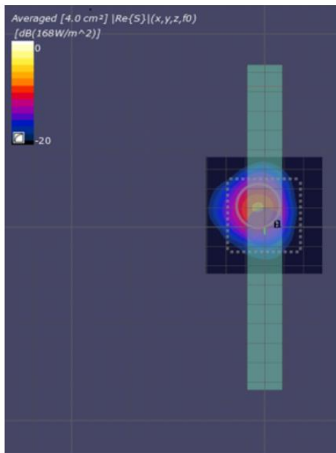
(a)Measurement
