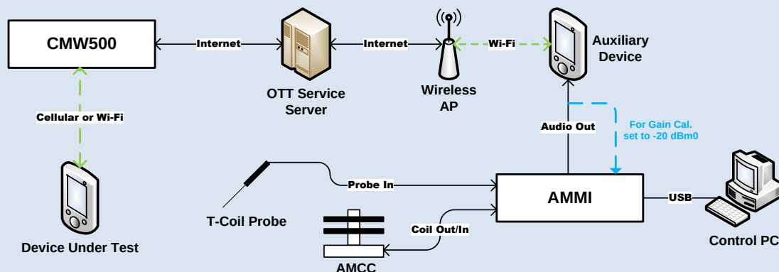
Fig-3.10 Testing Setup for OTT Calling
