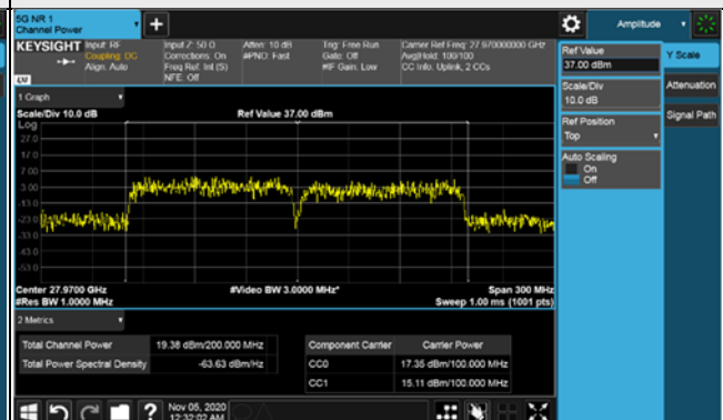
2CC / QPSK / Mid Channel
