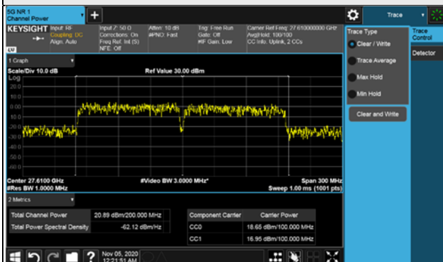
2CC / QPSK / High Channel
