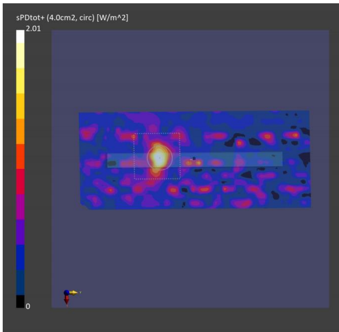
Figure 8-2: 4cm 2 -averaged power density distribution measured at input.power.limit of -0.9 dBm on the Left Side surface for n258 beam 31
