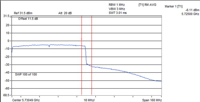
802.11ax (HE80) Full RU / Chain 0 : CH 138 (U-NII-3)
