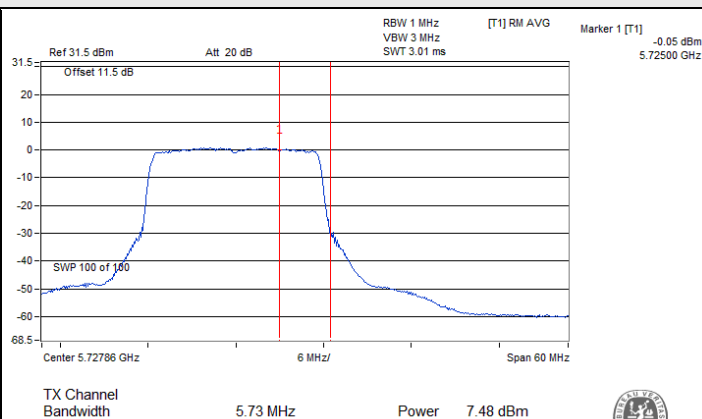
802.11ax (HE20) Full RU / Chain 0 : CH 144 (U-NII-3)
