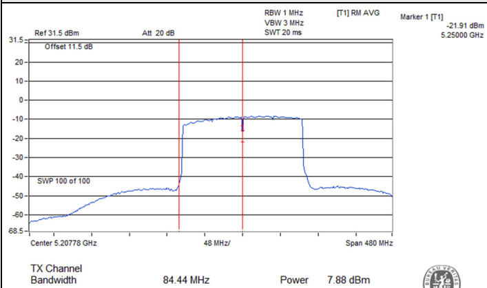
802.11ax (HE160) Full RU / Chain 0 : CH 50 (U-NII-1)
