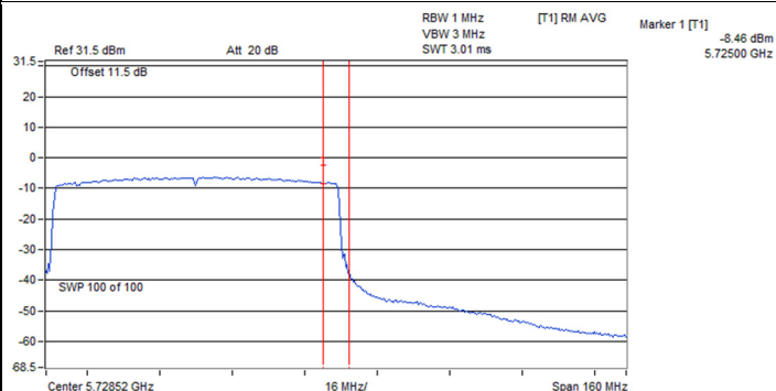
802.11ax (HE40) Full RU / Chain 1 : CH 142 (U-NII-3)
