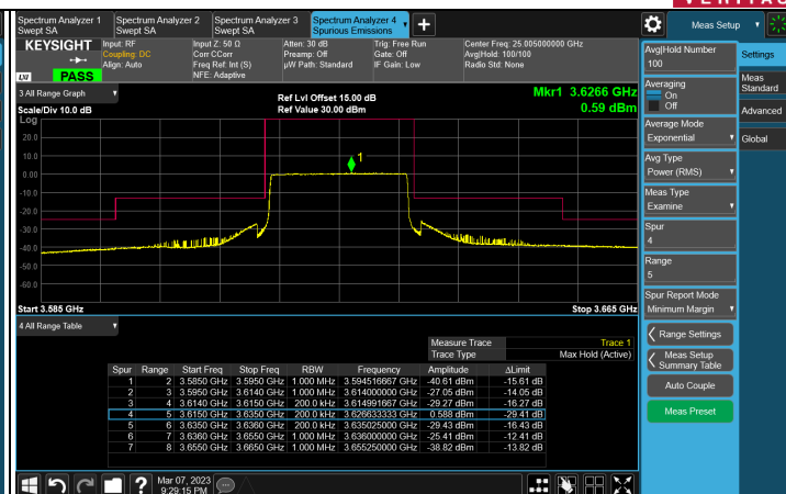
FULL CH 641666 (3624.99 MHz)
