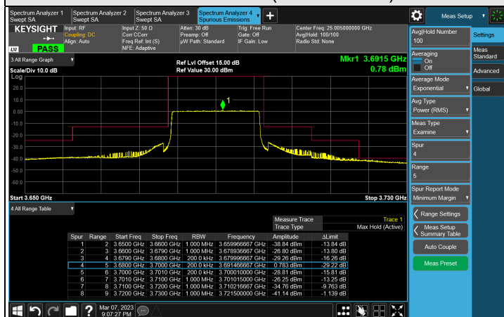
FULL CH 646000 (3690 MHz)
