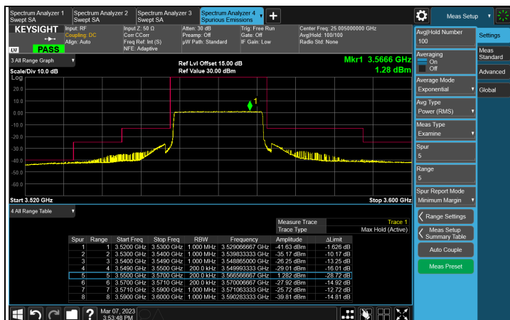
FULL CH 637334 (3560.01 MHz)
