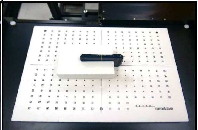
Left Side of EUT Tested at 2 mm
