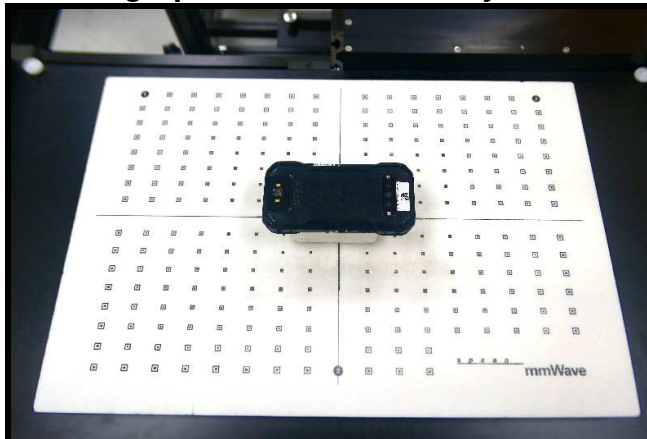
Rear Face of EUT Tested at 2 mm
