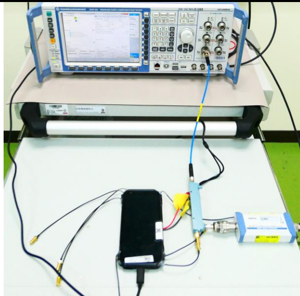
Setup for Conducted Power Test (Figure 4-1)
