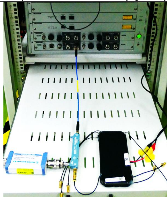
Setup for Conducted Power Test (Figure 4-1)
