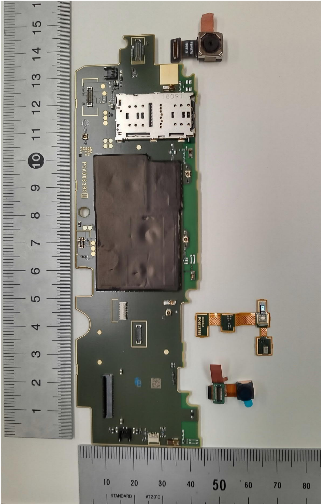
Main PCB Front
