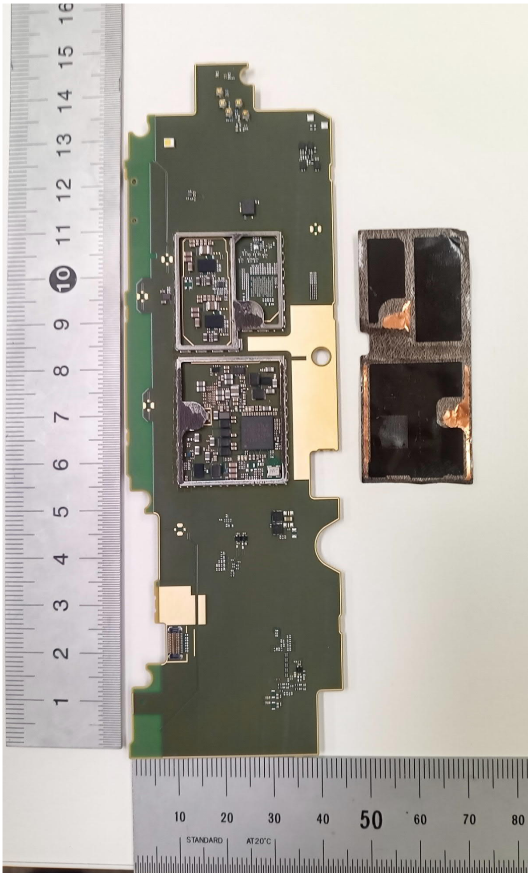
Main PCB Rear Open
