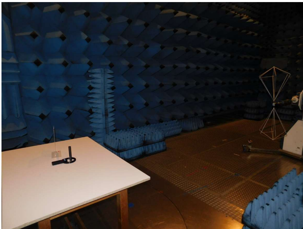
Pre-test setup
