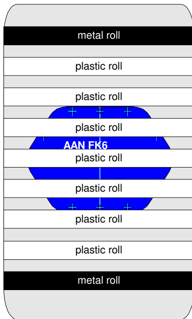
figure 5.4.1 orientation 0°
