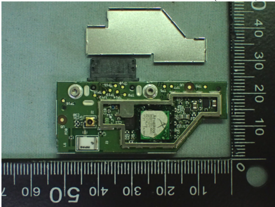
Figure 11 Internal View (Main Board, Front View)
