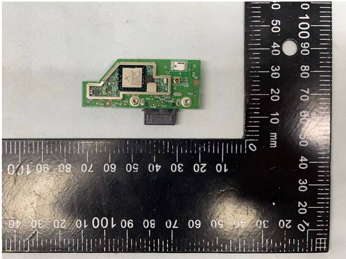
Figure 3 PCB Board (Cover Removed, Component Side)
