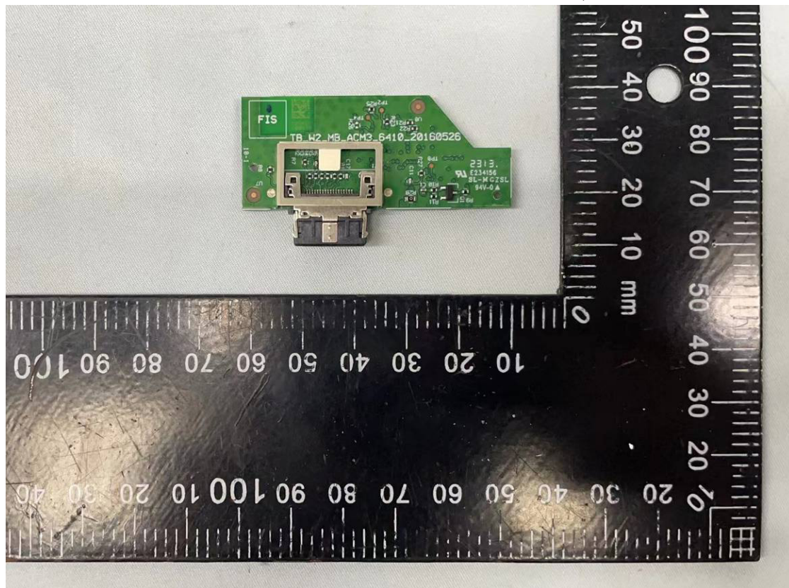
Figure 4 PCB Board (Cover Removed, Solder Side)
