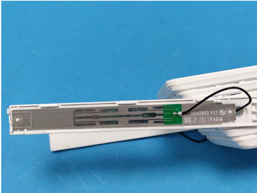
Antenna Chain 1
