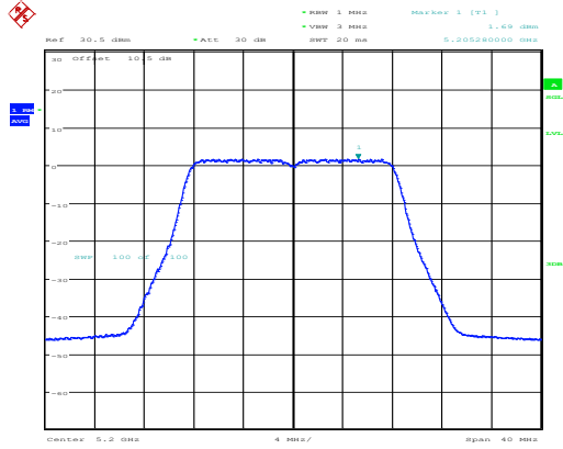
802.11a_5200MHz_Chain 1
