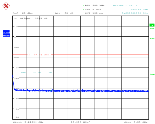
802.11ax20_5200MHz_RU_Full_Chain 1
