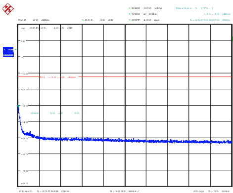
802.11a_5240MHz_Chain 1
