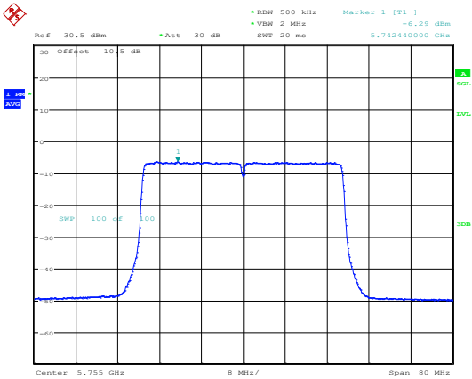
802.11ax40_5755MHz_RU_Full_Chain 1
