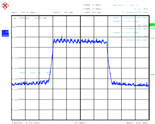
802.11ax80_5290MHz_RU_Full_Chain 0
