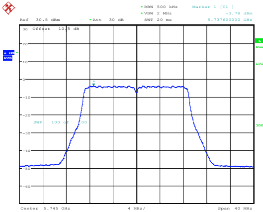
802.11ac20_5745MHz_Chain 1
