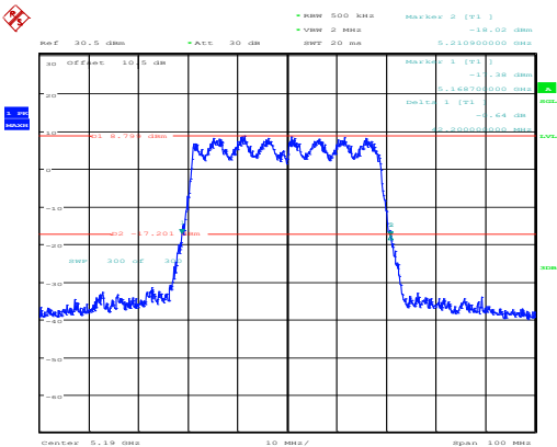
802.11ax40_5190MHz_RU_Full_Chain 0
