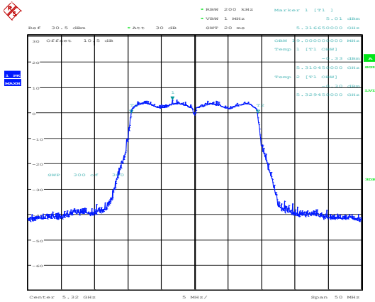
802.11ax20_5320MHz_RU_Full_Chain 0
