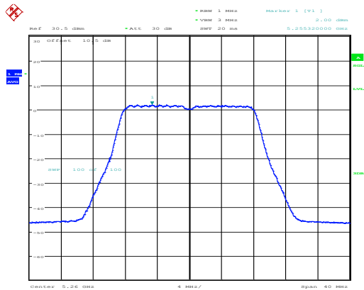
802.11a_5260MHz_Chain 0
