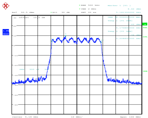
802.11ax40_5190MHz_RU_Full_Chain 0
