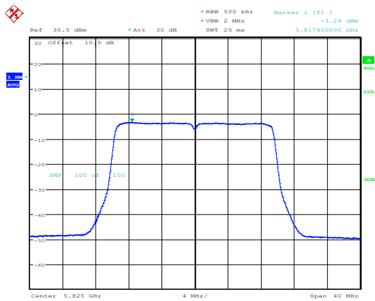
802.11ax20_5825MHz_RU_Full_Chain 1
