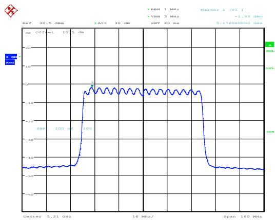
802.11ax80_5210MHz_RU_Full_Chain 0
