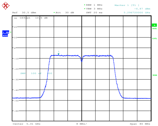
802.11ac40_5310MHz_Chain 1
