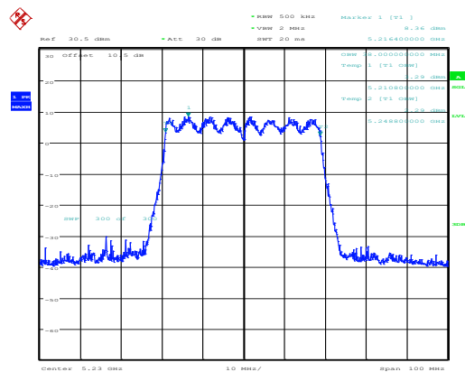
802.11ax40_5230MHz_RU_Full_Chain 0
