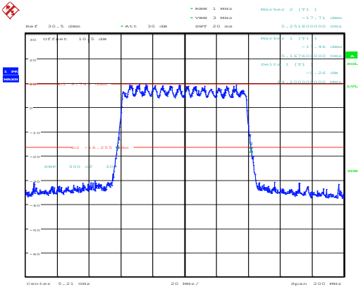
802.11ax80_5210MHz_RU_Full_Chain 0
