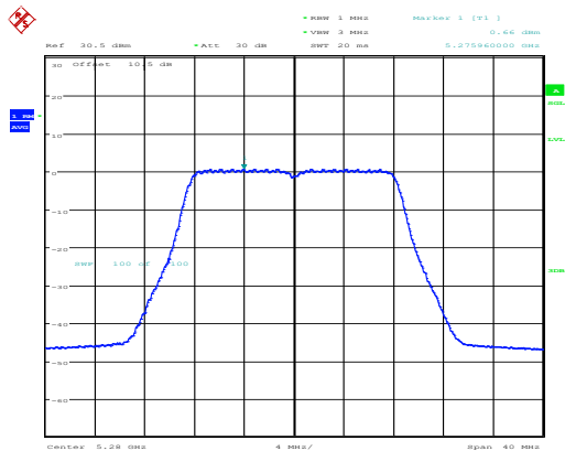
802.11a_5280MHz_Chain 1
