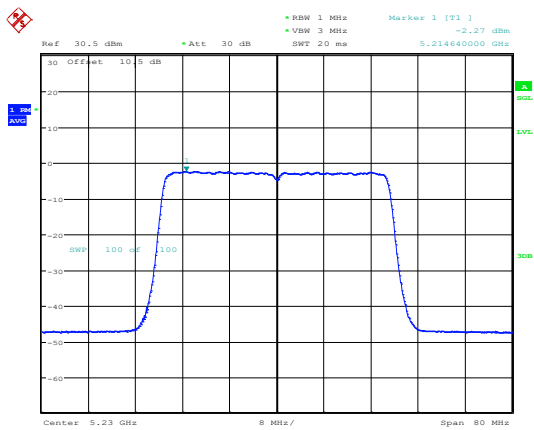
802.11ax40_5230MHz_RU_Full_Chain 0
