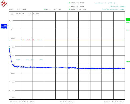
802.11ax80_5210MHz_RU_Full_Chain 1
