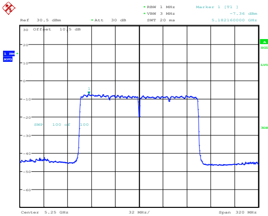
802.11ac160_5250MHz_Chain 1
