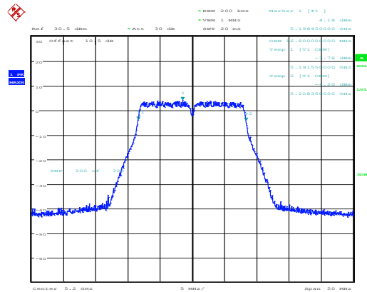
802.11a_5200MHz_Chain 0
