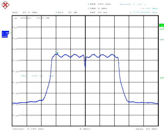
802.11ac40_5795MHz_Chain 0
