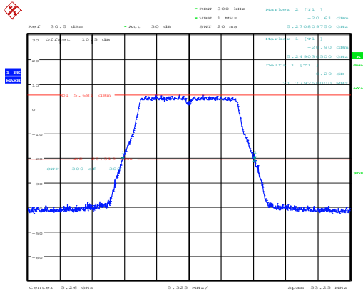
802.11a_5260MHz_Chain 0
