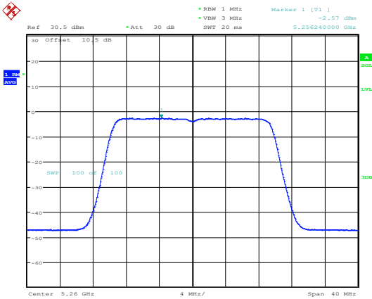
802.11ax20_5260MHz_RU_Full_Chain 0
