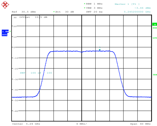
802.11ax20_5240MHz_RU_Full_Chain 1
