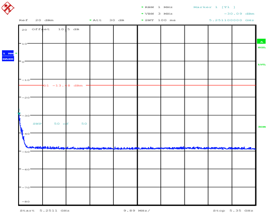
802.11ax40_5230MHz_RU_Full_Chain 0
