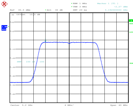
802.11ax20_5200MHz_RU_Full_Chain 0
