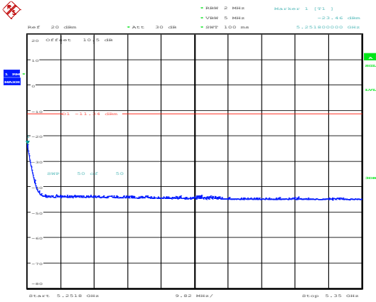
802.11ax80_5210MHz_RU_Full_Chain 0
