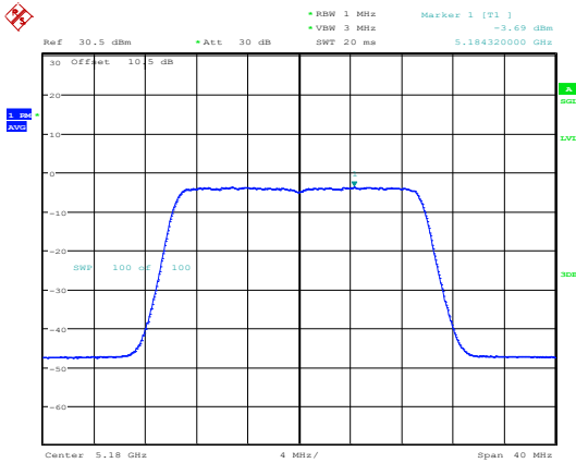
802.11ax20_5180MHz_RU_Full_Chain 1
