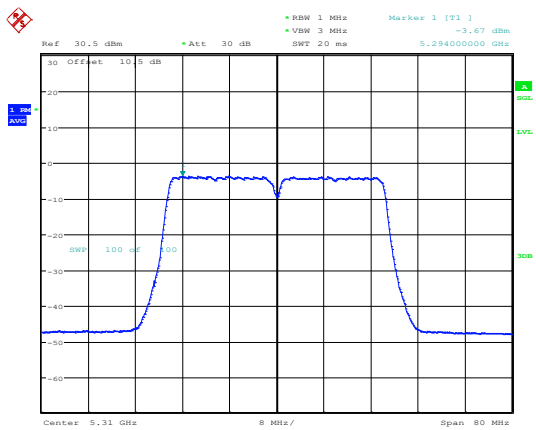
802.11ac40_5310MHz_Chain 0
