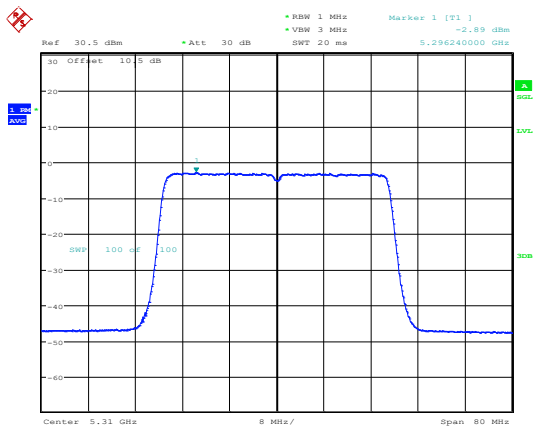
802.11ax40_5310MHz_RU_Full_Chain 0
