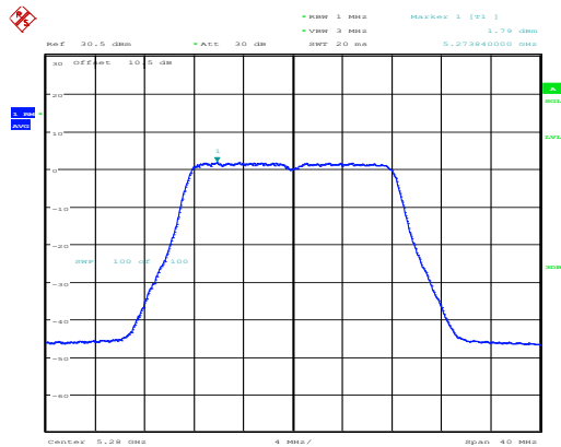
802.11a_5280MHz_Chain 0
