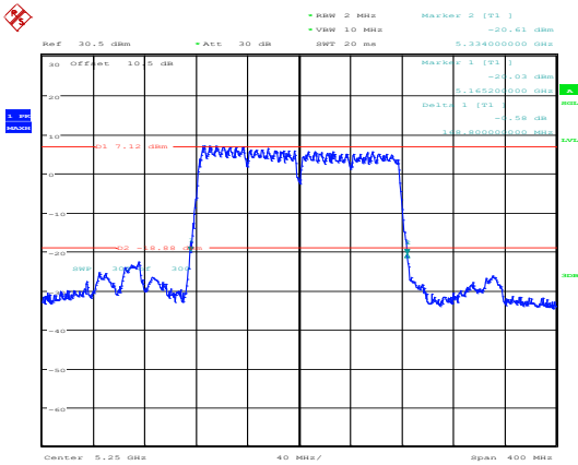
802.11ac160_5250MHz_Chain 0
