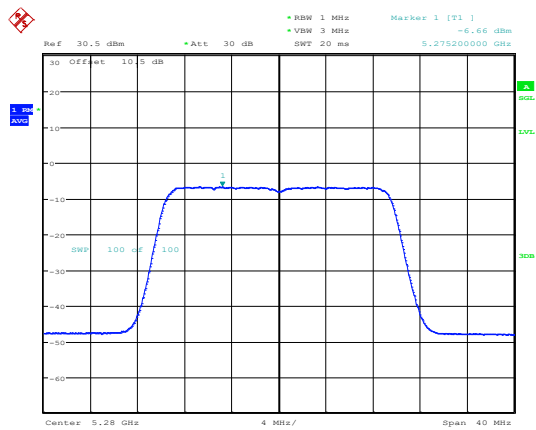
802.11ax20_5280MHz_RU_Full_Chain 1
