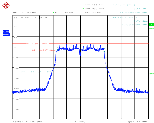
802.11ac20_5745MHz_Chain 0
