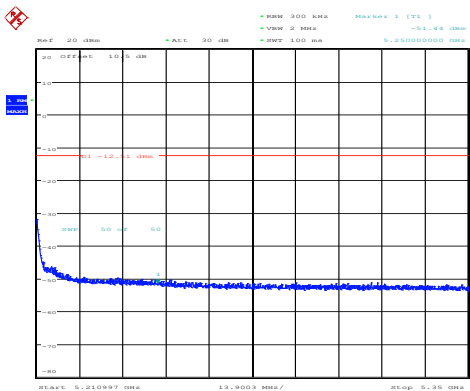
802.11a_5200MHz_Chain 1
