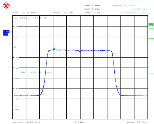
802.11ax40_5190MHz_RU_Full_Chain 0
