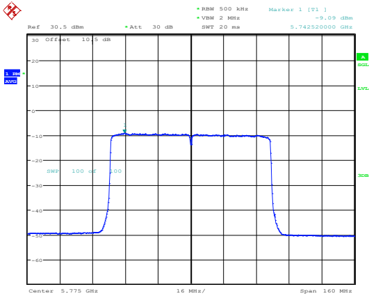
802.11ax80_5775MHz_RU_Full_Chain 1
