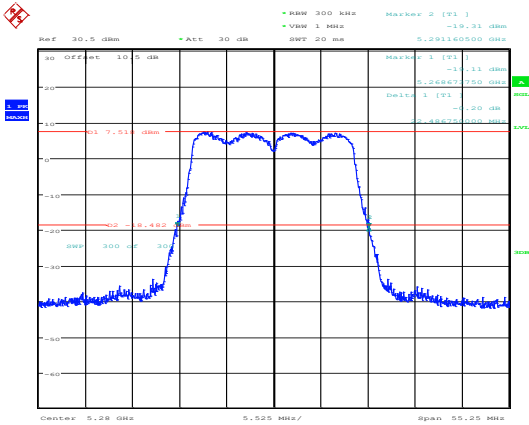
802.11ax20_5280MHz_RU_Full_Chain 0
