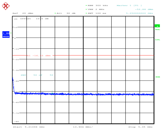
802.11ax20_5200MHz_RU_Full_Chain 0
