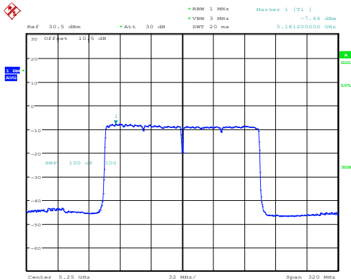
802.11ax160_5250MHz_RU_Full_Chain 1
