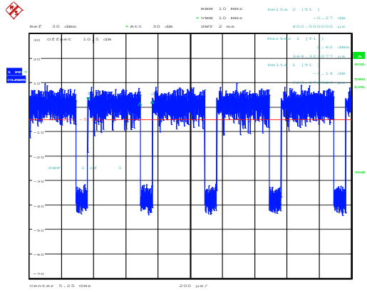
802.11ax160_5250MHz_RU_Full_Chain 0
