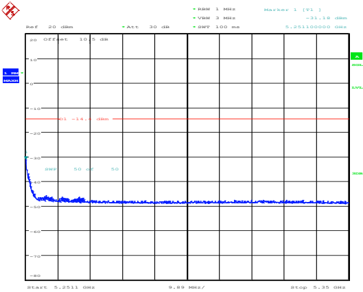
802.11ax40_5230MHz_RU_Full_Chain 1
