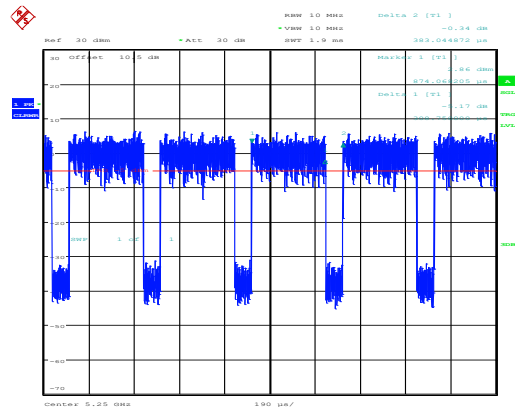
802.11ac160_5250MHz_Chain 0
