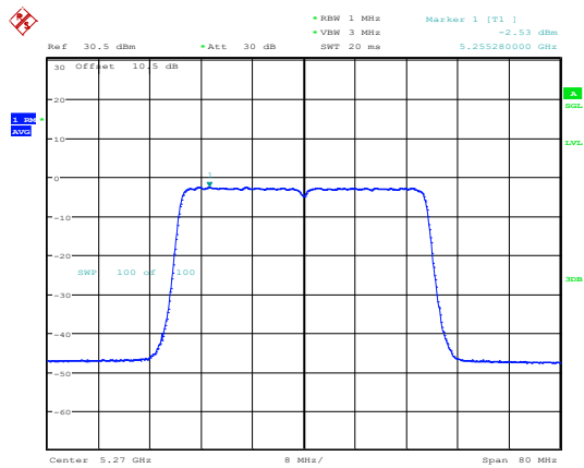
802.11ax40_5270MHz_RU_Full_Chain 0
