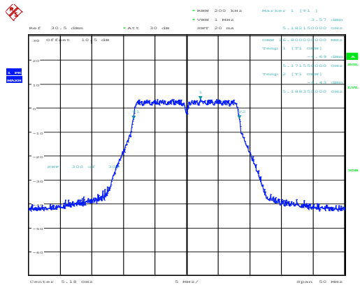
802.11a_5180MHz_Chain 0
