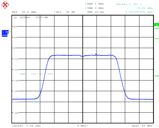
802.11ax20_5260MHz_RU_Full_Chain 1
