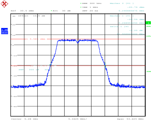
802.11a_5280MHz_Chain 0
