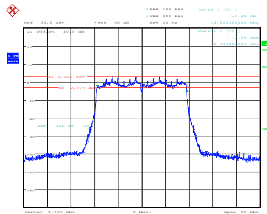
802.11ax20_5745MHz_RU_Full_Chain 0
