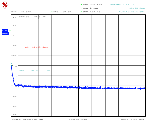
802.11a_5240MHz_Chain 0
