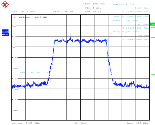
802.11ax40_5310MHz_RU_Full_Chain 0
