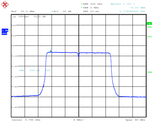
802.11ax40_5795MHz_RU_Full_Chain 1
