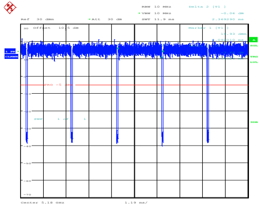
802.11ax20_5180MHz_RU_Full_Chain 0
