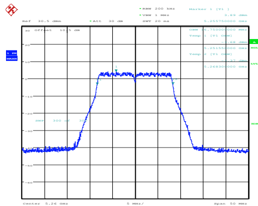
802.11a_5260MHz_Chain 0
