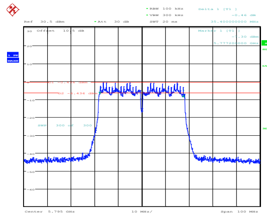
802.11ac40_5795MHz_Chain 0
