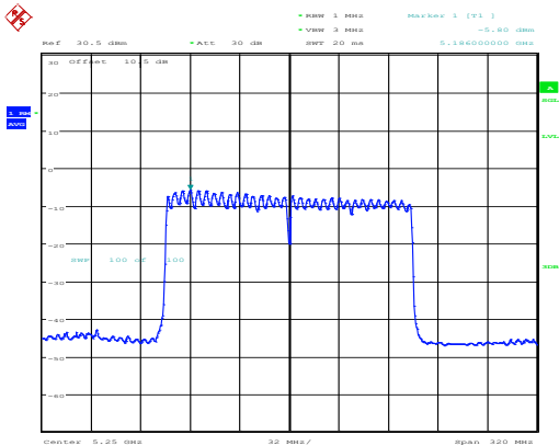
802.11ax160_5250MHz_RU_Full_Chain 0
