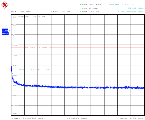
802.11a_5180MHz_Chain 1
