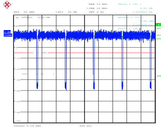
802.11ax40_5190MHz_RU_Full_Chain 0
