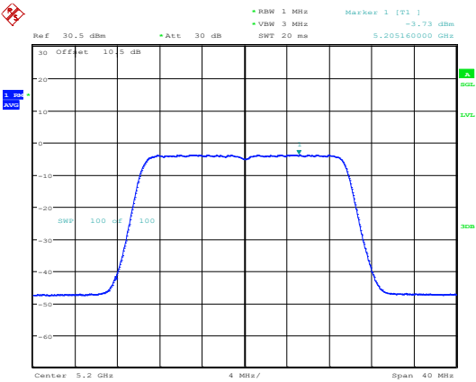
802.11ax20_5200MHz_RU_Full_Chain 1
