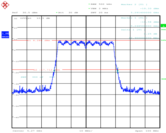
802.11ax40_5270MHz_RU_Full_Chain 0
