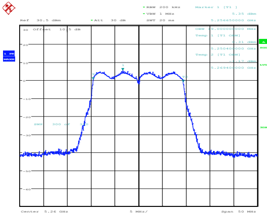
802.11ax20_5260MHz_RU_Full_Chain 0
