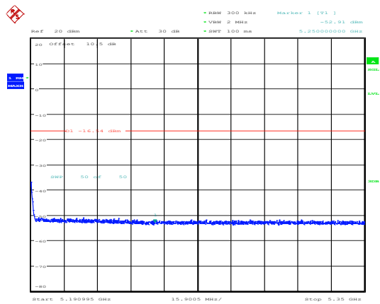
802.11ax20_5180MHz_RU_Full_Chain 0
