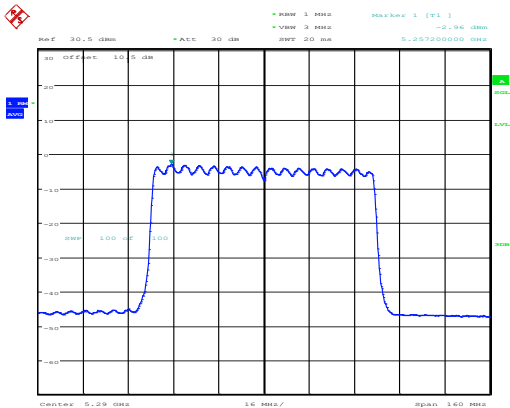
802.11ax80_5290MHz_RU_Full_Chain 0
