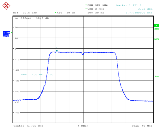
802.11ax20_5785MHz_RU_Full_Chain 1
