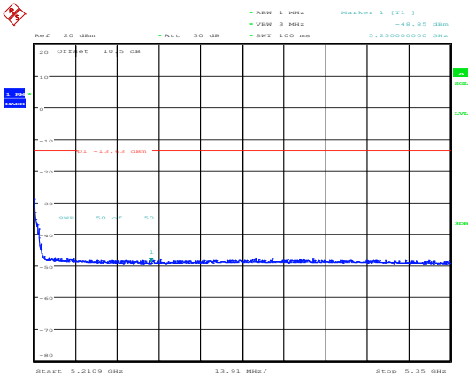
802.11ax40_5190MHz_RU_Full_Chain 0
