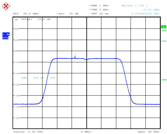
802.11ax20_5320MHz_RU_Full_Chain 1
