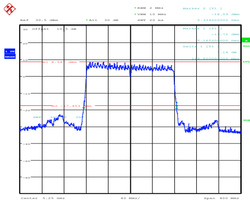
802.11ax160_5250MHz_RU_Full_Chain 0
