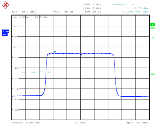
802.11ax80_5290MHz_RU_Full_Chain 1
