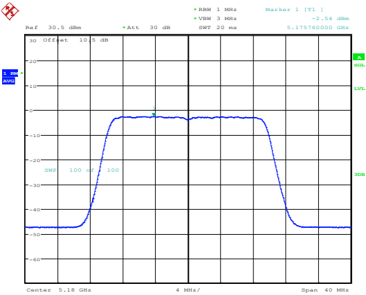
802.11ax20_5180MHz_RU_Full_Chain 0
