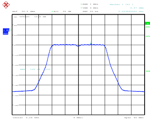
802.11a_5260MHz_Chain 1
