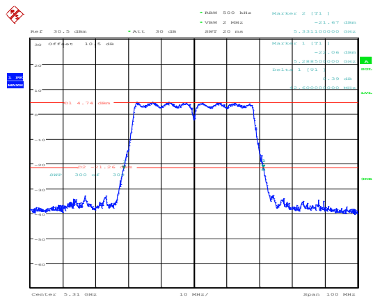
802.11ac40_5310MHz_Chain 0
