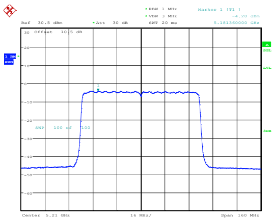
802.11ax80_5210MHz_RU_Full_Chain 1
