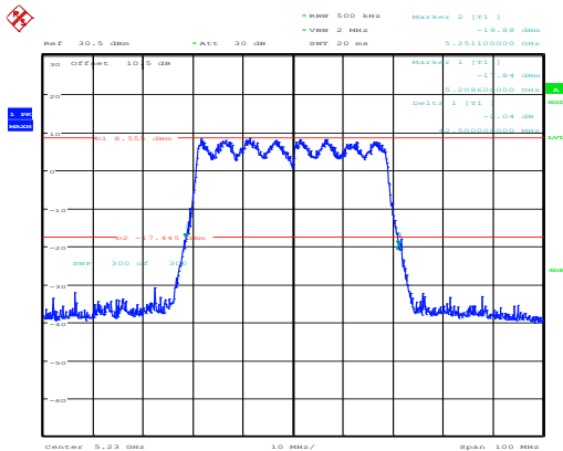
802.11ax40_5230MHz_RU_Full_Chain 0
