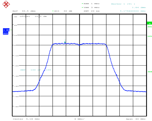
802.11a_5180MHz_Chain 1
