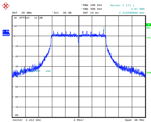
802.11g_2412MHz_Chain 1
