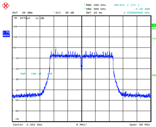
802.11n40_2452MHz_Chain 1
