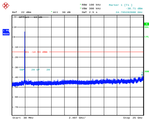
802.11g_2437MHz_Chain 1
