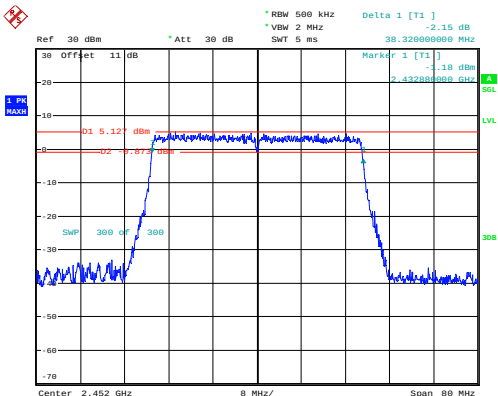
802.11ax40_2452MHz_RU_Full_Chain 1
