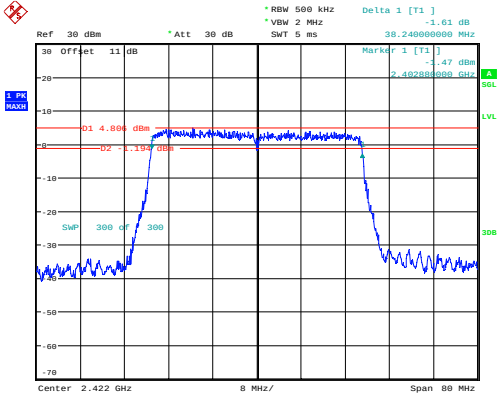
802.11ax40_2422MHz_RU_Full_Chain 0
