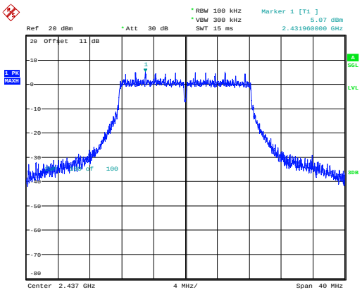
802.11g_2437MHz_Chain 1
