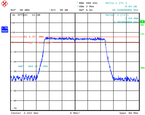
802.11ax40_2422MHz_RU_Full_Chain 1
