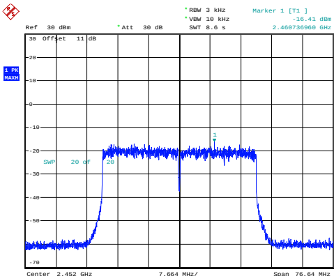
802.11ax40_2452MHz_RU_Full_Chain 1
