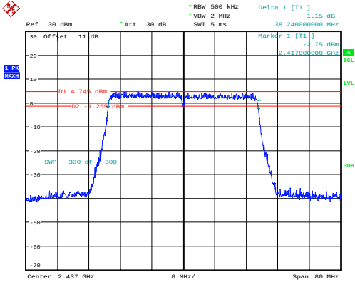
802.11ax40_2437MHz_RU_Full_Chain 0
