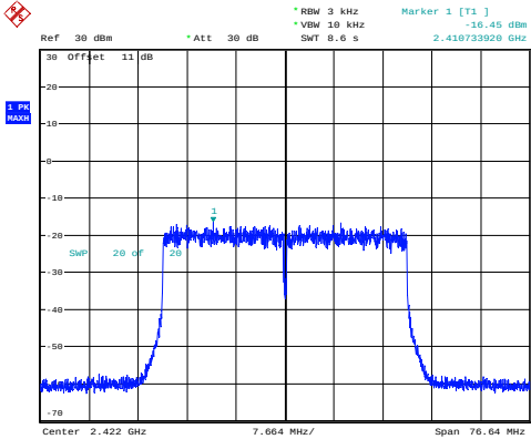
802.11ax40_2422MHz_RU_Full_Chain 1
