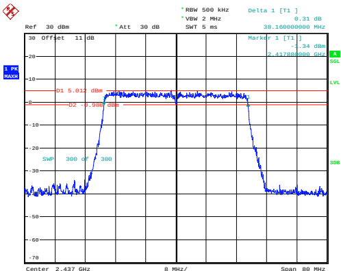
802.11ax40_2437MHz_RU_Full_Chain 1
