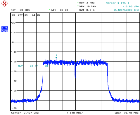
802.11ax40_2437MHz_RU_Full_Chain 0
