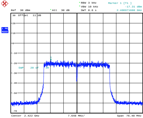
802.11ax40_2422MHz_RU_Full_Chain 0
