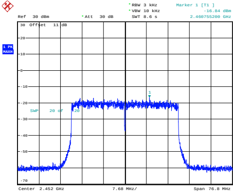
802.11ax40_2452MHz_RU_Full_Chain 0
