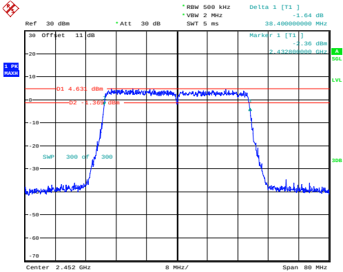
802.11ax40_2452MHz_RU_Full_Chain 0
