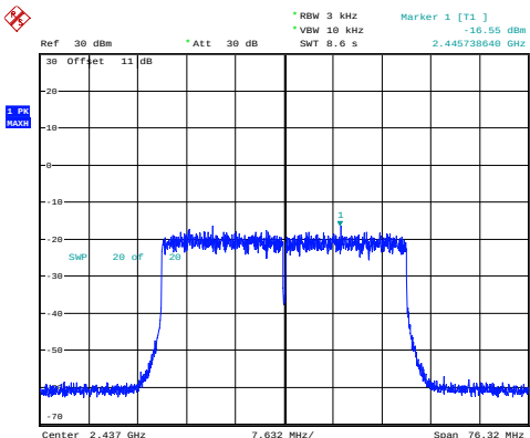
802.11ax40_2437MHz_RU_Full_Chain 1
