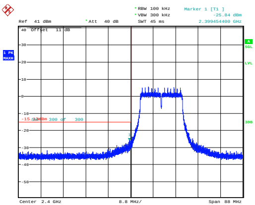
802.11g_2412MHz_Chain 1
