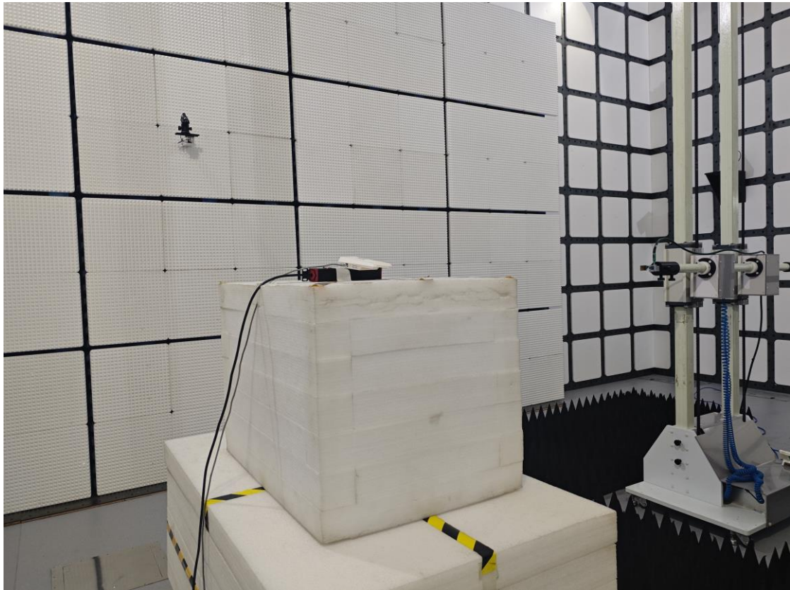
Radiated Emission 26.5-40GHz View
