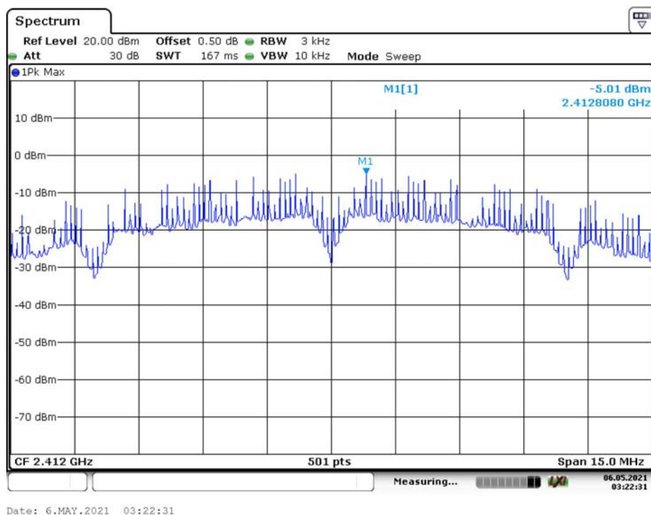
Chain 0, Power Spectral Density, 802.11b Low Channel
