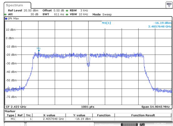
n40_2422MHz_Chain 1
