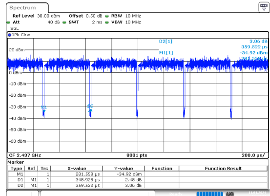
n40_2437MHz_Chain 0
