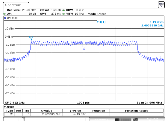
g_2412MHz_Chain 1
