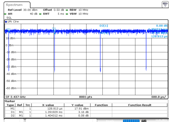
g_2437MHz_Chain 0
