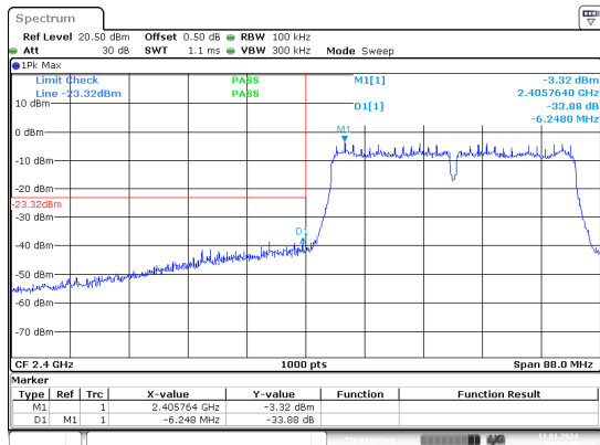
n40_2422MHz_Chain 0
