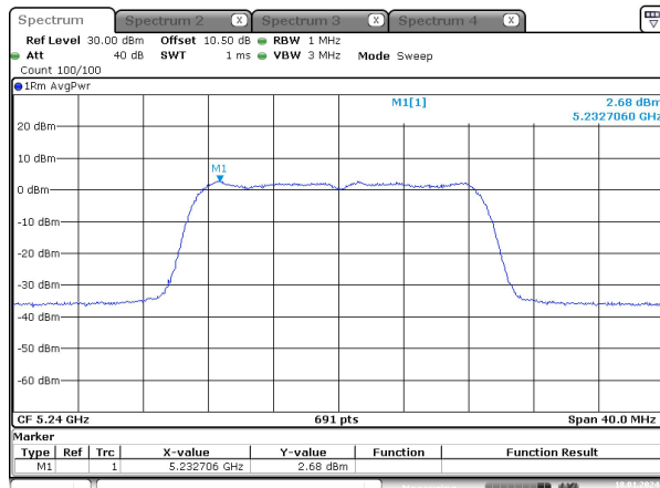
ac20_5240MHz_Chain 0
