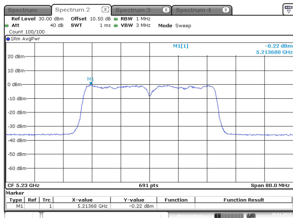
ac40_5230MHz_Chain 0
