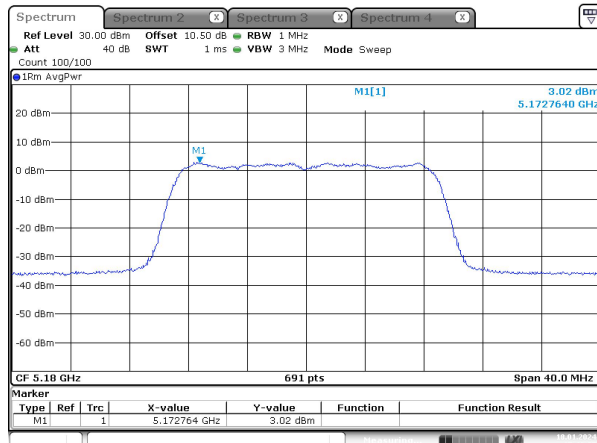
ac20_5180MHz_Chain 0
