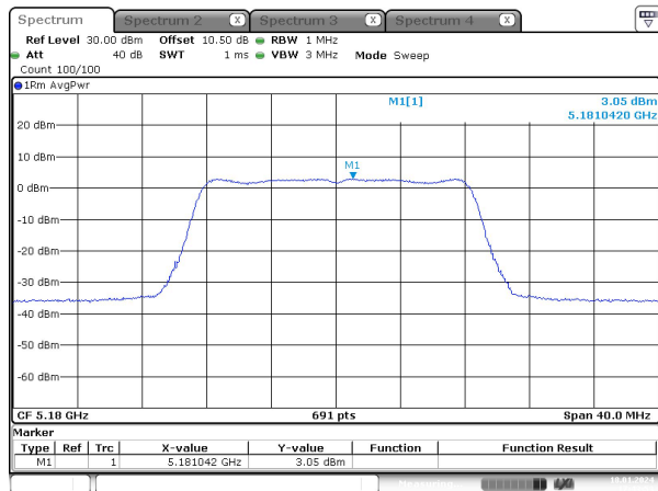
a_ 5180 MHz_Chain 0
