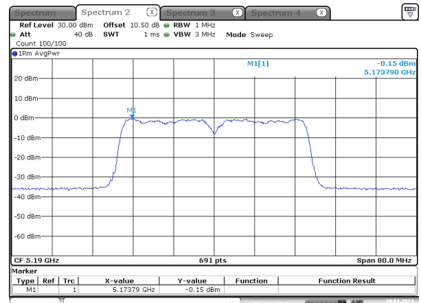
ac40_5190MHz_Chain 0
