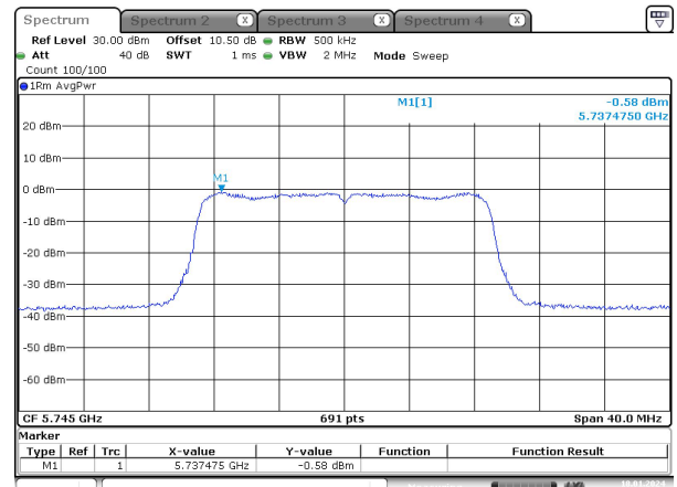
n20_ 5745MHz_Chain 0
