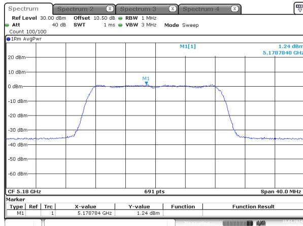
ac20_5180MHz_Chain 1
