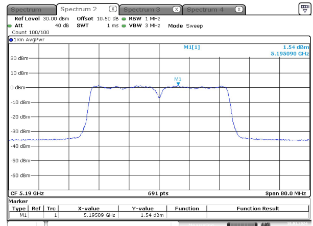
ac40_5190MHz_Chain 1
