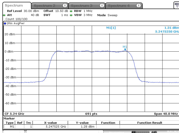
ac20_5240MHz_Chain 1
