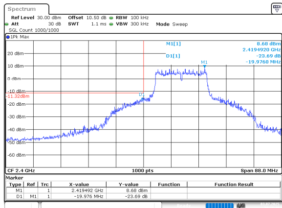
802.11g_2412MHz_Chain 1
