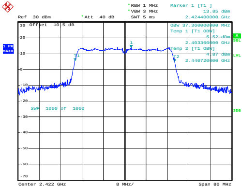
802.11n40_2422MHz_Chain 0
