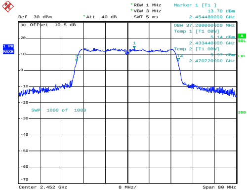
802.11n40_2452MHz_Chain 0
