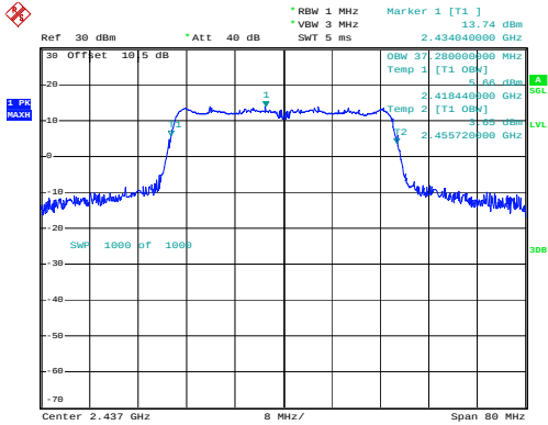
802.11n40_2437MHz_Chain 0
