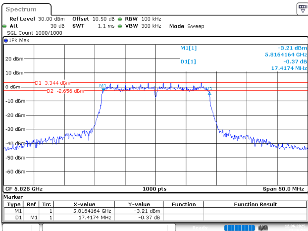
802.11n20_5825MHz
