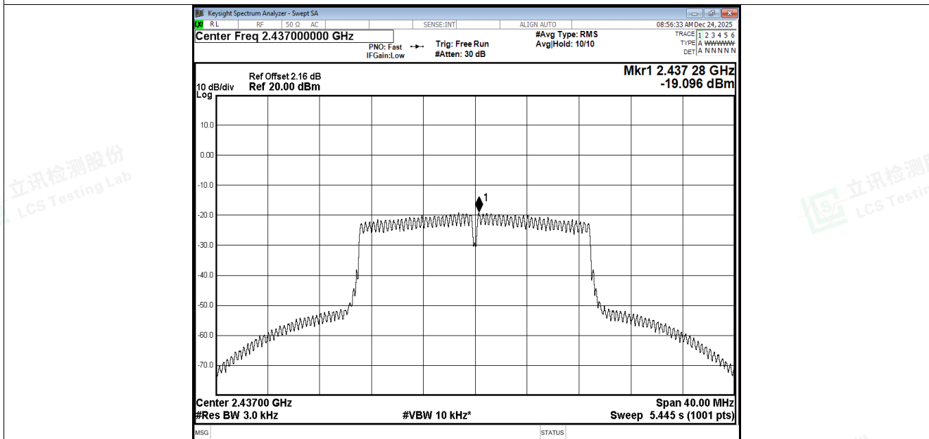
PSD NVNT n20 2437MHz Ant2
