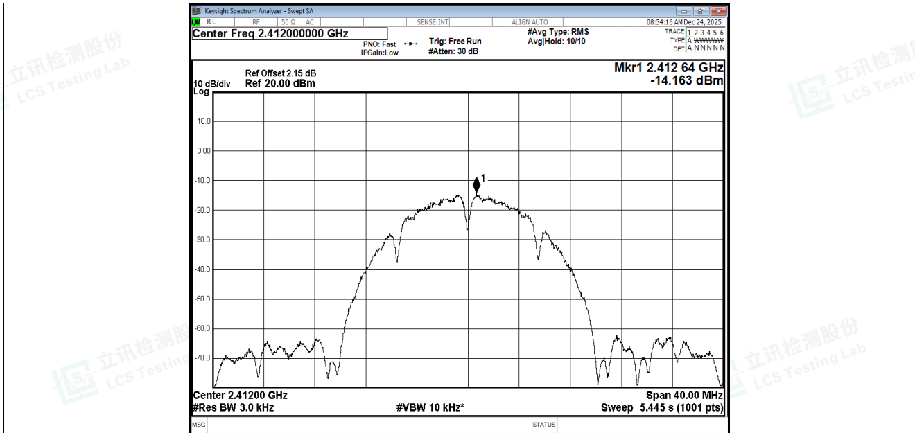
PSD NVNT b 2412MHz Ant2
