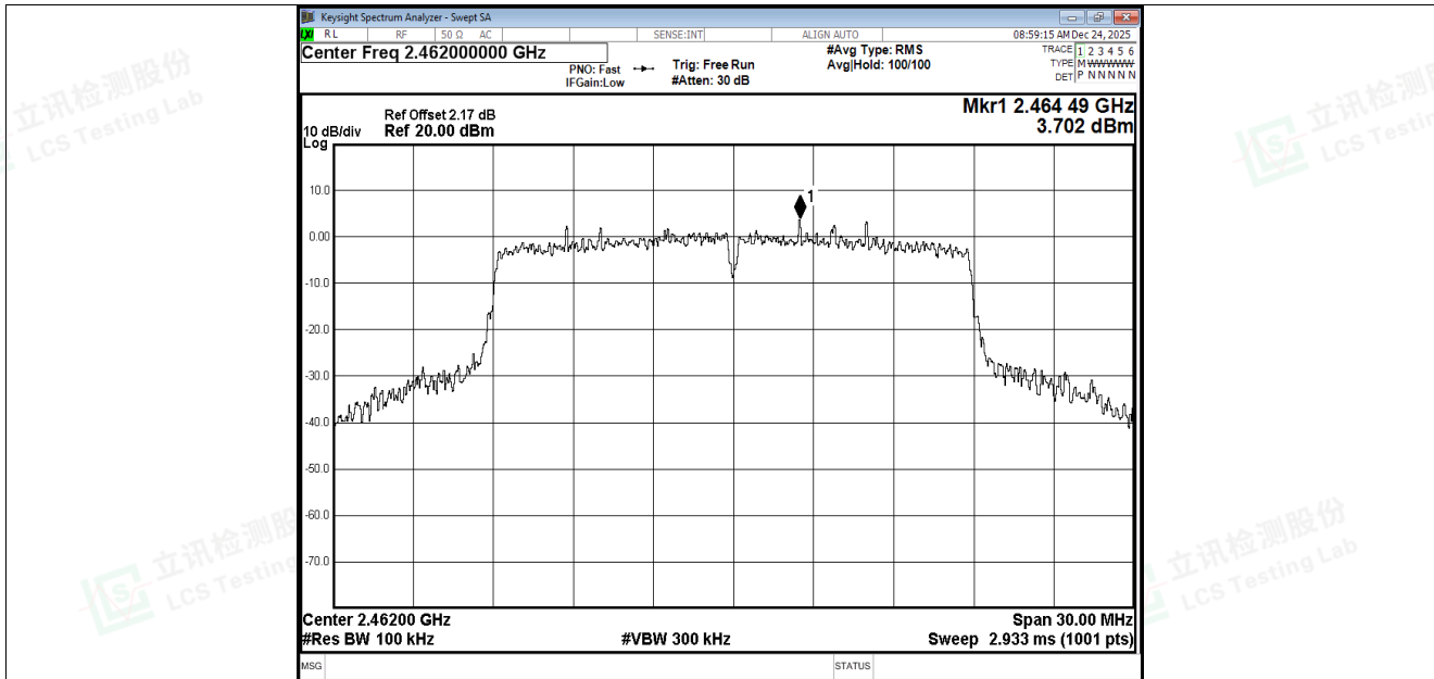
Band Edge NVNT n20 2462MHz Ant2 Ref
