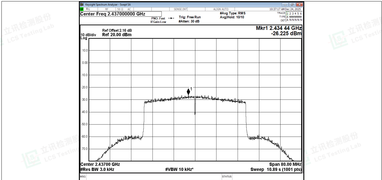
PSD NVNT ax40 2437MHz Ant3
