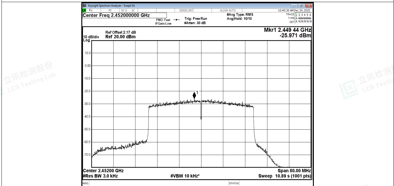
PSD NVNT ax40 2452MHz Ant3
