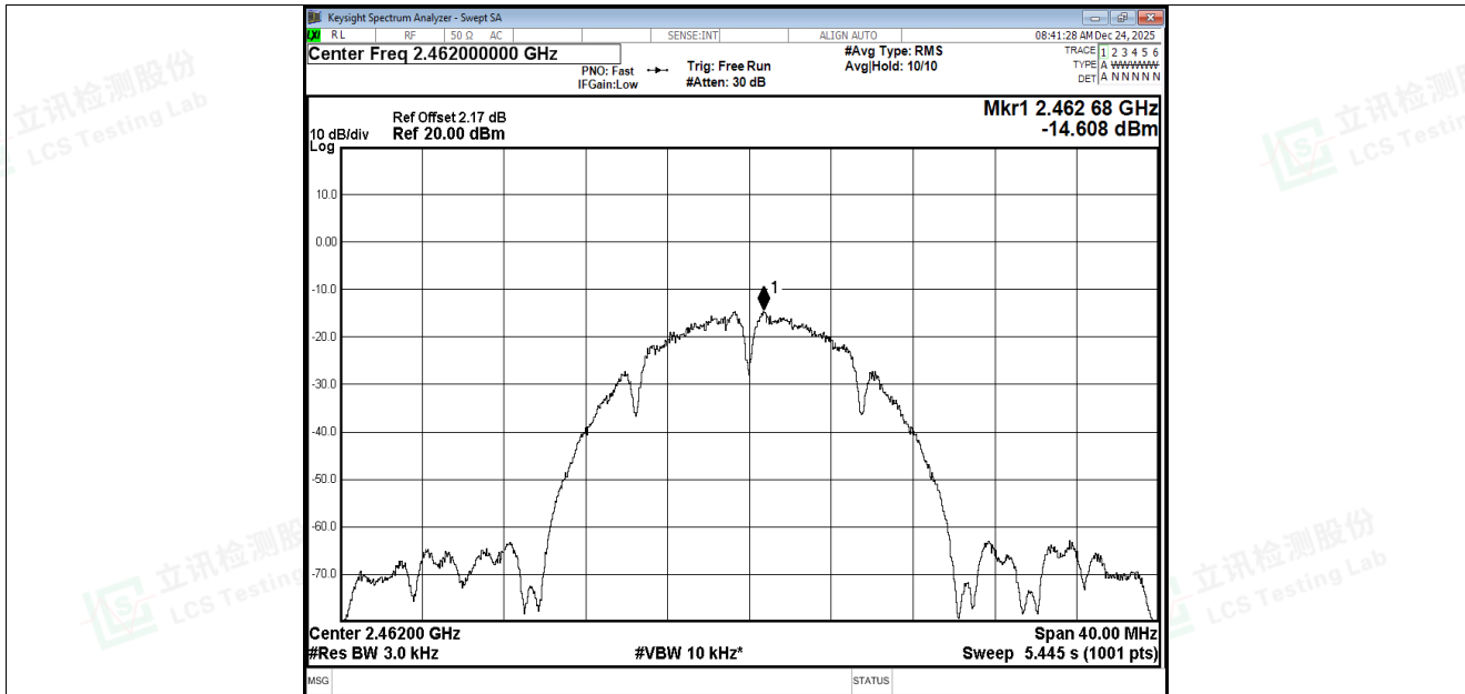
PSD NVNT b 2462MHz Ant2
