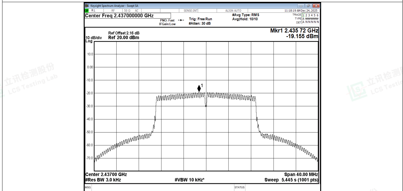
PSD NVNT n20 2437MHz Ant4
