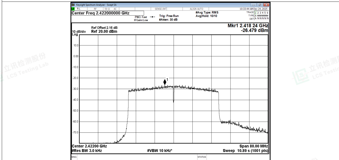
PSD NVNT ax40 2422MHz Ant3
