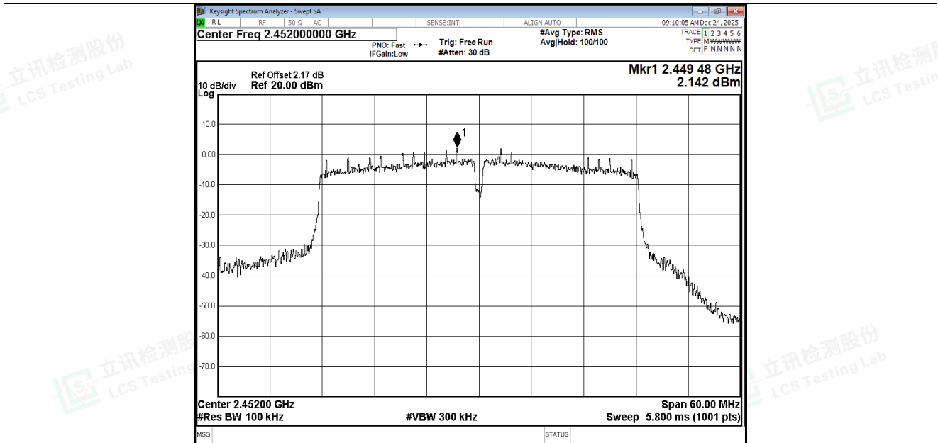
Band Edge NVNT n40 2452MHz Ant2 Ref
