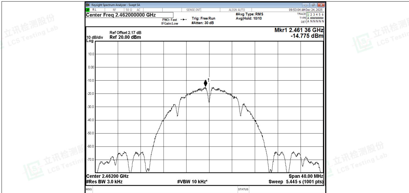
PSD NVNT b 2462MHz Ant3
