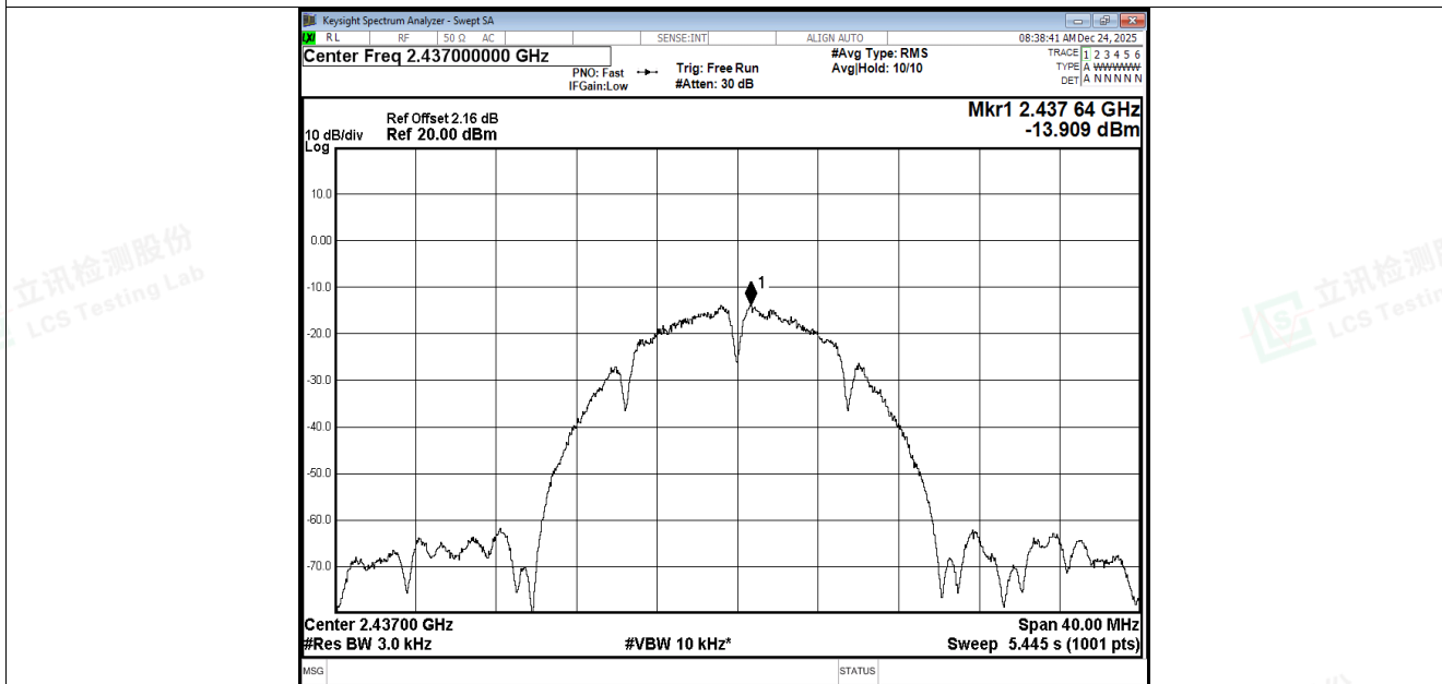
PSD NVNT b 2437MHz Ant2
