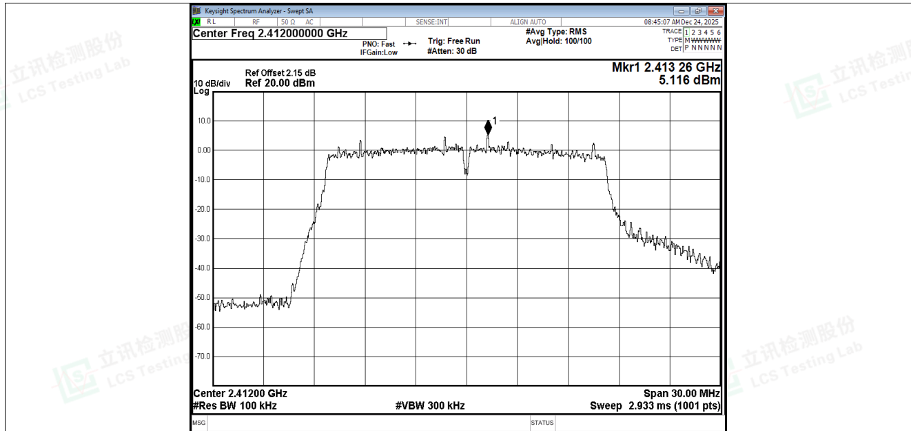
Band Edge NVNT g 2412MHz Ant2 Ref
