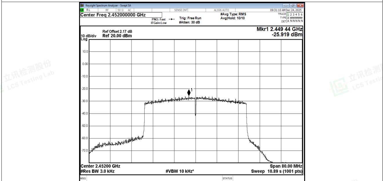
PSD NVNT ax40 2452MHz Ant2
