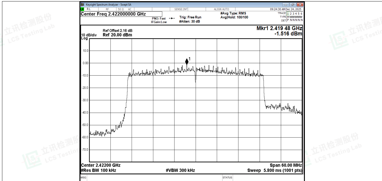
Band Edge NVNT ax40 2422MHz Ant2 Ref
