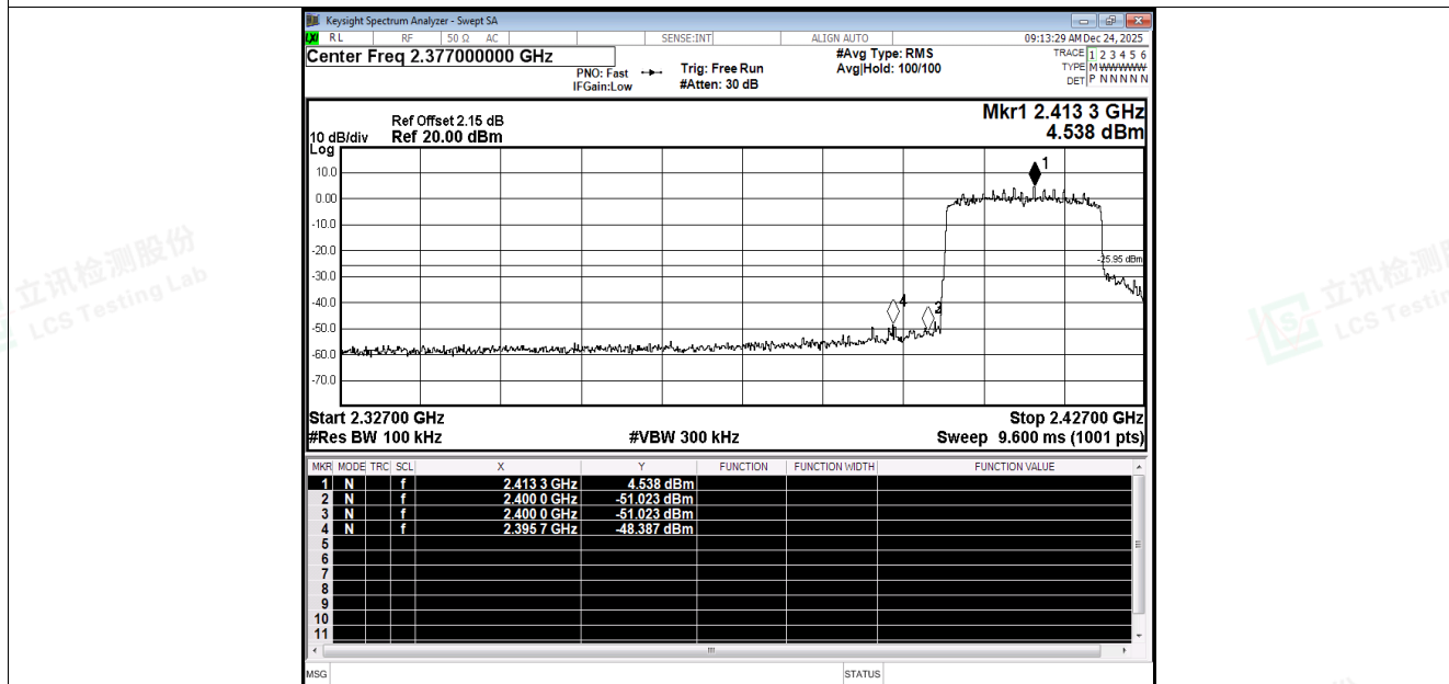
Band Edge NVNT ax20 2412MHz Ant2 Emission
