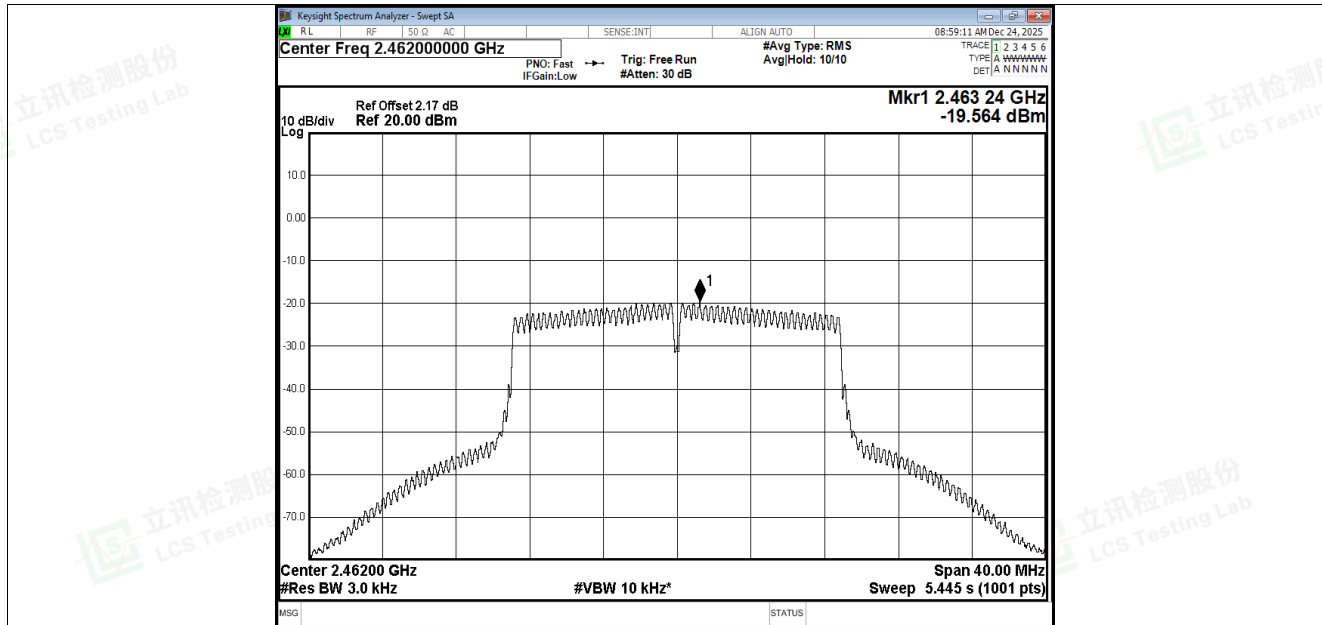
PSD NVNT n20 2462MHz Ant2
