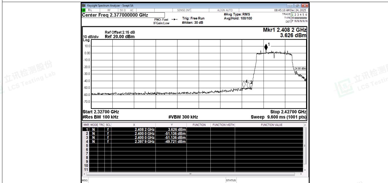
Band Edge NVNT g 2412MHz Ant2 Emission
