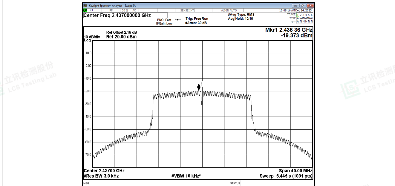
PSD NVNT n20 2437MHz Ant3
