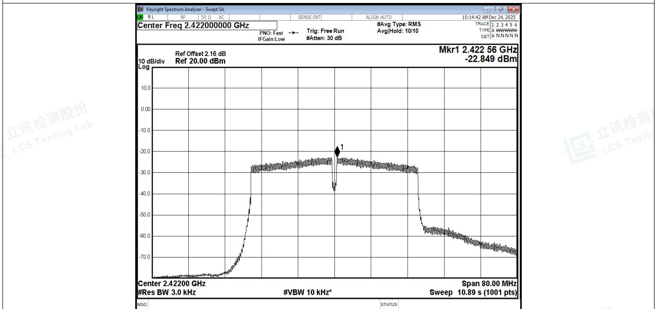
PSD NVNT n40 2422MHz Ant3
