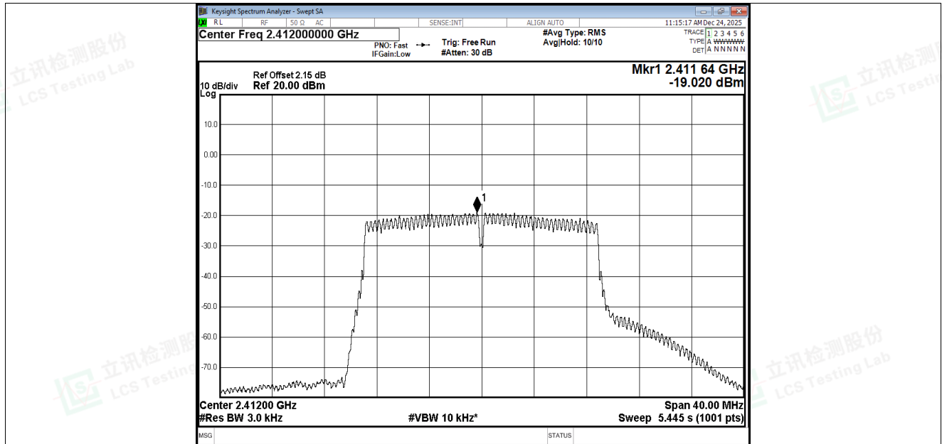
PSD NVNT n20 2412MHz Ant4
