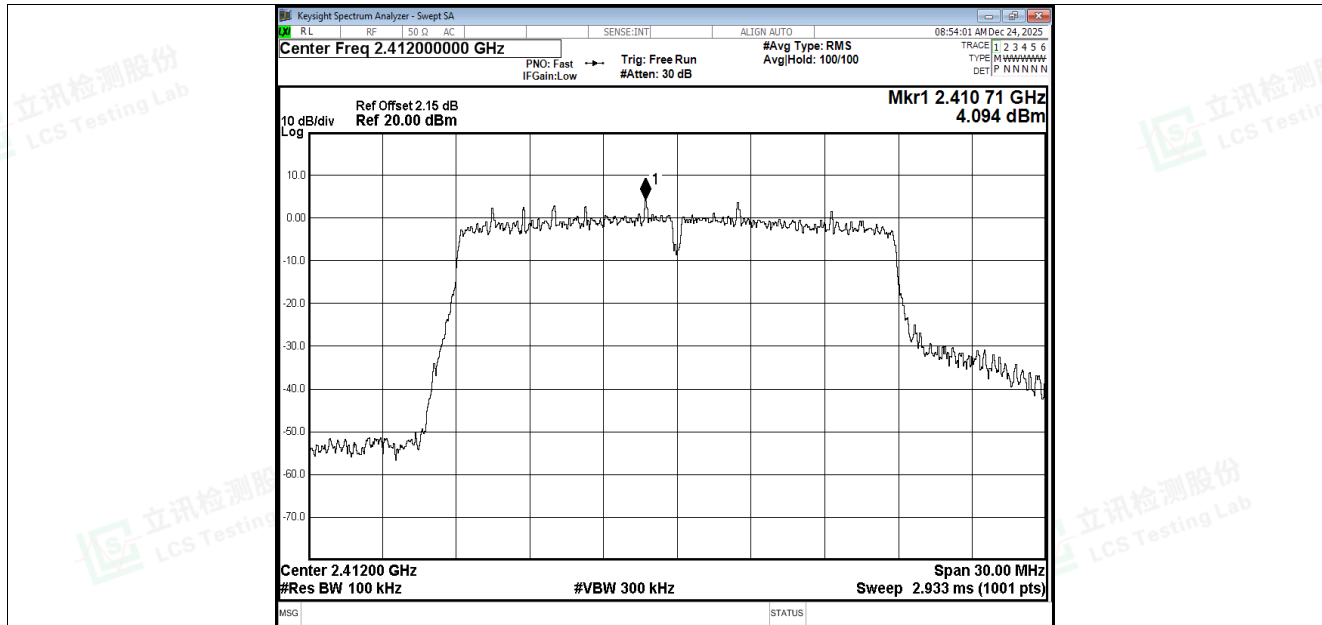
Band Edge NVNT n20 2412MHz Ant2 Ref
