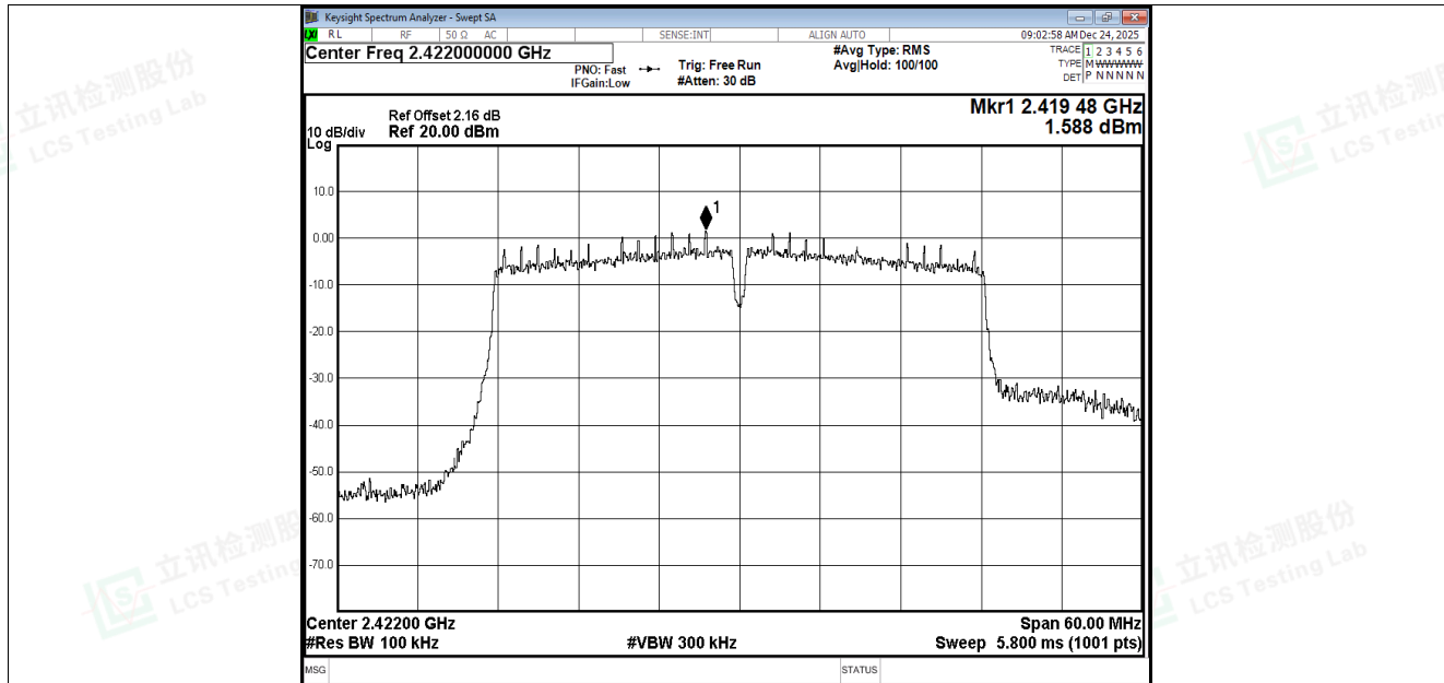
Band Edge NVNT n40 2422MHz Ant2 Ref
