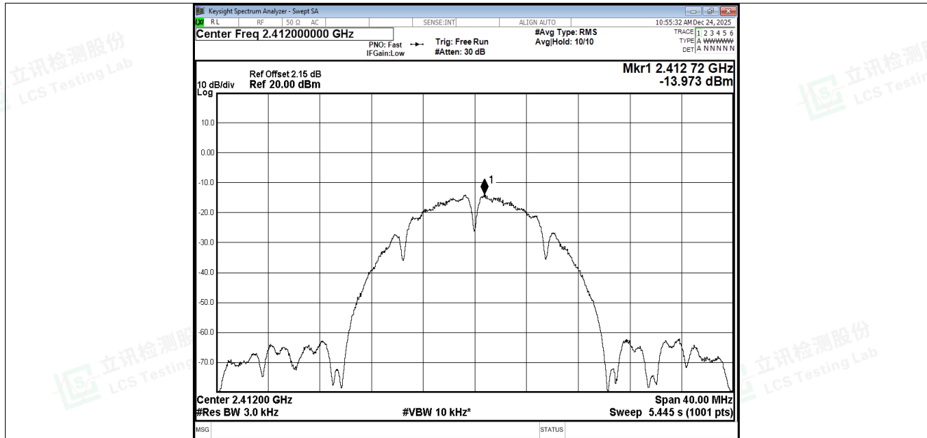
PSD NVNT b 2412MHz Ant4
