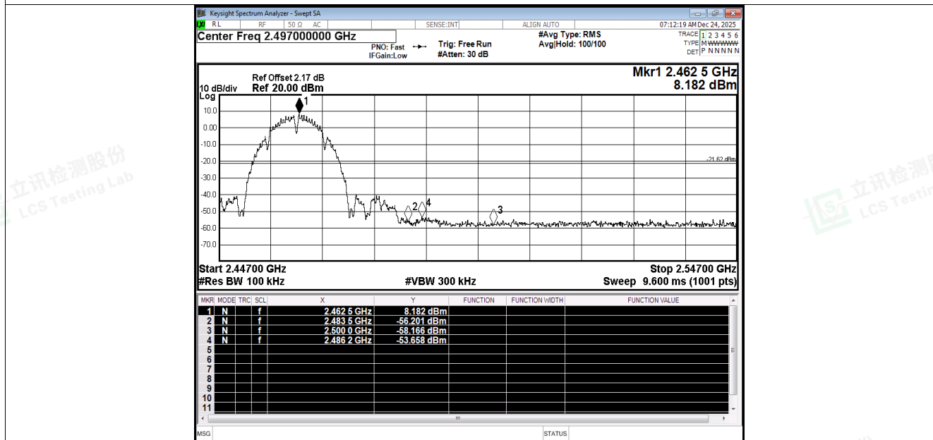
Band Edge NVNT b 2462MHz Ant1 Emission
