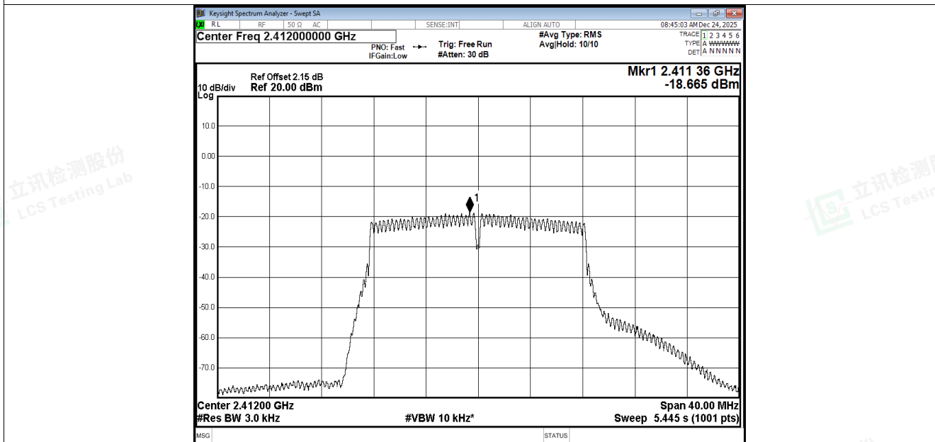
PSD NVNT g 2412MHz Ant2
