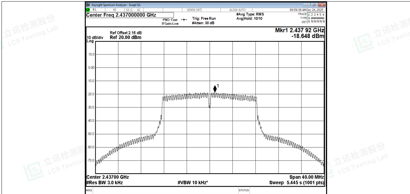
PSD NVNT g 2437MHz Ant3
