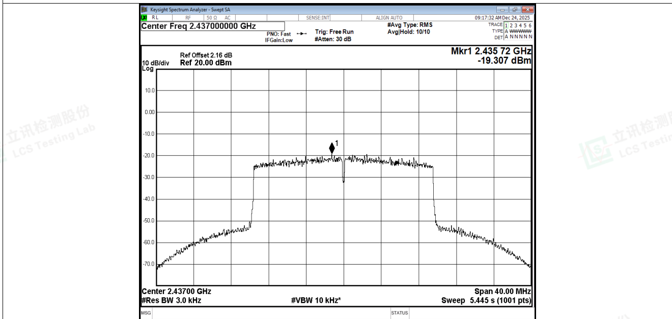
PSD NVNT ax20 2437MHz Ant2
