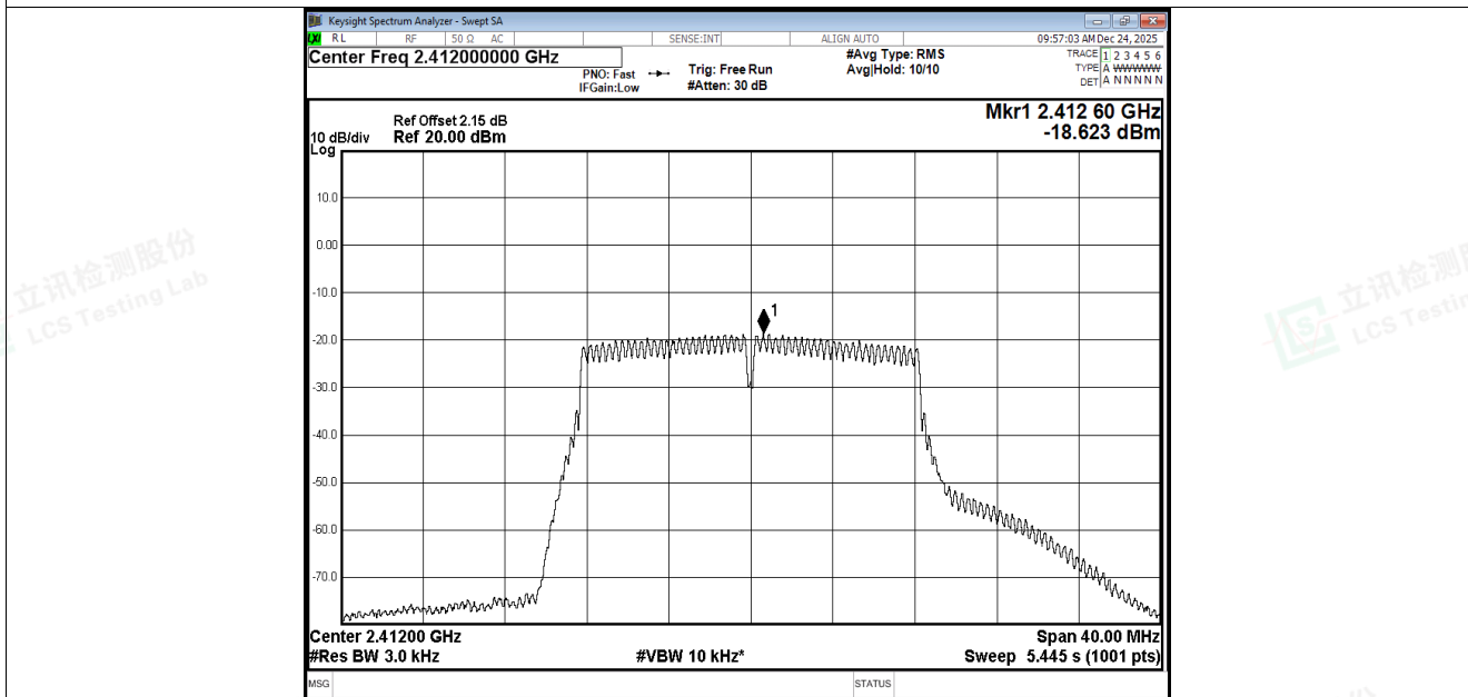
PSD NVNT g 2412MHz Ant3
