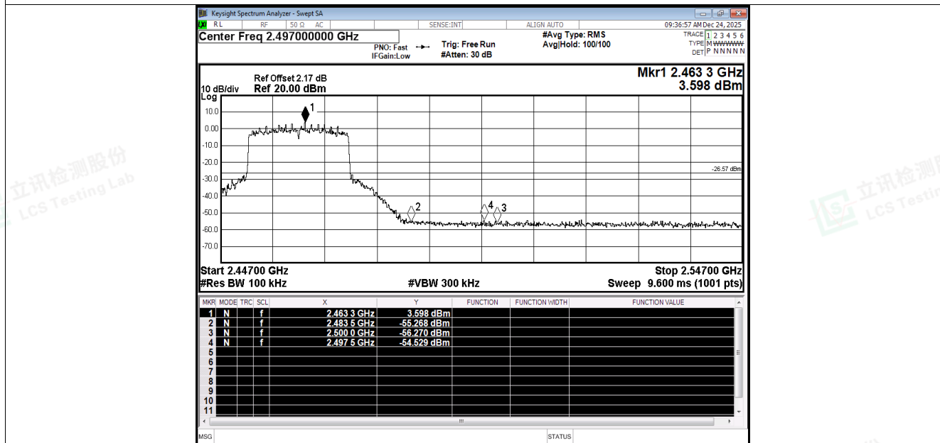
Band Edge NVNT be20 2462MHz Ant2 Emission
