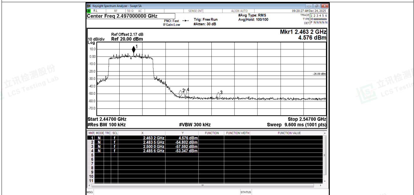
Band Edge NVNT ax20 2462MHz Ant2 Emission
