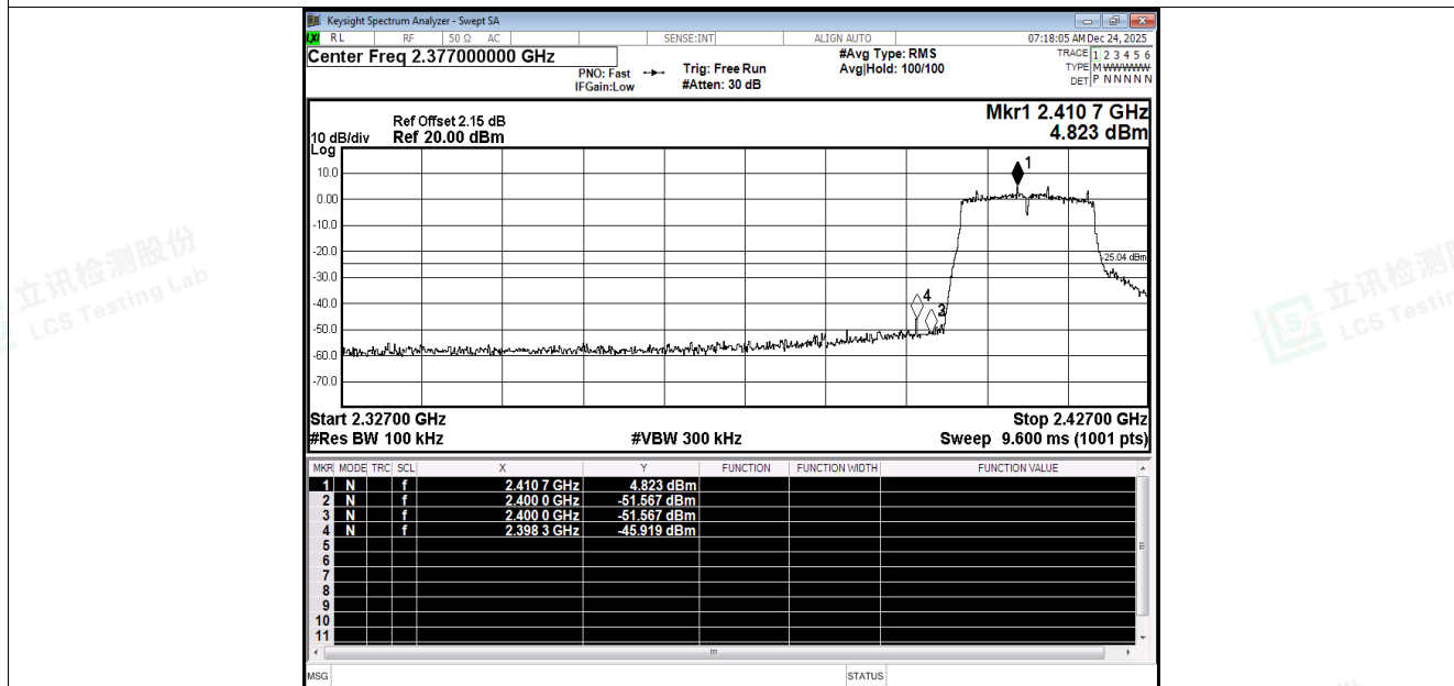
Band Edge NVNT g 2412MHz Ant1 Emission
