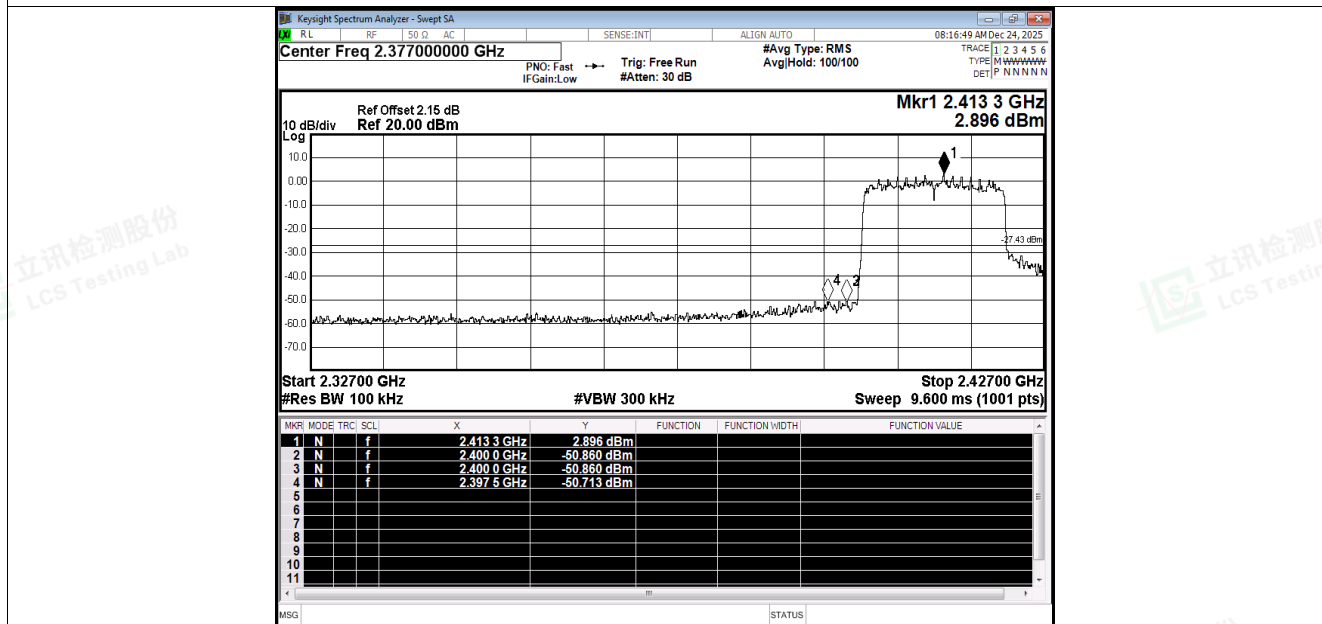
Band Edge NVNT be20 2412MHz Ant1 Emission
