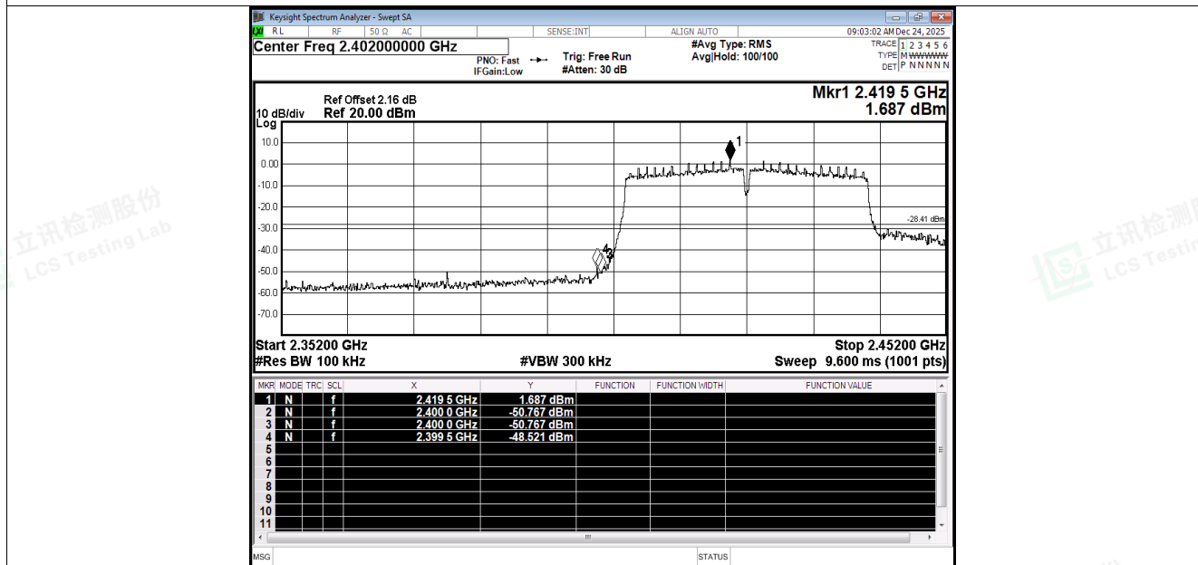
Band Edge NVNT n40 2422MHz Ant2 Emission
