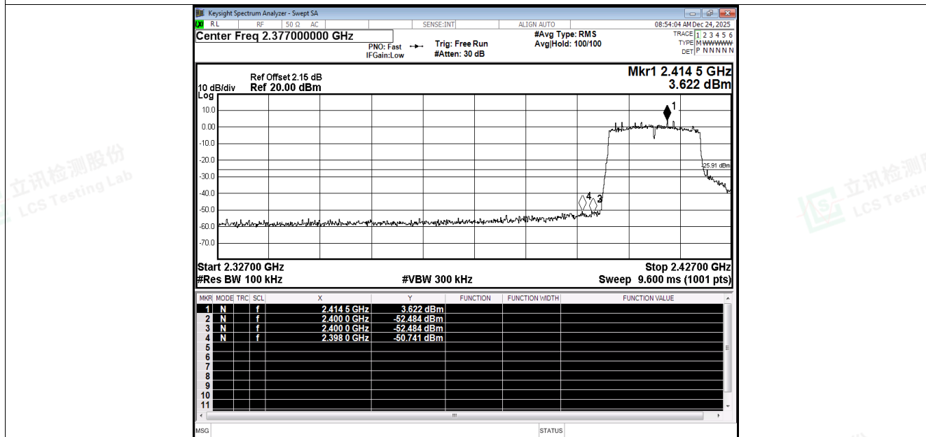
Band Edge NVNT n20 2412MHz Ant2 Emission
