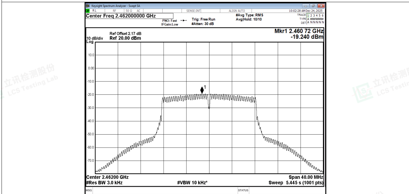
PSD NVNT g 2462MHz Ant3
