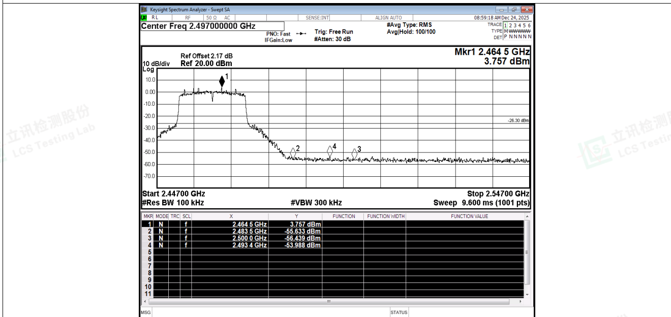
Band Edge NVNT n20 2462MHz Ant2 Emission
