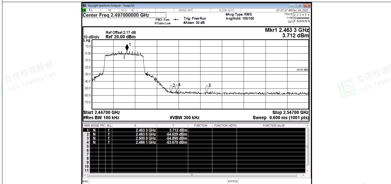
Band Edge NVNT n20 2462MHz Ant1 Emission
