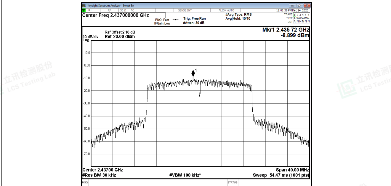
PSD NVNT be20 2437MHz Ant4
