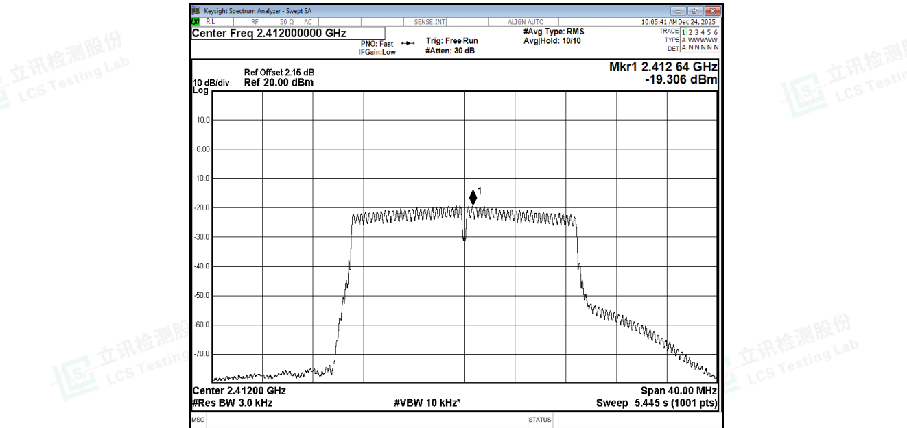
PSD NVNT n20 2412MHz Ant3
