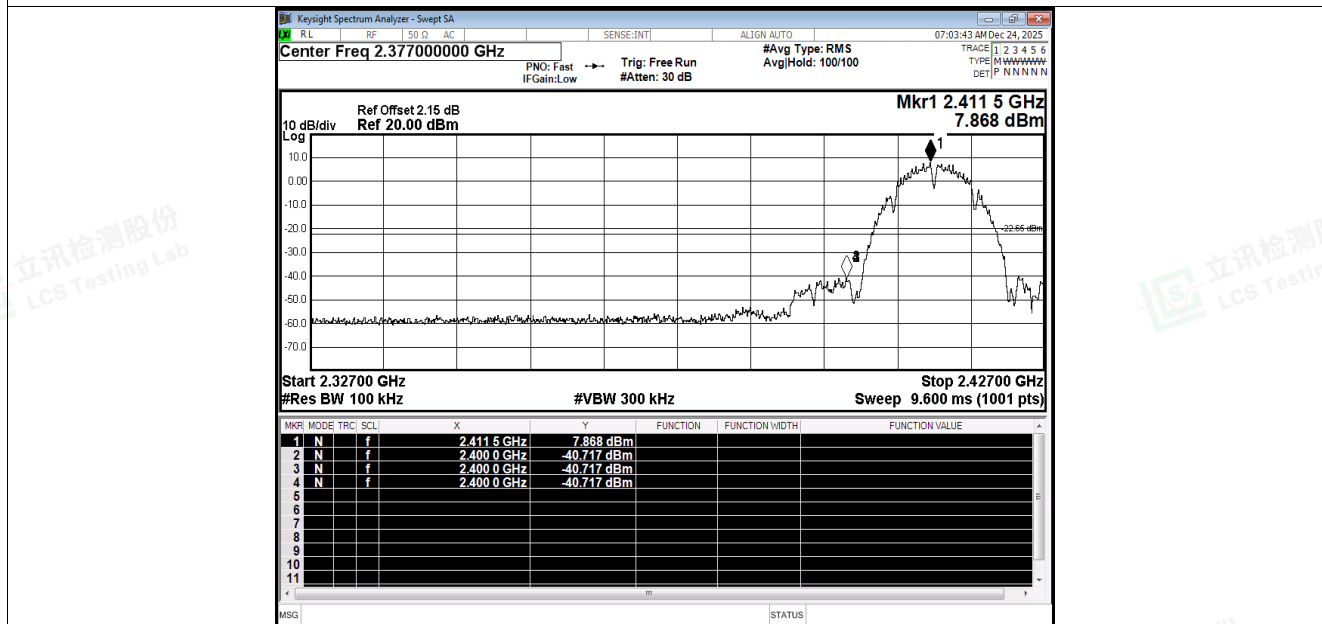
Band Edge NVNT b 2412MHz Ant1 Emission
