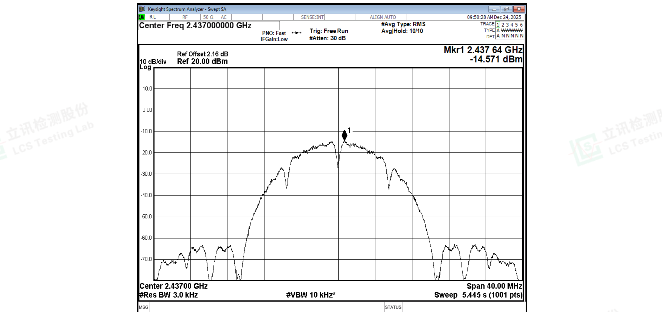
PSD NVNT b 2437MHz Ant3
