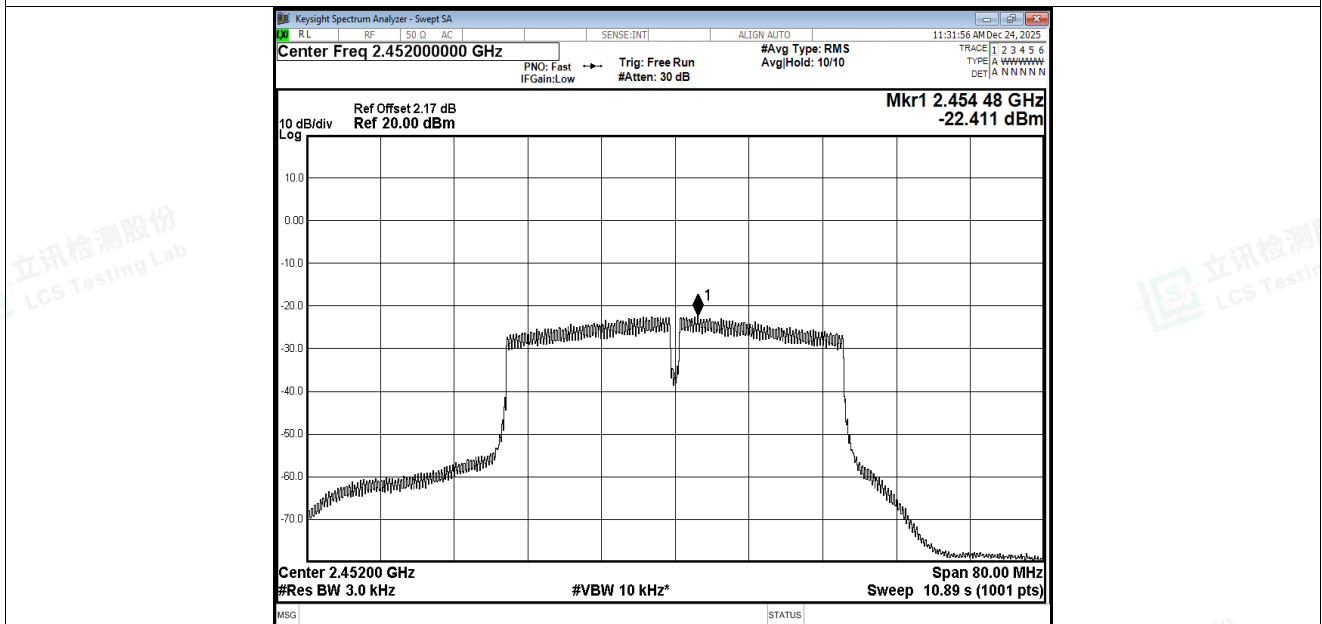
PSD NVNT n40 2452MHz Ant4
