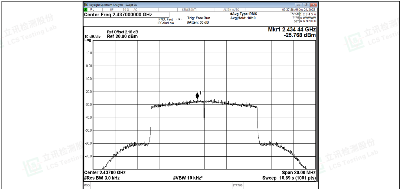
PSD NVNT ax40 2437MHz Ant2
