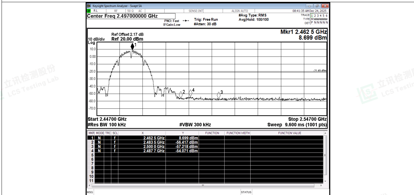
Band Edge NVNT b 2462MHz Ant2 Emission
