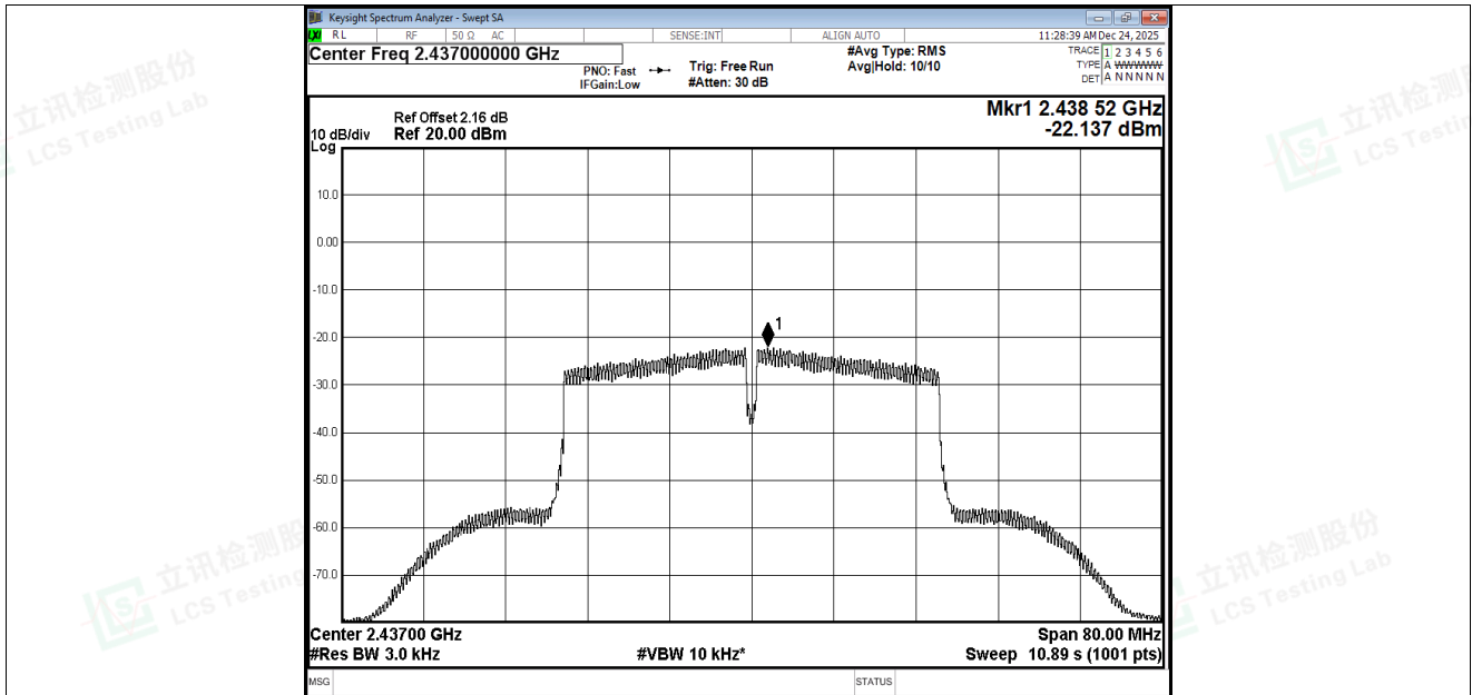
PSD NVNT n40 2437MHz Ant4
