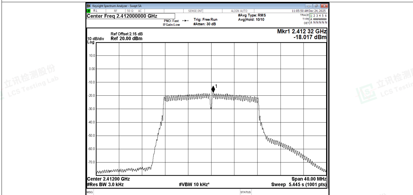
PSD NVNT g 2412MHz Ant4
