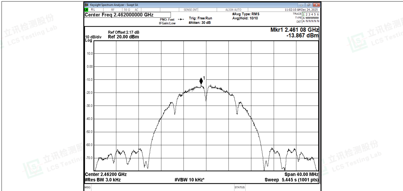
PSD NVNT b 2462MHz Ant4
