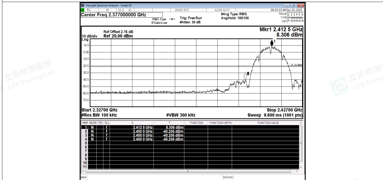
Band Edge NVNT b 2412MHz Ant2 Emission
