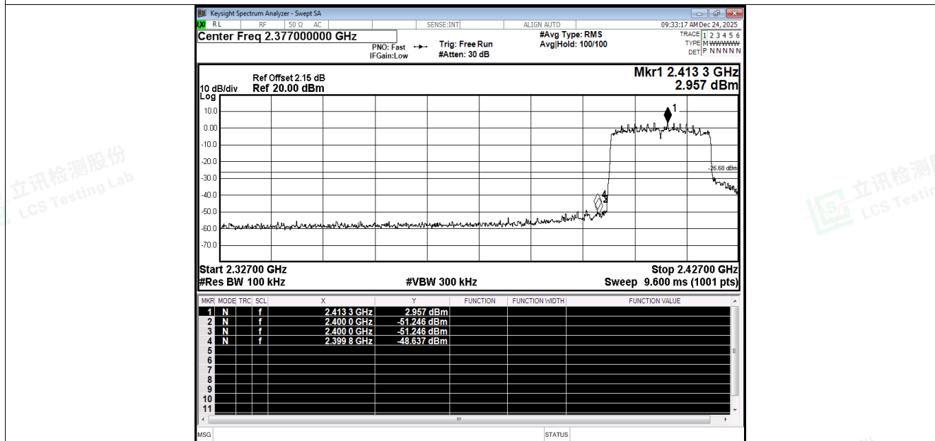
Band Edge NVNT be20 2412MHz Ant2 Emission
