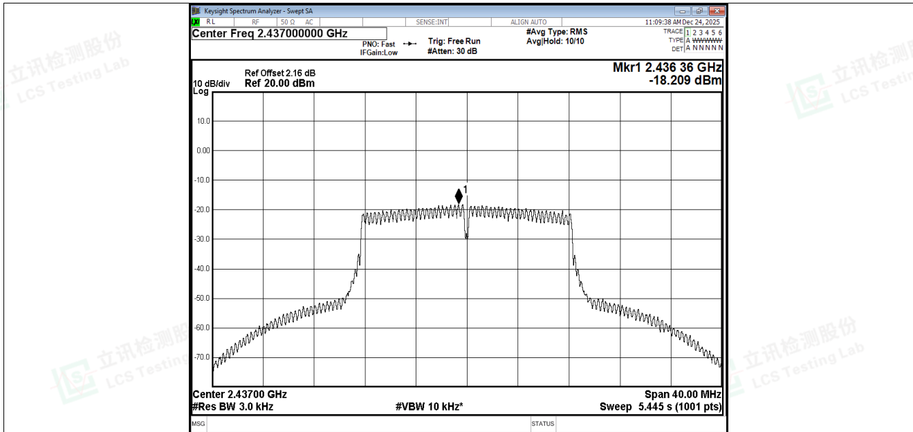
PSD NVNT g 2437MHz Ant4
