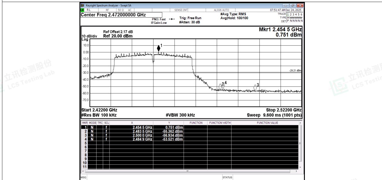
Band Edge NVNT n40 2452MHz Ant1 Emission
