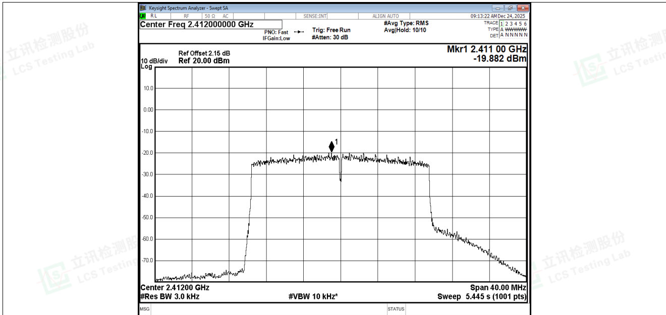
PSD NVNT ax20 2412MHz Ant2
