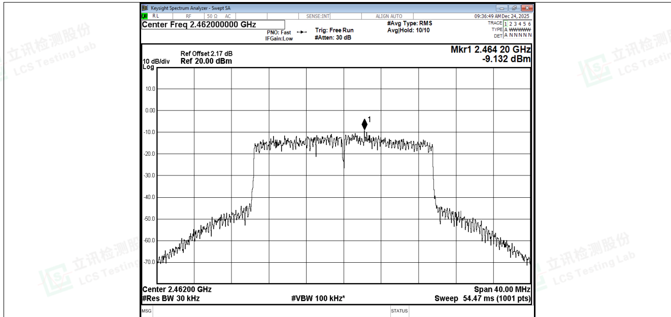
PSD NVNT be20 2462MHz Ant2
