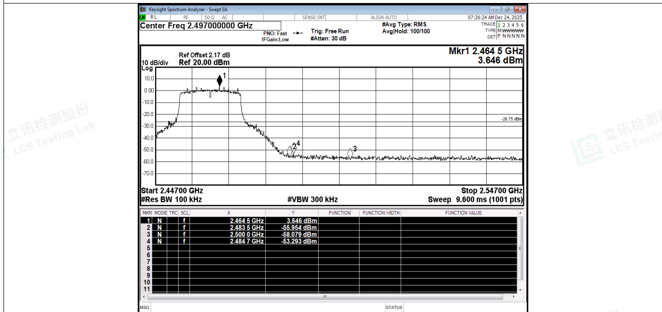
Band Edge NVNT g 2462MHz Ant1 Emission
