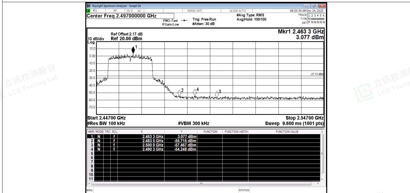
Band Edge NVNT be20 2462MHz Ant1 Emission
