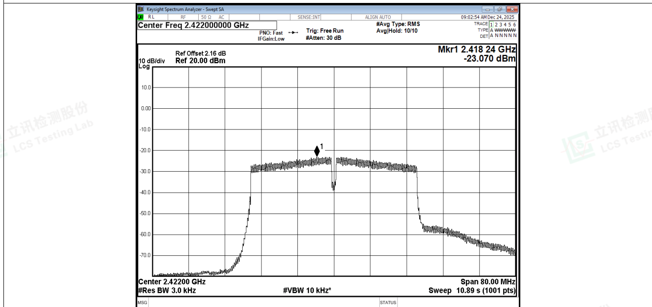
PSD NVNT n40 2422MHz Ant2
