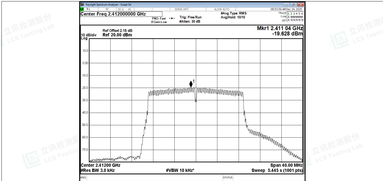
PSD NVNT n20 2412MHz Ant2
