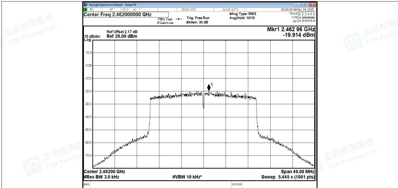
PSD NVNT ax20 2462MHz Ant2
