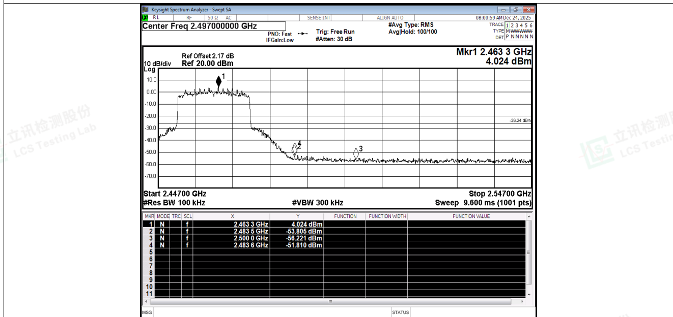
Band Edge NVNT ax20 2462MHz Ant1 Emission
