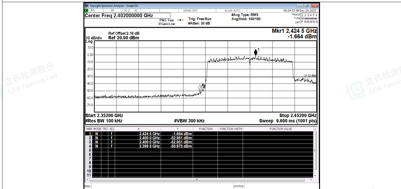
Band Edge NVNT ax40 2422MHz Ant2 Emission
