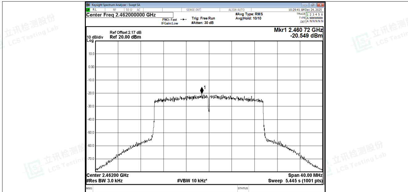
PSD NVNT ax20 2462MHz Ant3
