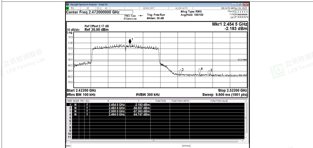
Band Edge NVNT ax40 2452MHz Ant1 Emission
