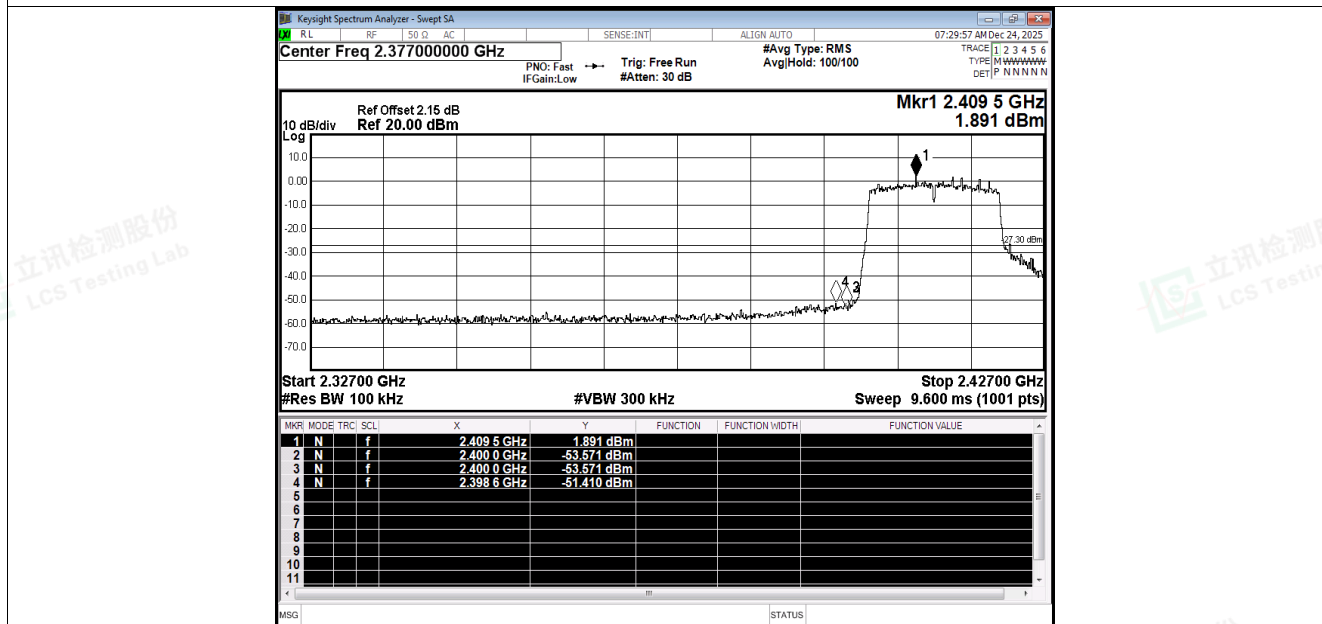
Band Edge NVNT n20 2412MHz Ant1 Emission
