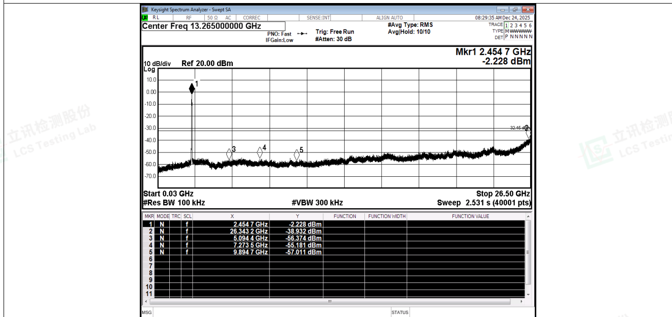
Tx. Spurious NVNT be40 2452MHz Ant1 Emission
