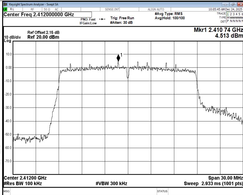
Band Edge NVNT n20 2412MHz Ant3 Ref
