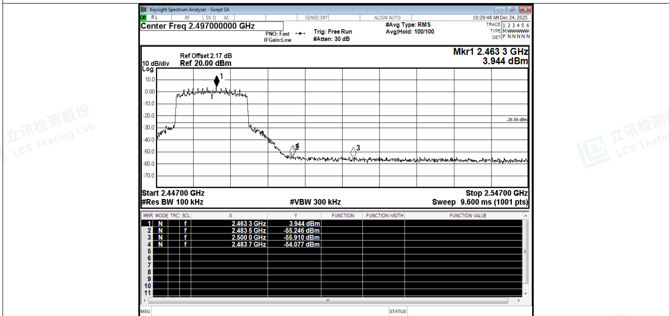
Band Edge NVNT ax20 2462MHz Ant3 Emission
