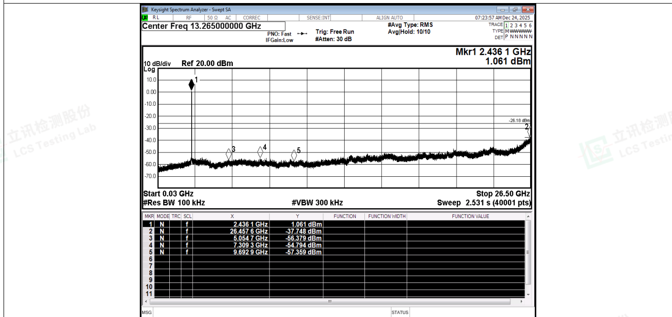
Tx. Spurious NVNT g 2437MHz Ant1 Emission
