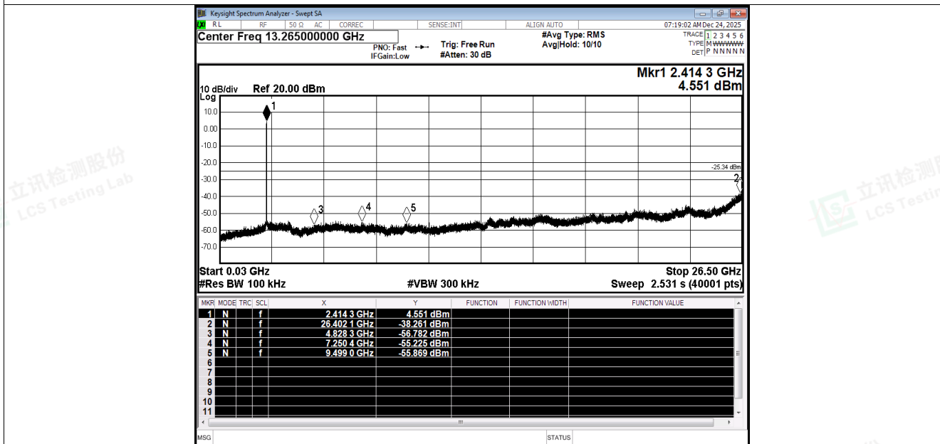
Tx. Spurious NVNT g 2412MHz Ant1 Emission
