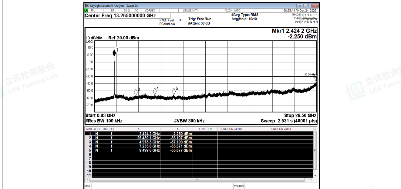
Tx. Spurious NVNT be40 2422MHz Ant1 Emission
