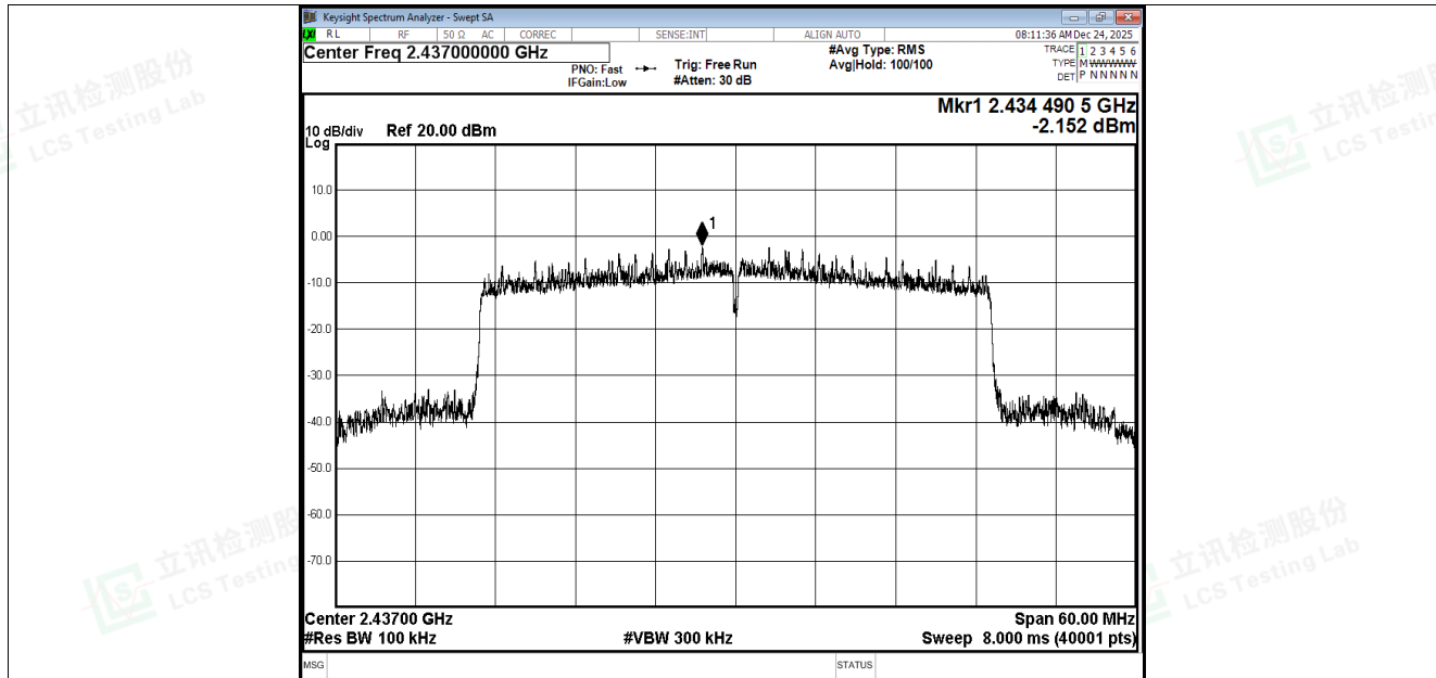
Tx. Spurious NVNT ax40 2437MHz Ant1 Ref
