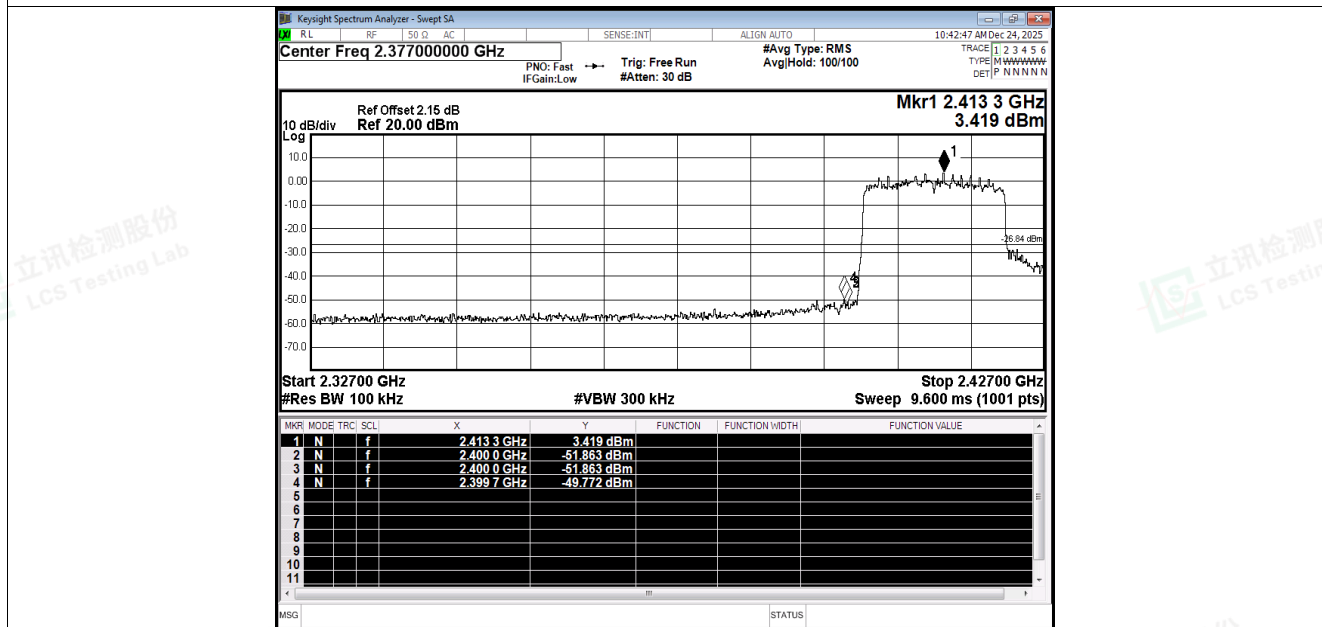
Band Edge NVNT be20 2412MHz Ant3 Emission
