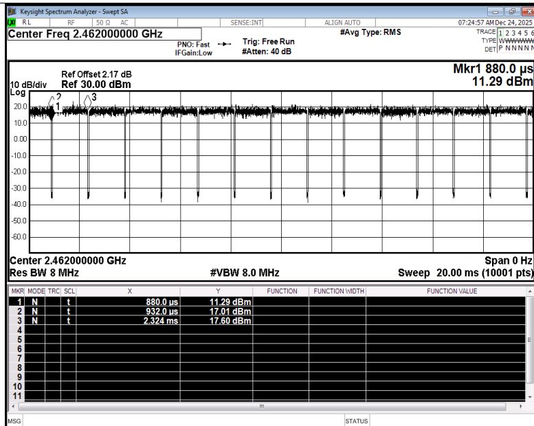
Duty Cycle NVNT g 2462MHz Ant1
