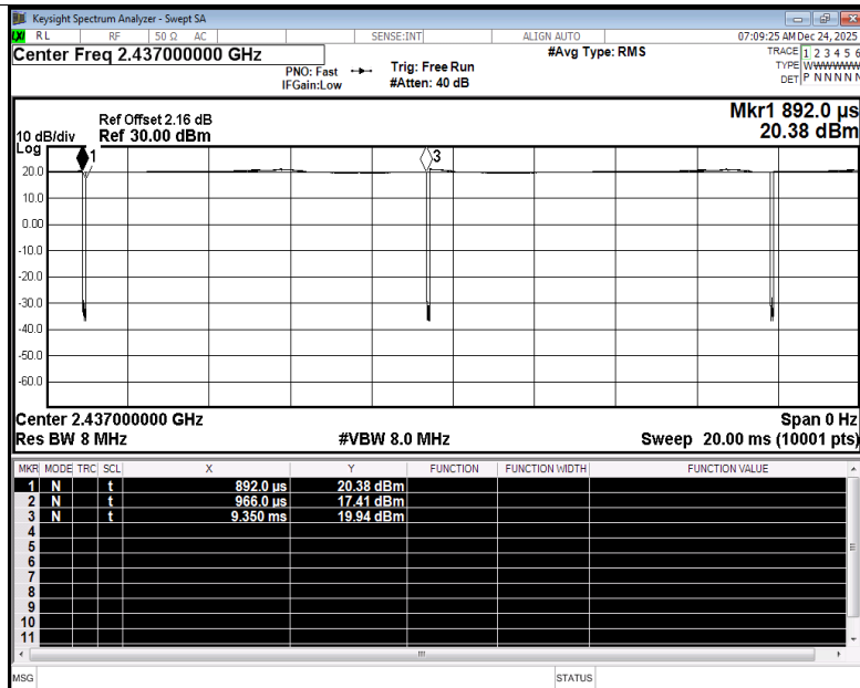
Duty Cycle NVNT b 2437MHz Ant1
