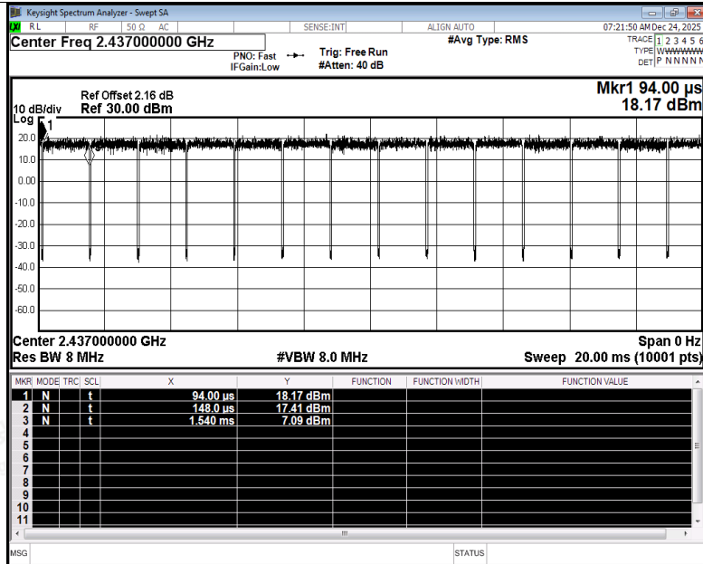
Duty Cycle NVNT g 2437MHz Ant1
