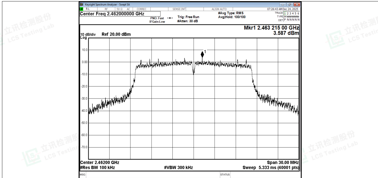
Tx. Spurious NVNT g 2462MHz Ant1 Ref
