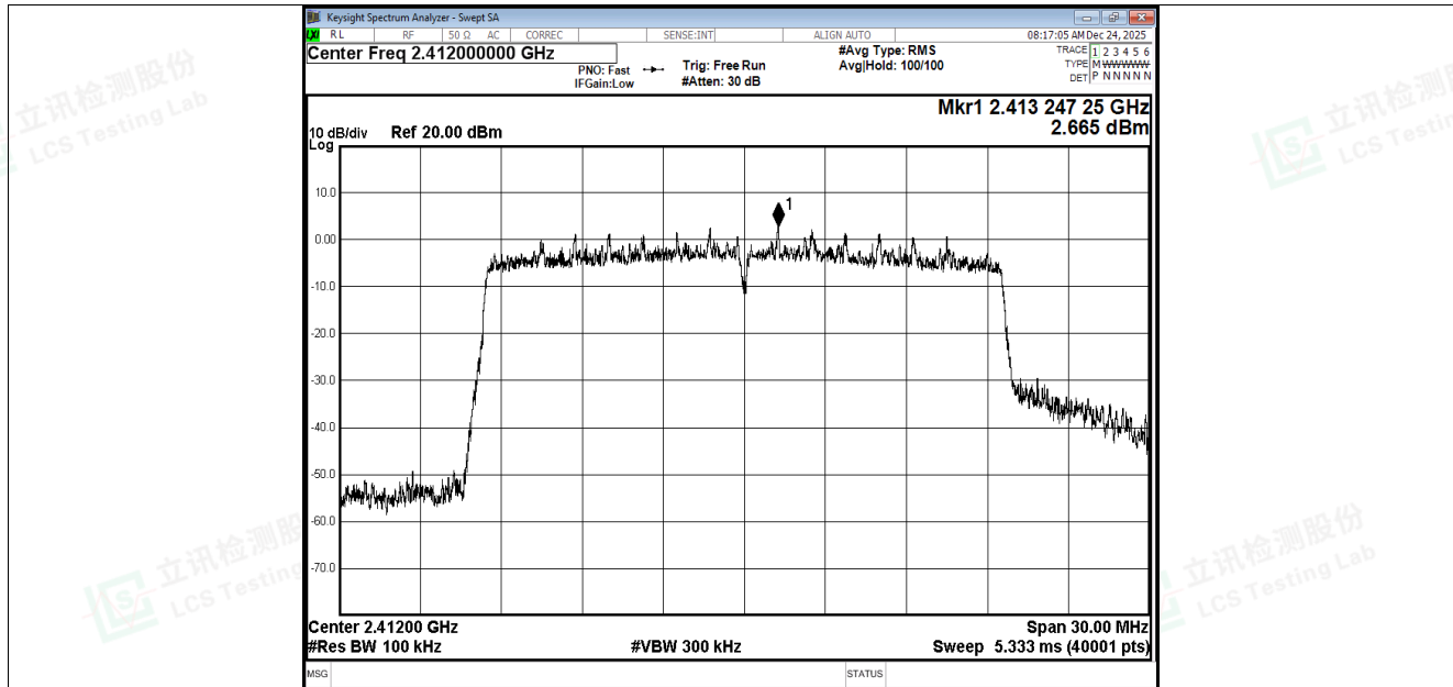
Tx. Spurious NVNT be20 2412MHz Ant1 Ref
