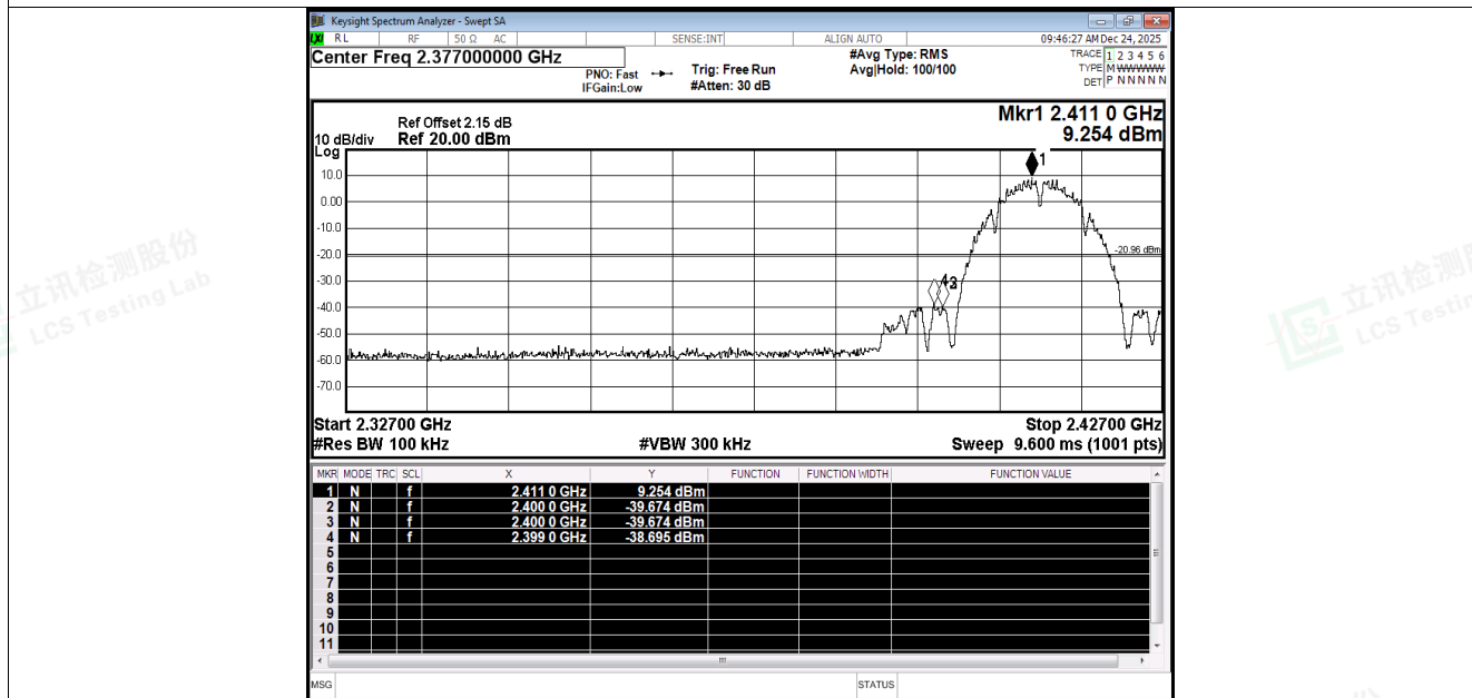
Band Edge NVNT b 2412MHz Ant3 Emission
