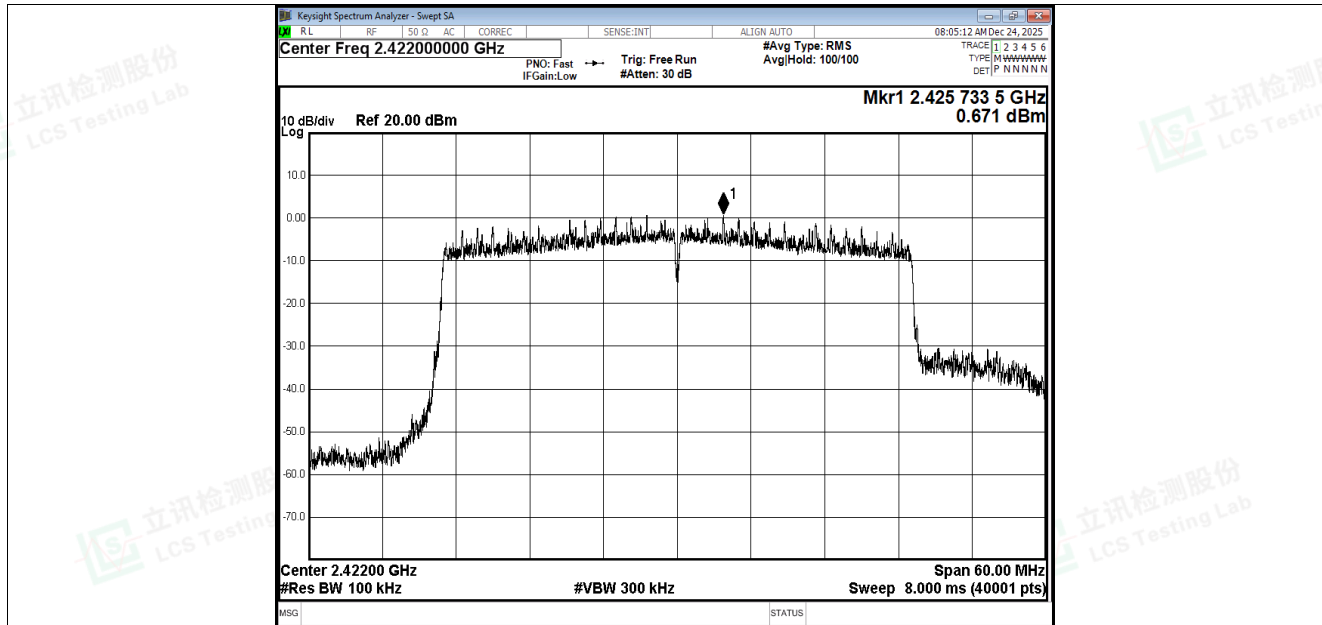
Tx. Spurious NVNT ax40 2422MHz Ant1 Ref
