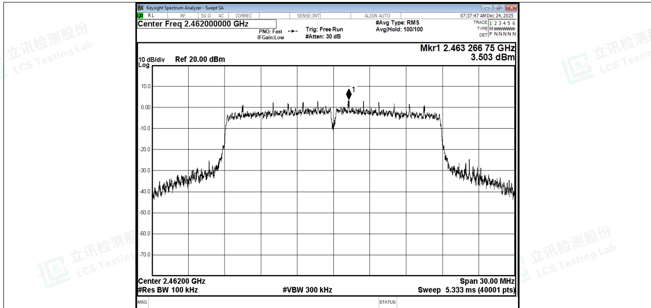
Tx. Spurious NVNT n20 2462MHz Ant1 Ref
