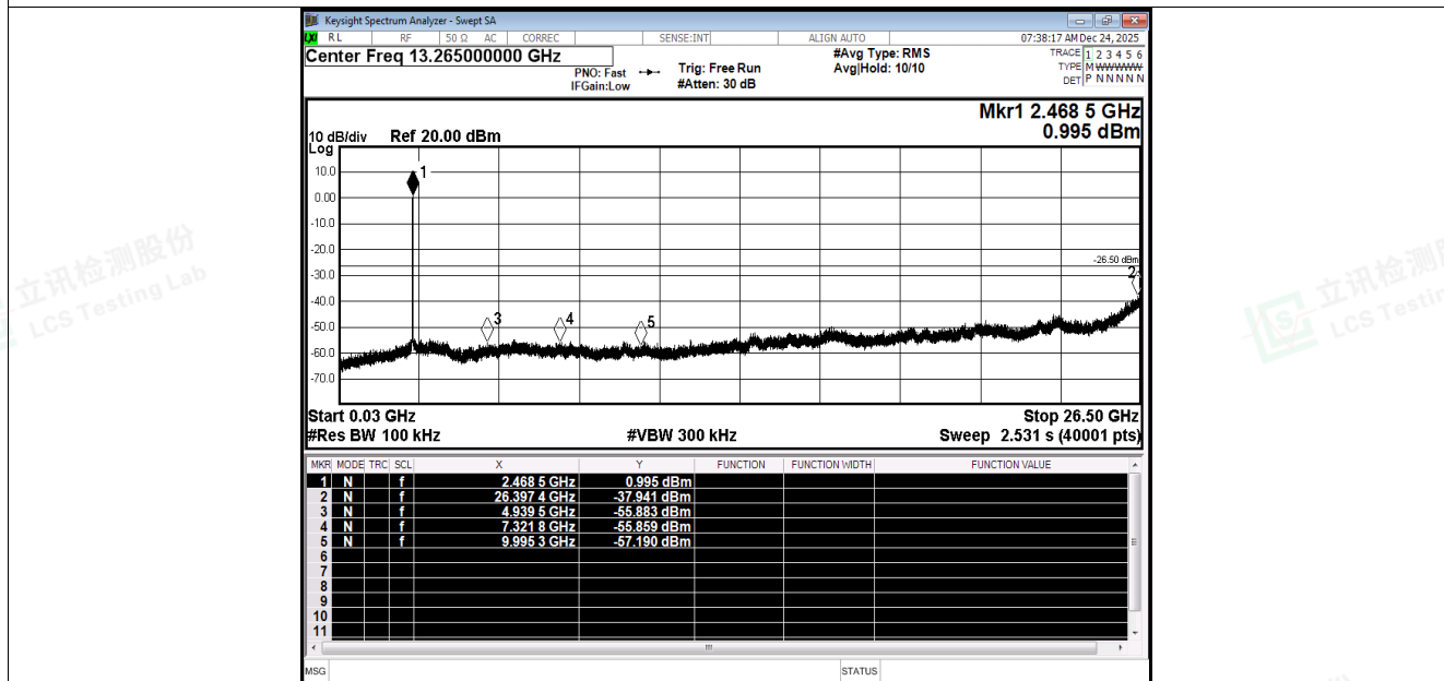
Tx. Spurious NVNT n20 2462MHz Ant1 Emission
