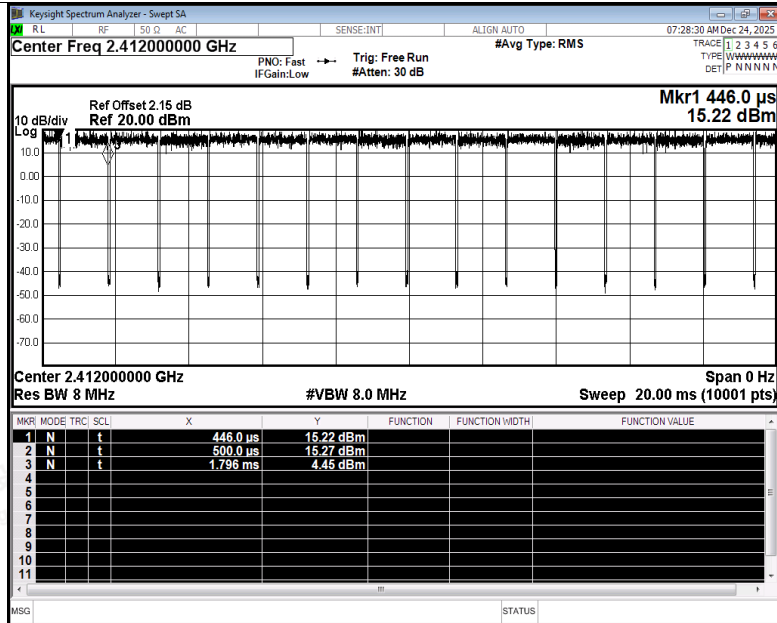
Duty Cycle NVNT n20 2412MHz Ant1
