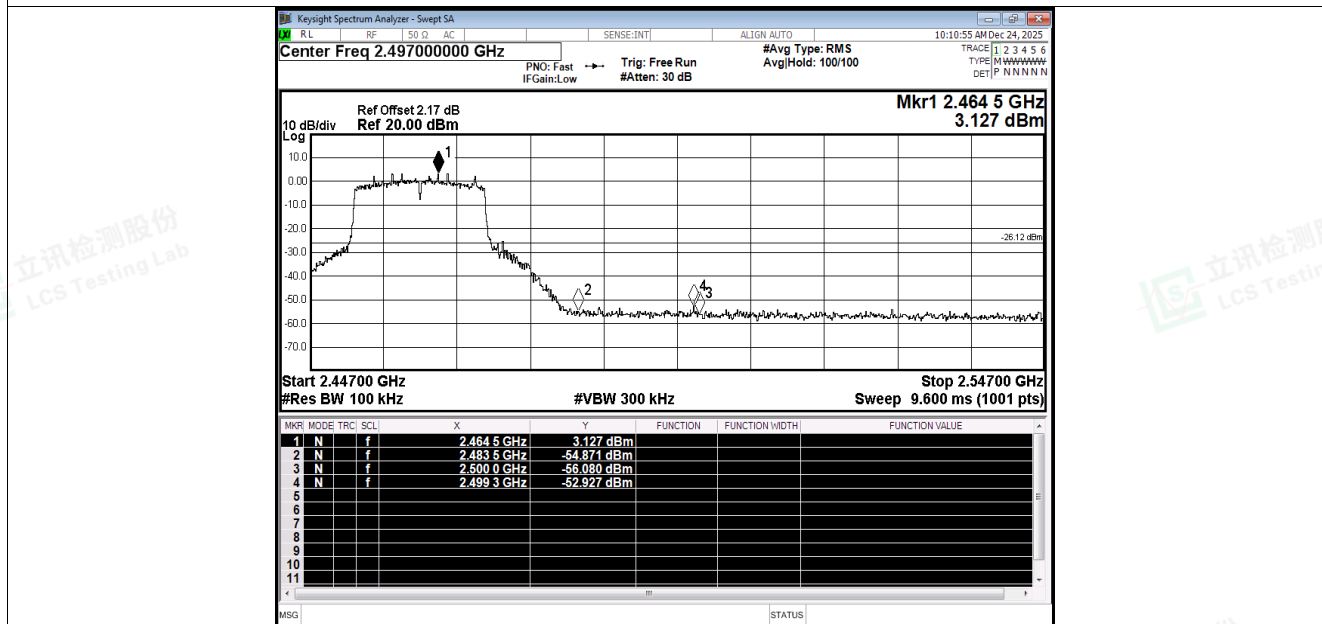
Band Edge NVNT n20 2462MHz Ant3 Emission
