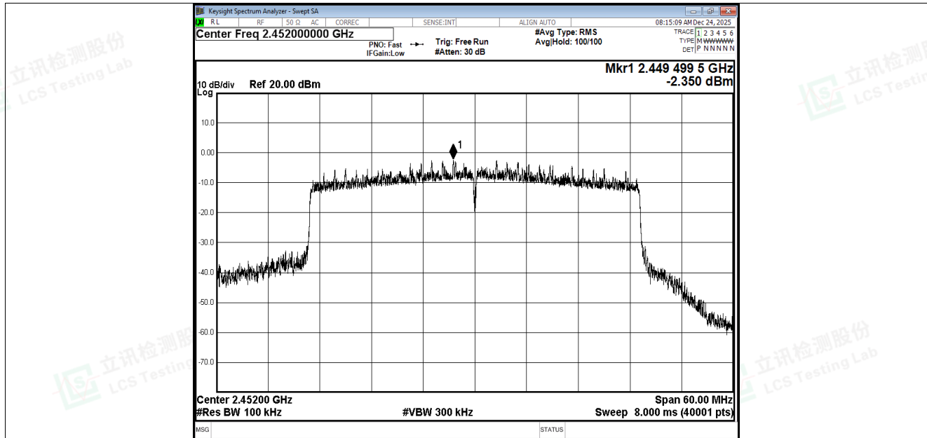
Tx. Spurious NVNT ax40 2452MHz Ant1 Ref
