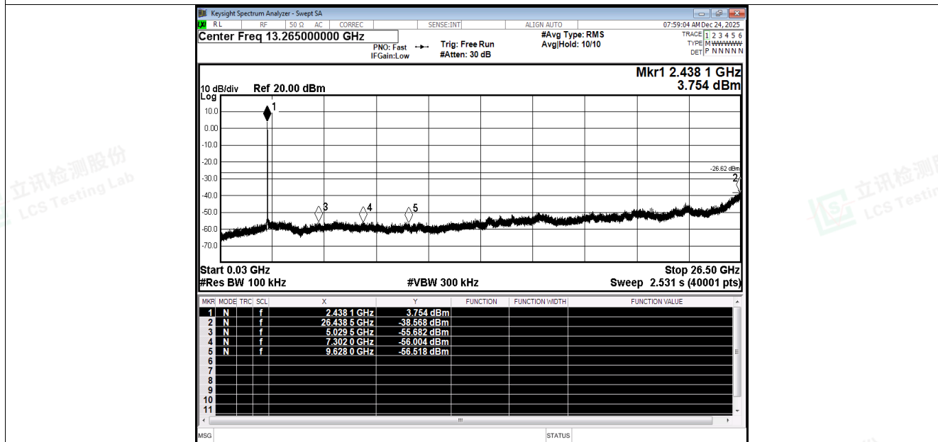
Tx. Spurious NVNT ax20 2437MHz Ant1 Emission
