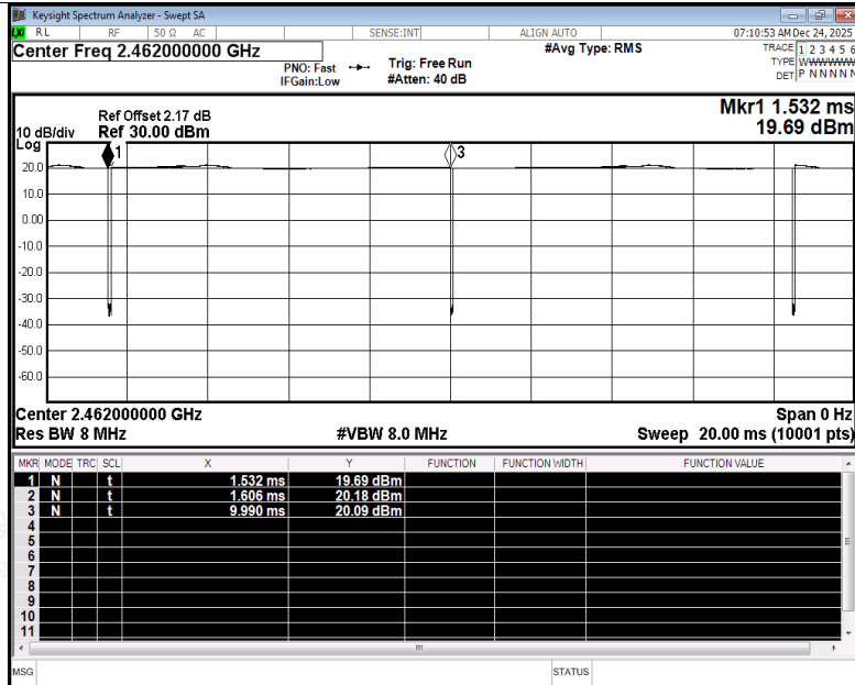
Duty Cycle NVNT b 2462MHz Ant1
