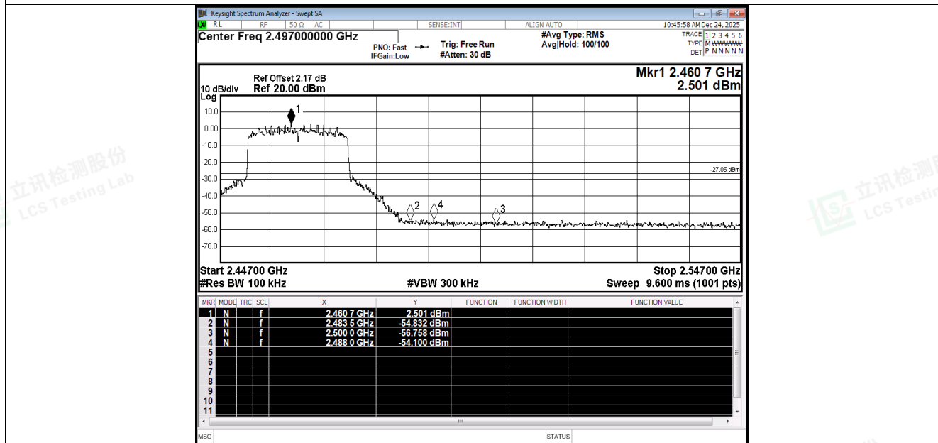
Band Edge NVNT be20 2462MHz Ant3 Emission
