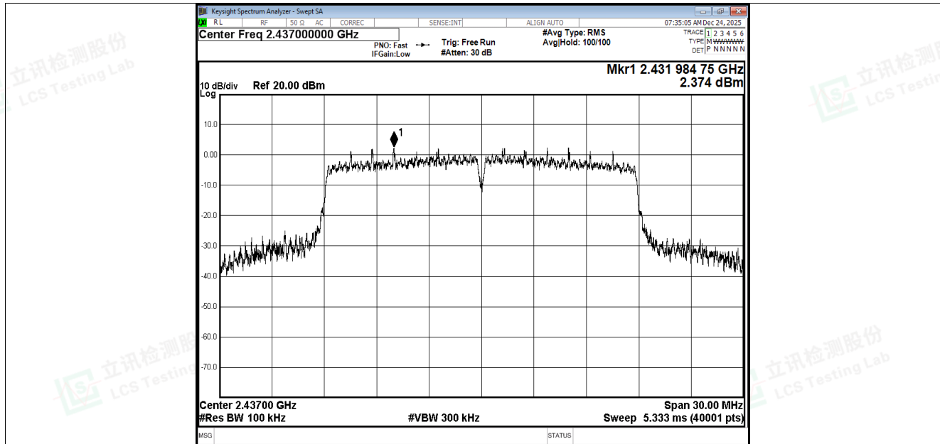
Tx. Spurious NVNT n20 2437MHz Ant1 Ref
