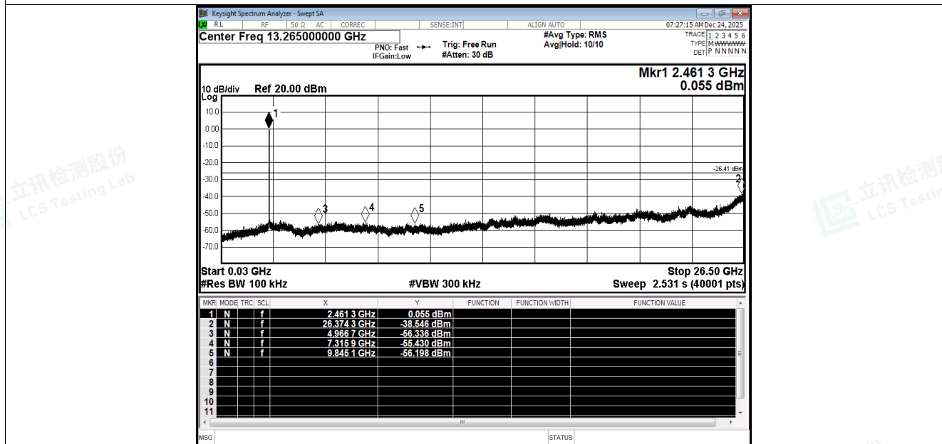
Tx. Spurious NVNT g 2462MHz Ant1 Emission
