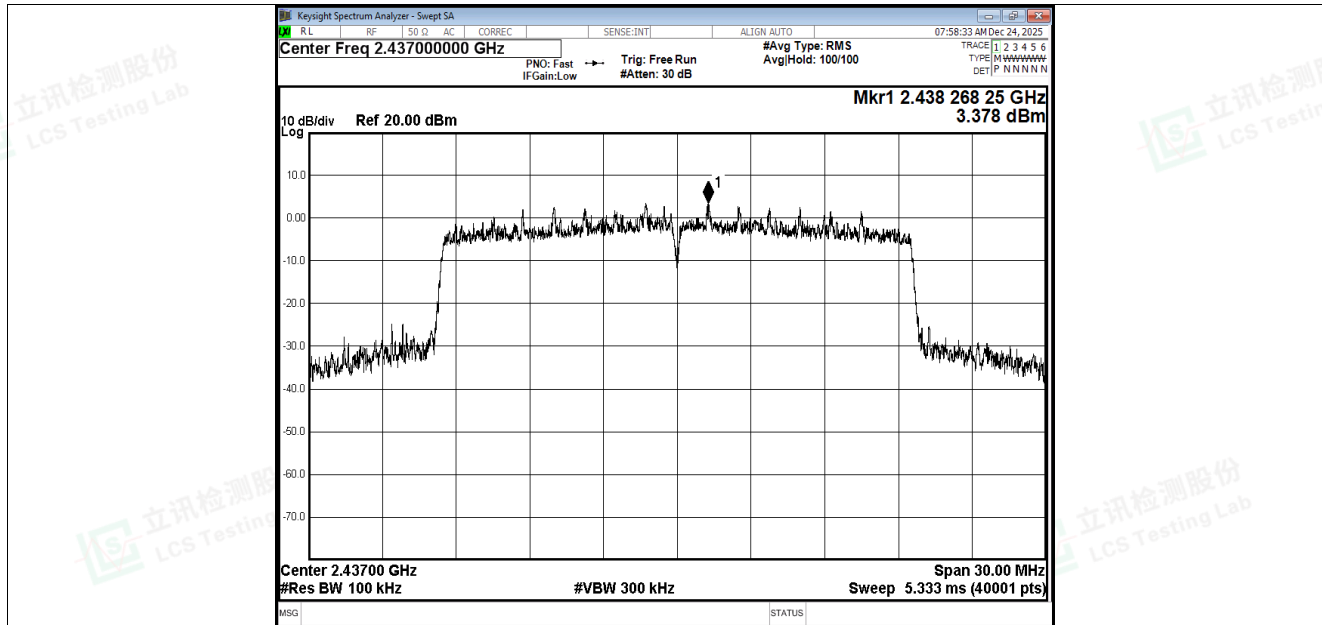
Tx. Spurious NVNT ax20 2437MHz Ant1 Ref
