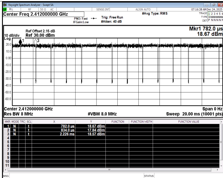
Duty Cycle NVNT g 2412MHz Ant1
