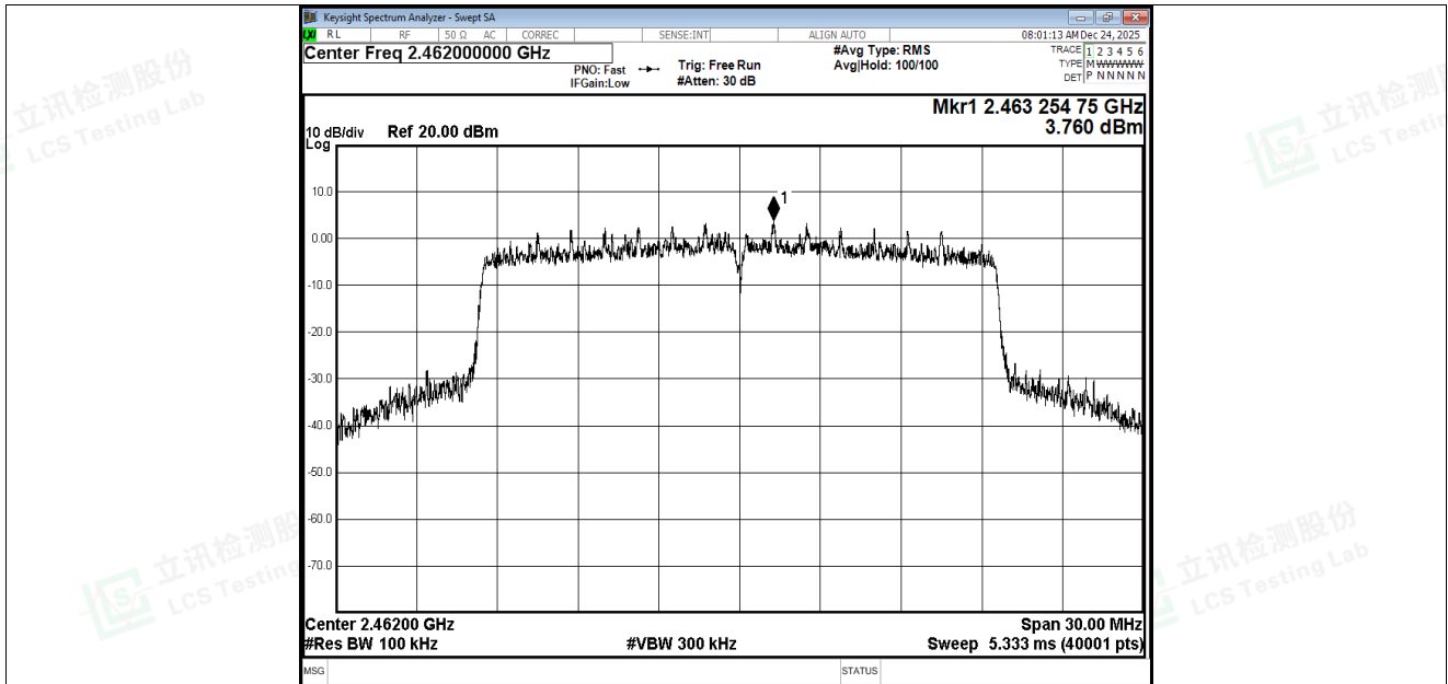
Tx. Spurious NVNT ax20 2462MHz Ant1 Ref
