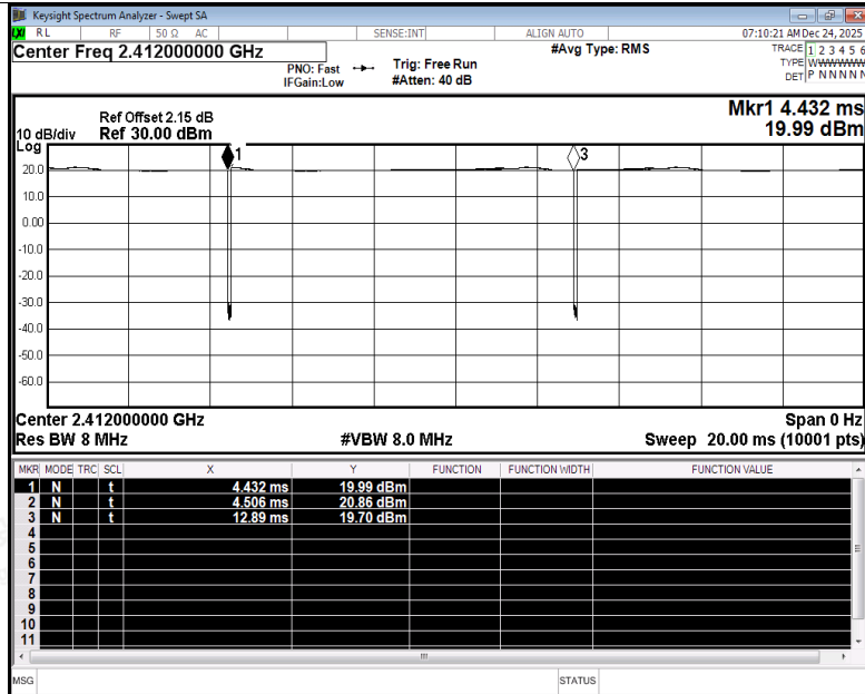
Duty Cycle NVNT b 2412MHz Ant1
