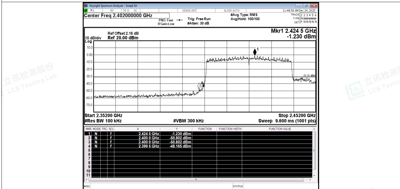
Band Edge NVNT ax40 2422MHz Ant4 Emission
