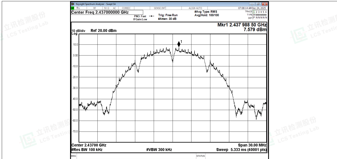
Tx. Spurious NVNT b 2437MHz Ant1 Ref
