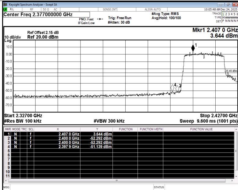
Band Edge NVNT n20 2412MHz Ant3 Emission
