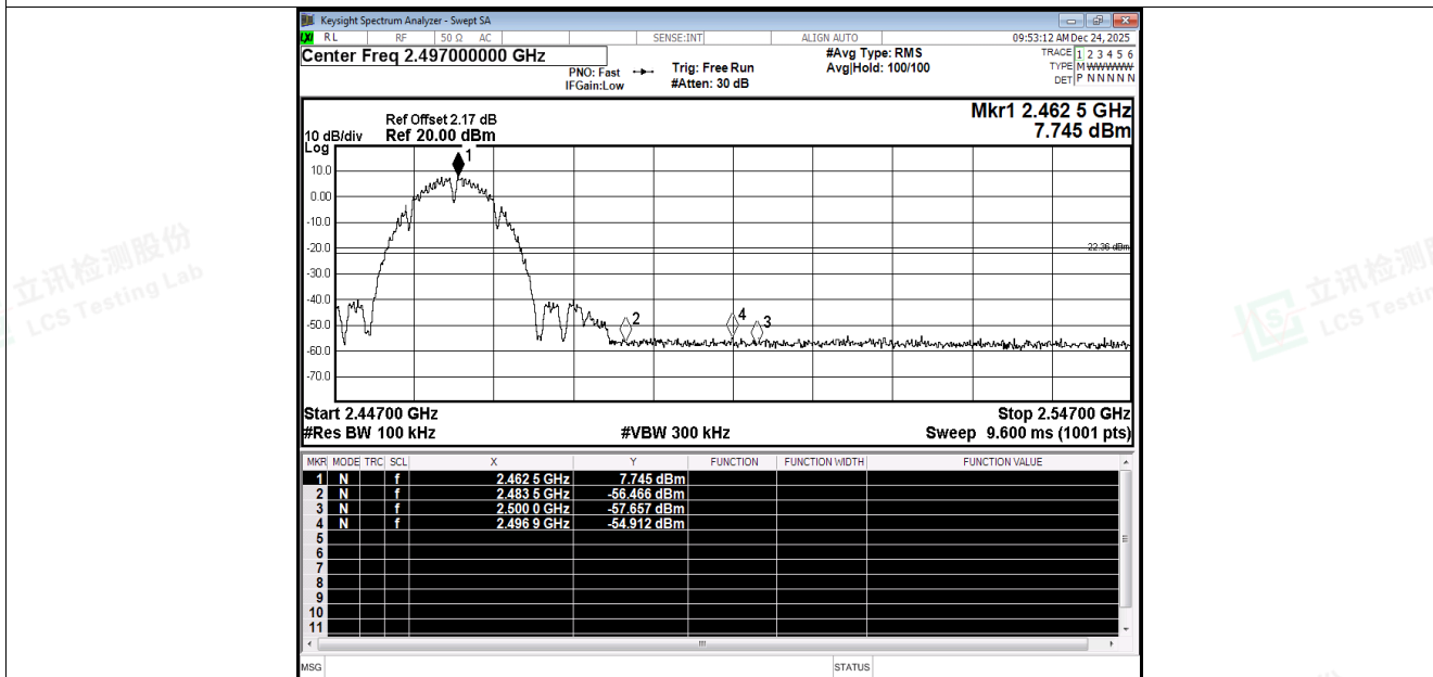
Band Edge NVNT b 2462MHz Ant3 Emission
