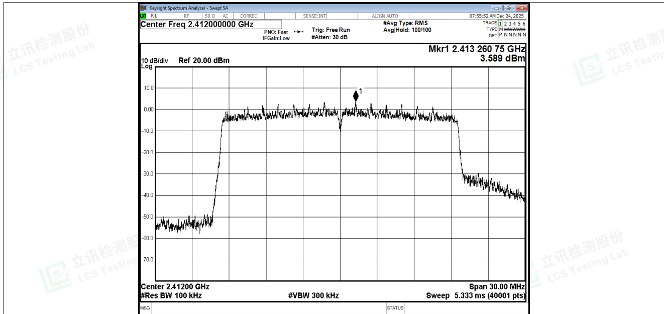
Tx. Spurious NVNT ax20 2412MHz Ant1 Ref
