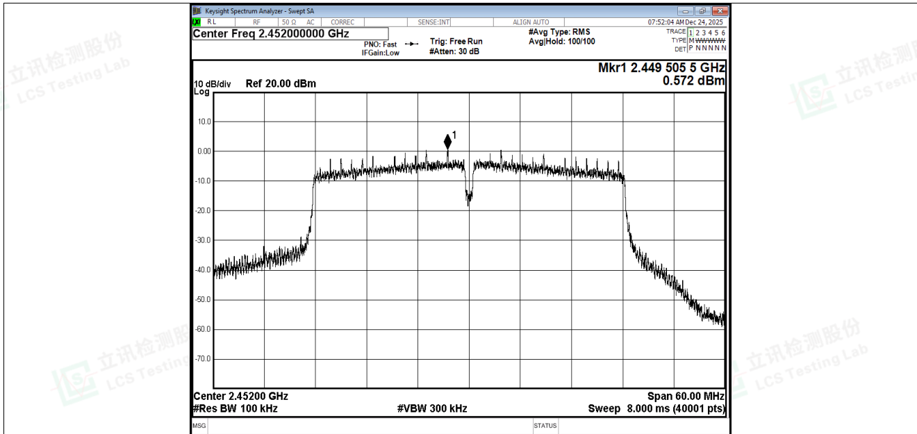
Tx. Spurious NVNT n40 2452MHz Ant1 Ref
