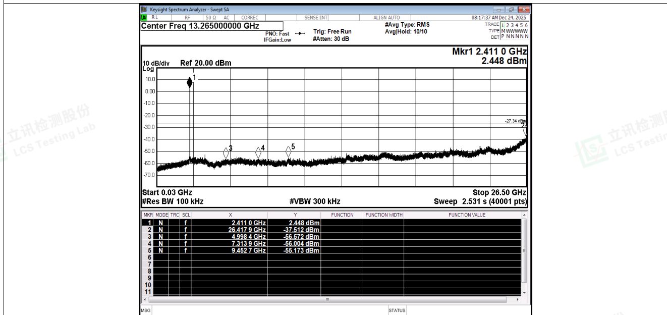
Tx. Spurious NVNT be20 2412MHz Ant1 Emission
