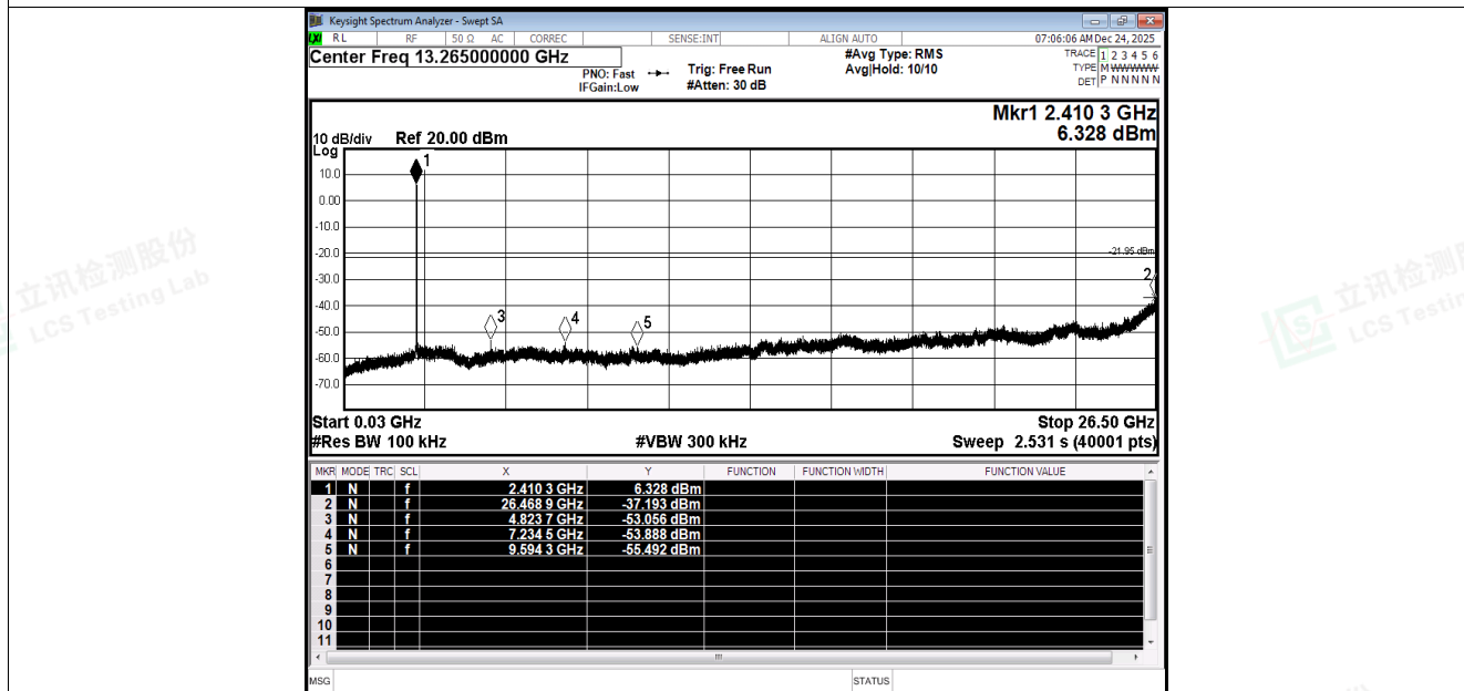
Tx. Spurious NVNT b 2412MHz Ant1 Emission
