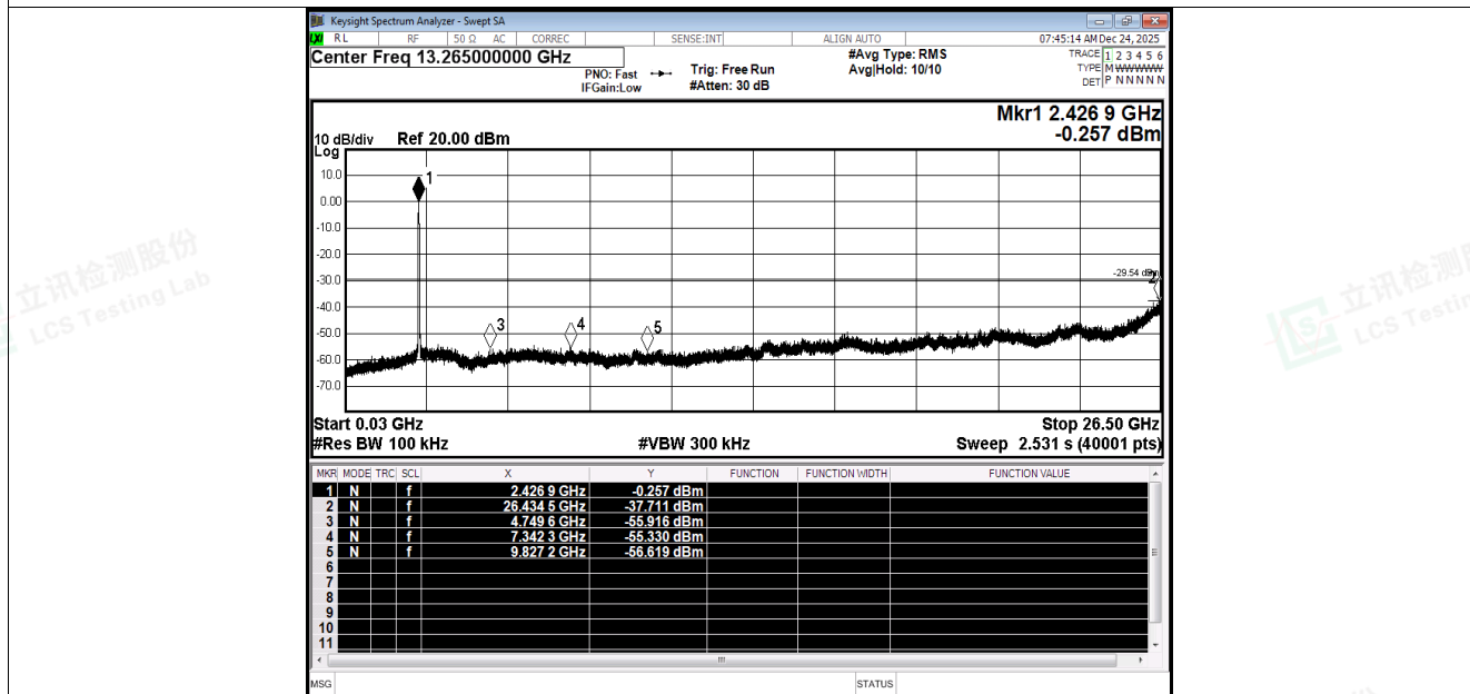
Tx. Spurious NVNT n40 2422MHz Ant1 Emission
