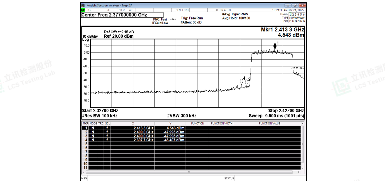
Band Edge NVNT ax20 2412MHz Ant3 Emission
