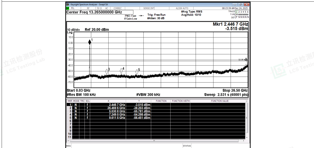
Tx. Spurious NVNT ax40 2452MHz Ant1 Emission
