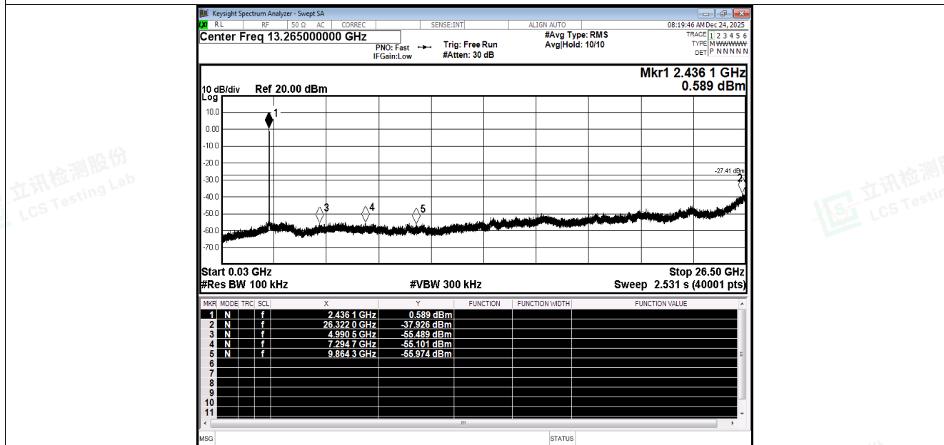
Tx. Spurious NVNT be20 2437MHz Ant1 Emission
