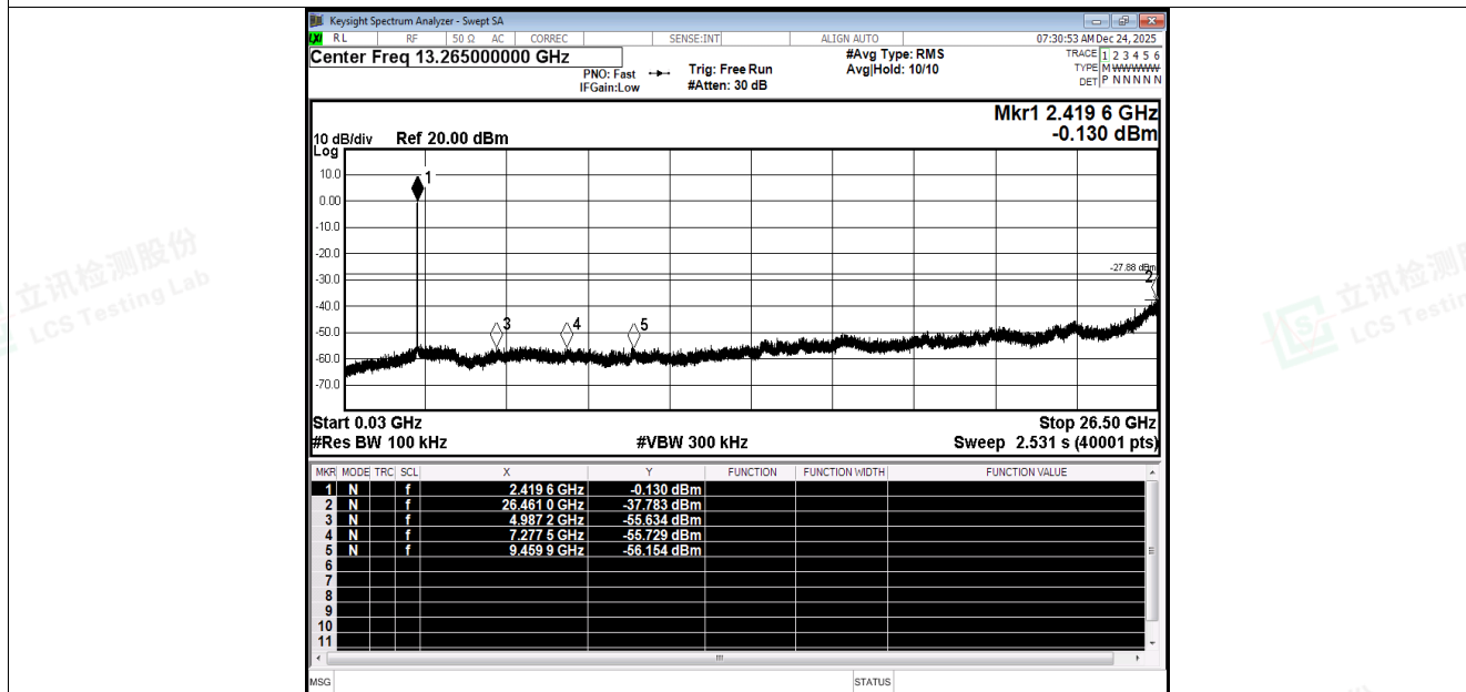
Tx. Spurious NVNT n20 2412MHz Ant1 Emission
