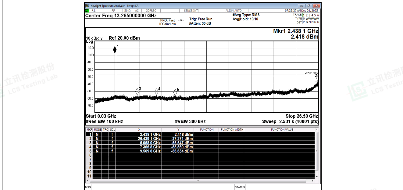
Tx. Spurious NVNT n20 2437MHz Ant1 Emission
