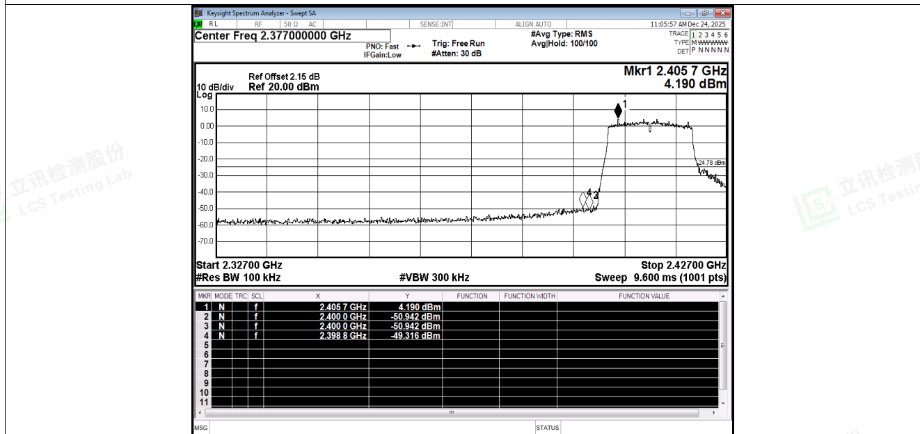
Band Edge NVNT g 2412MHz Ant4 Emission
