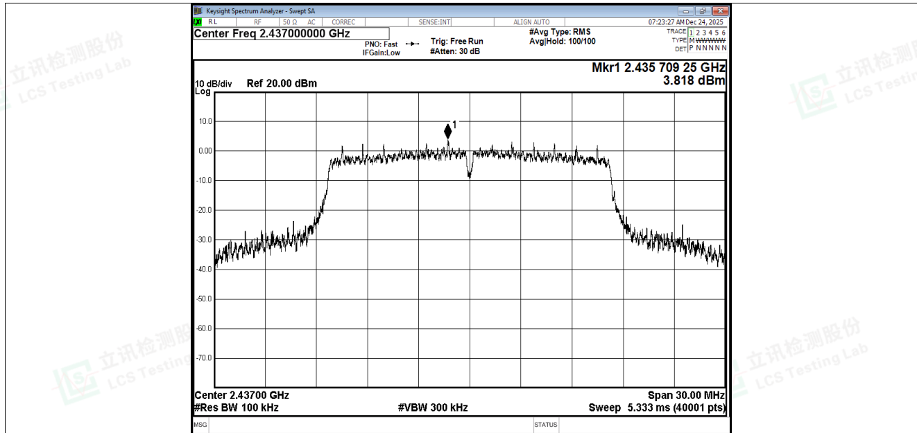
Tx. Spurious NVNT g 2437MHz Ant1 Ref
