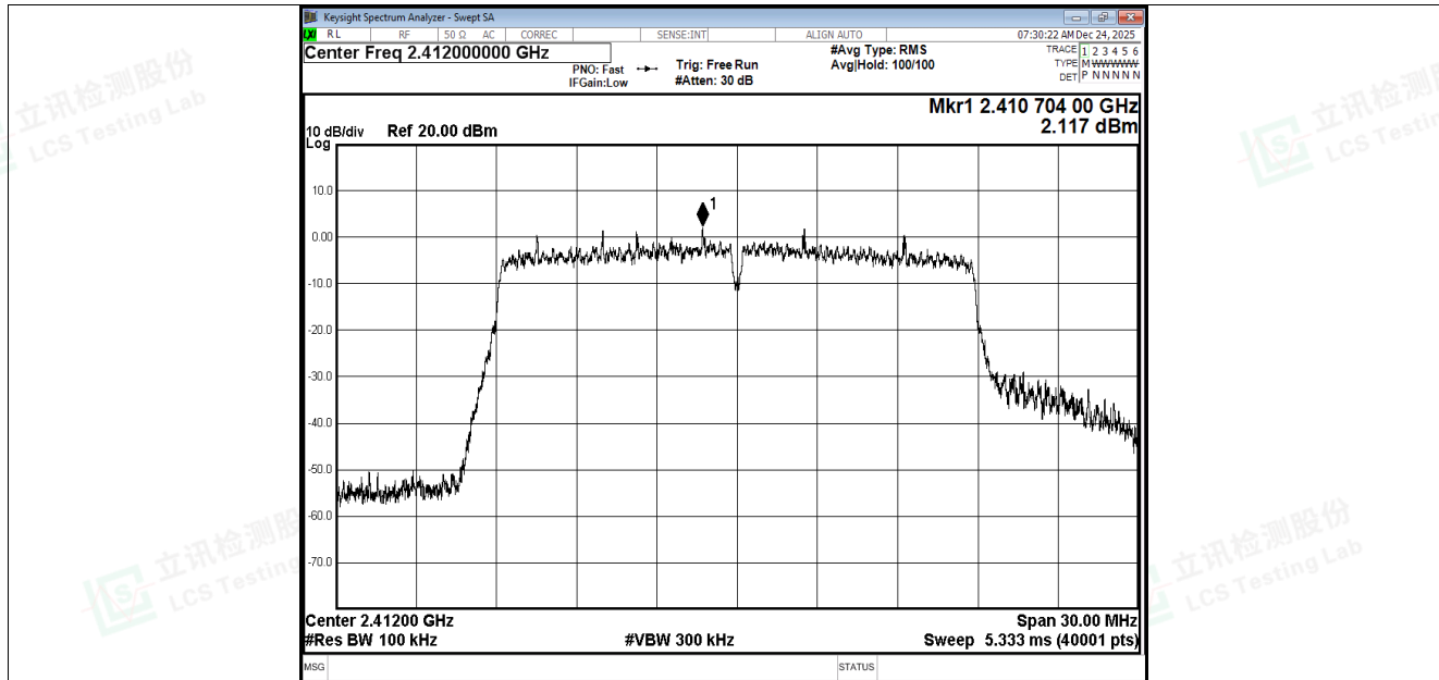
Tx. Spurious NVNT n20 2412MHz Ant1 Ref
