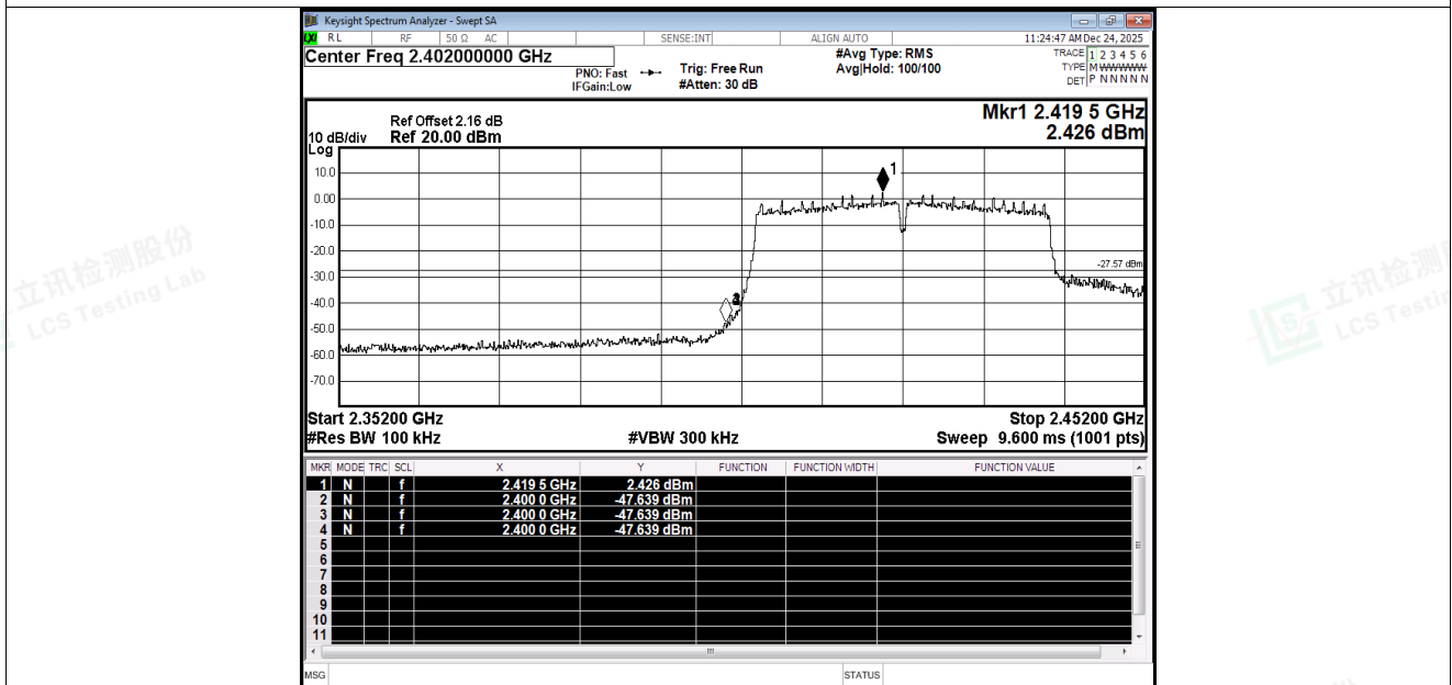
Band Edge NVNT n40 2422MHz Ant4 Emission
