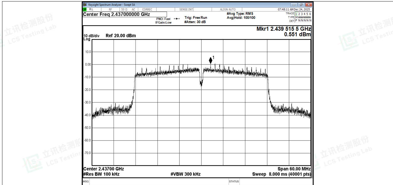
Tx. Spurious NVNT n40 2437MHz Ant1 Ref
