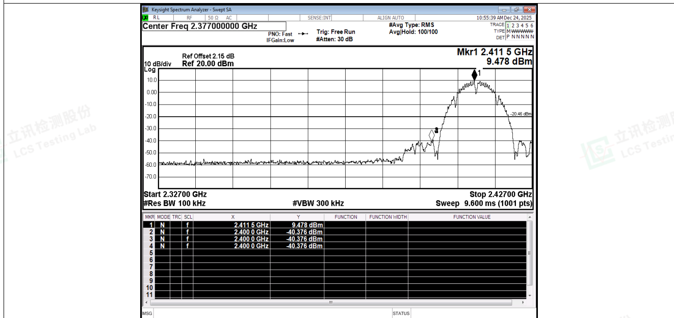
Band Edge NVNT b 2412MHz Ant4 Emission
