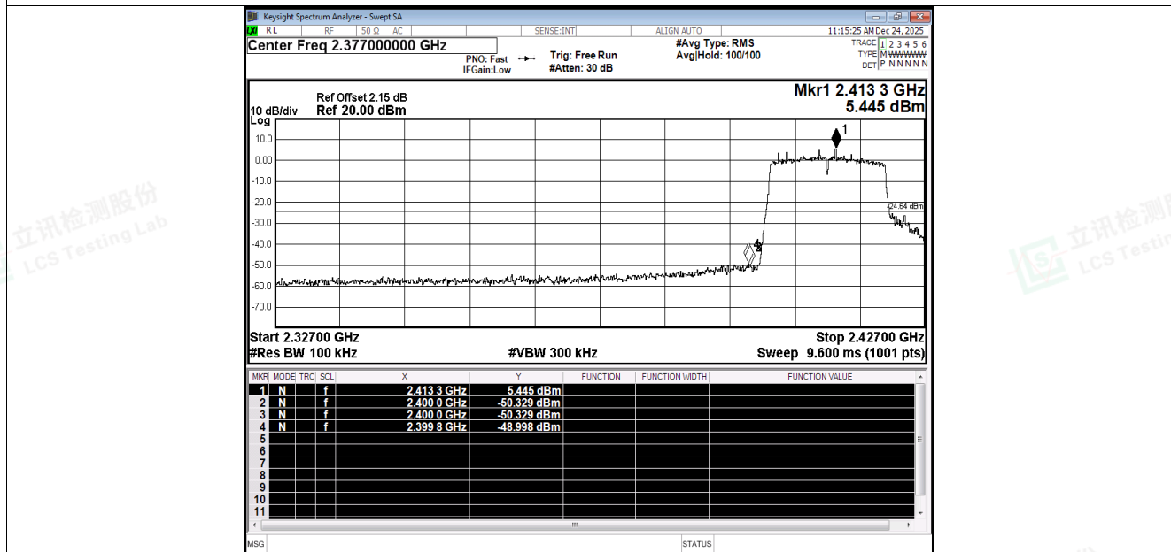
Band Edge NVNT n20 2412MHz Ant4 Emission
