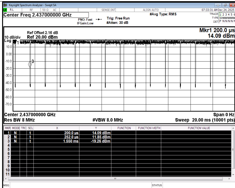
Duty Cycle NVNT n20 2437MHz Ant1
