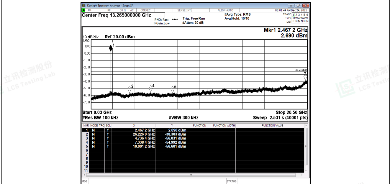
Tx. Spurious NVNT ax20 2462MHz Ant1 Emission
