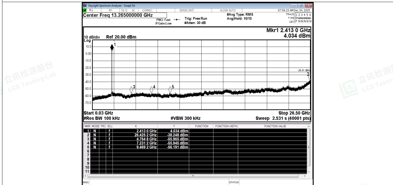
Tx. Spurious NVNT ax20 2412MHz Ant1 Emission
