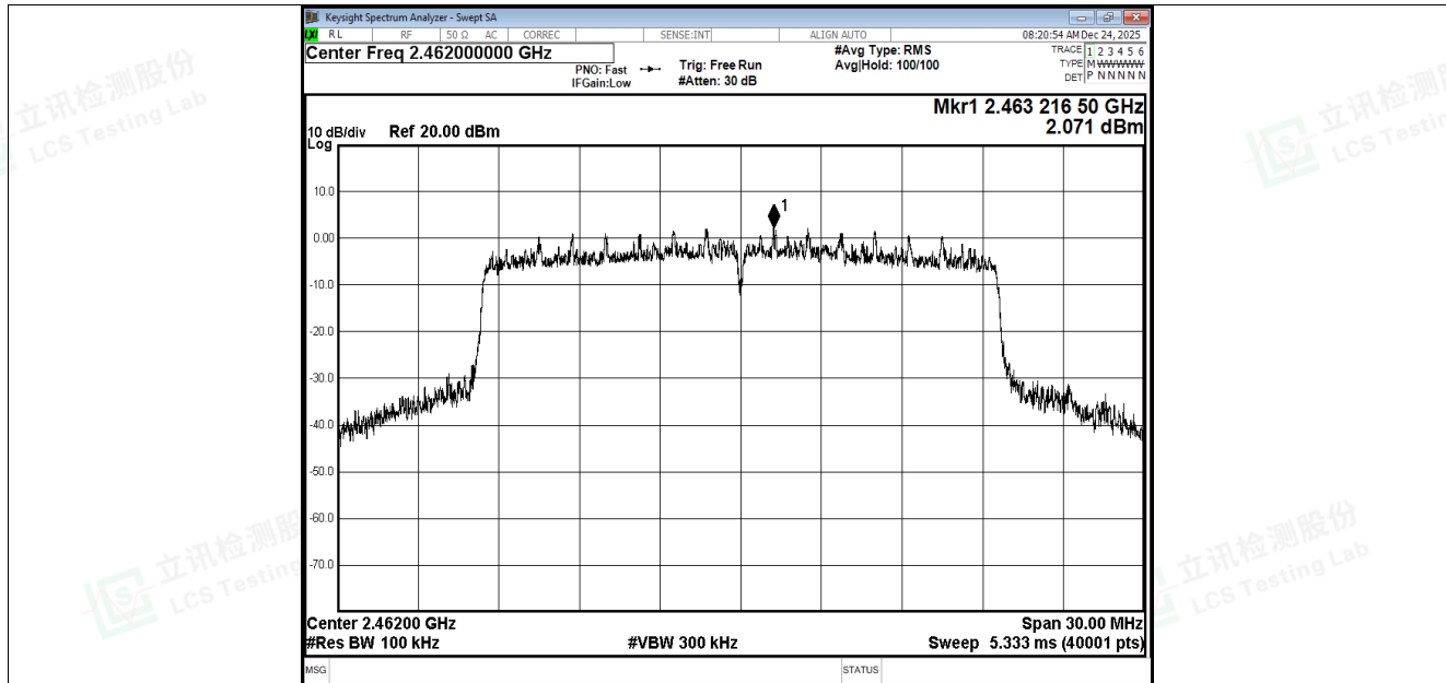
Tx. Spurious NVNT be20 2462MHz Ant1 Ref
