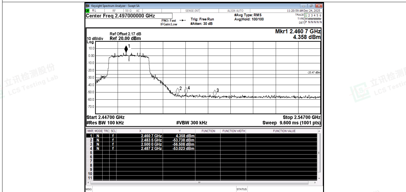
Band Edge NVNT n20 2462MHz Ant4 Emission
