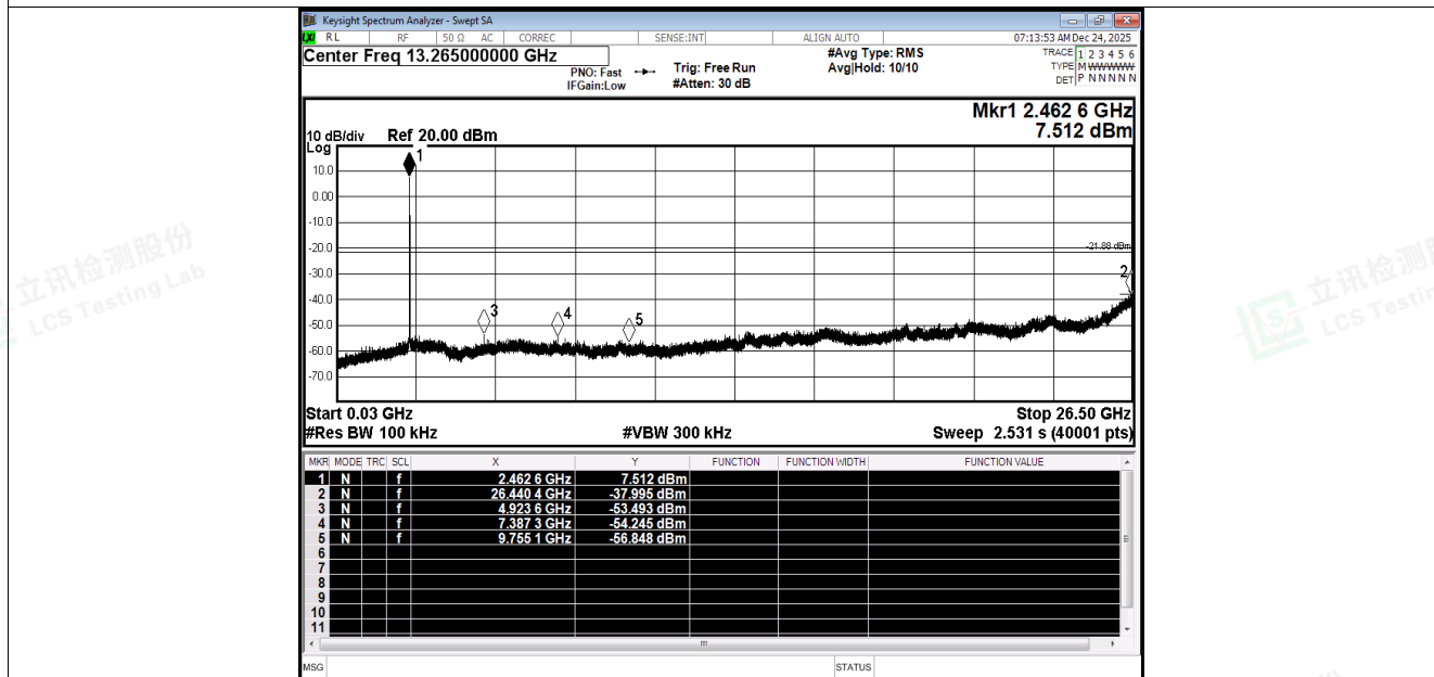
Tx. Spurious NVNT b 2462MHz Ant1 Emission
