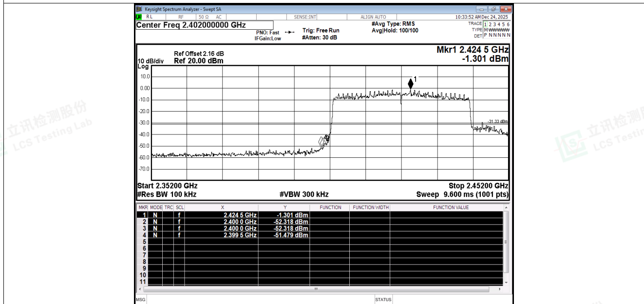
Band Edge NVNT ax40 2422MHz Ant3 Emission
