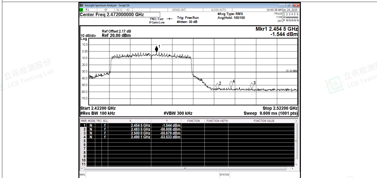
Band Edge NVNT ax40 2452MHz Ant3 Emission
