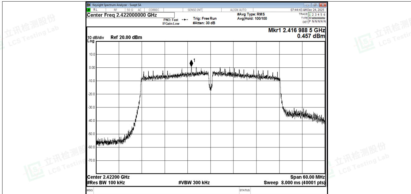
Tx. Spurious NVNT n40 2422MHz Ant1 Ref
