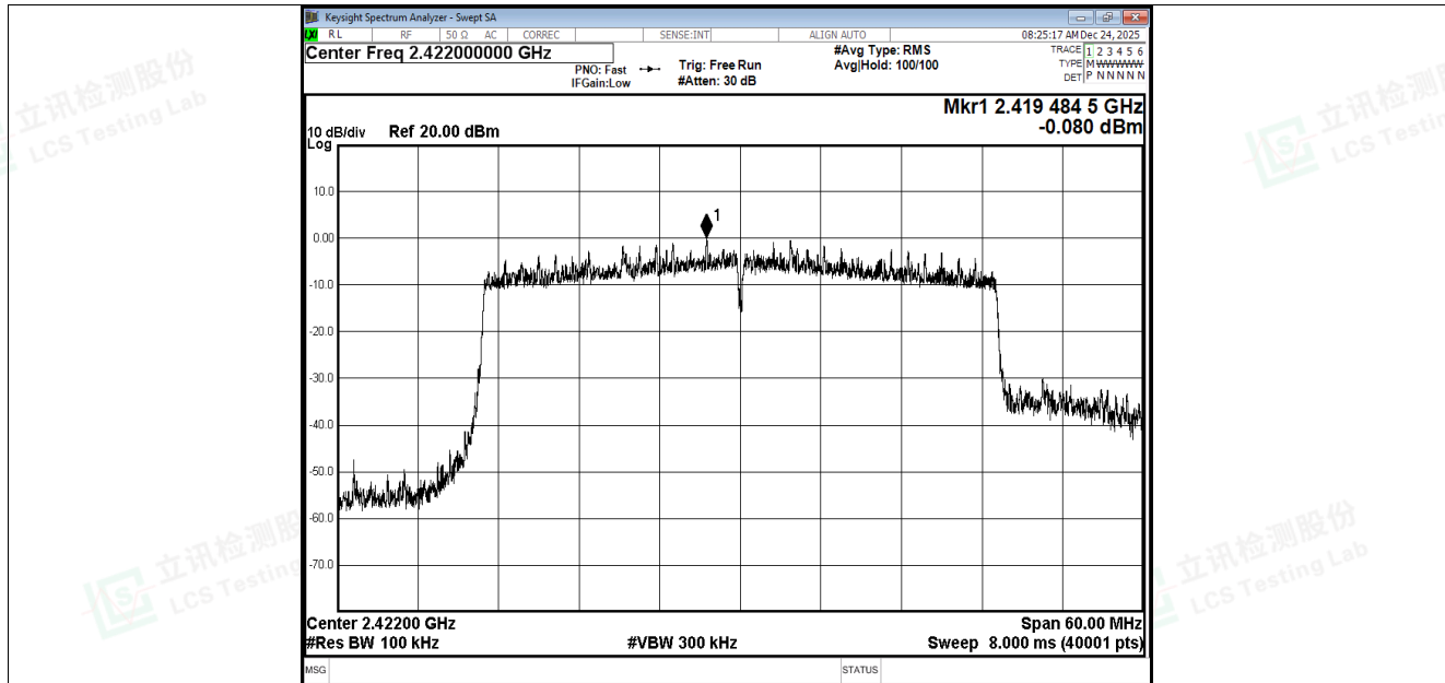
Tx. Spurious NVNT be40 2422MHz Ant1 Ref
