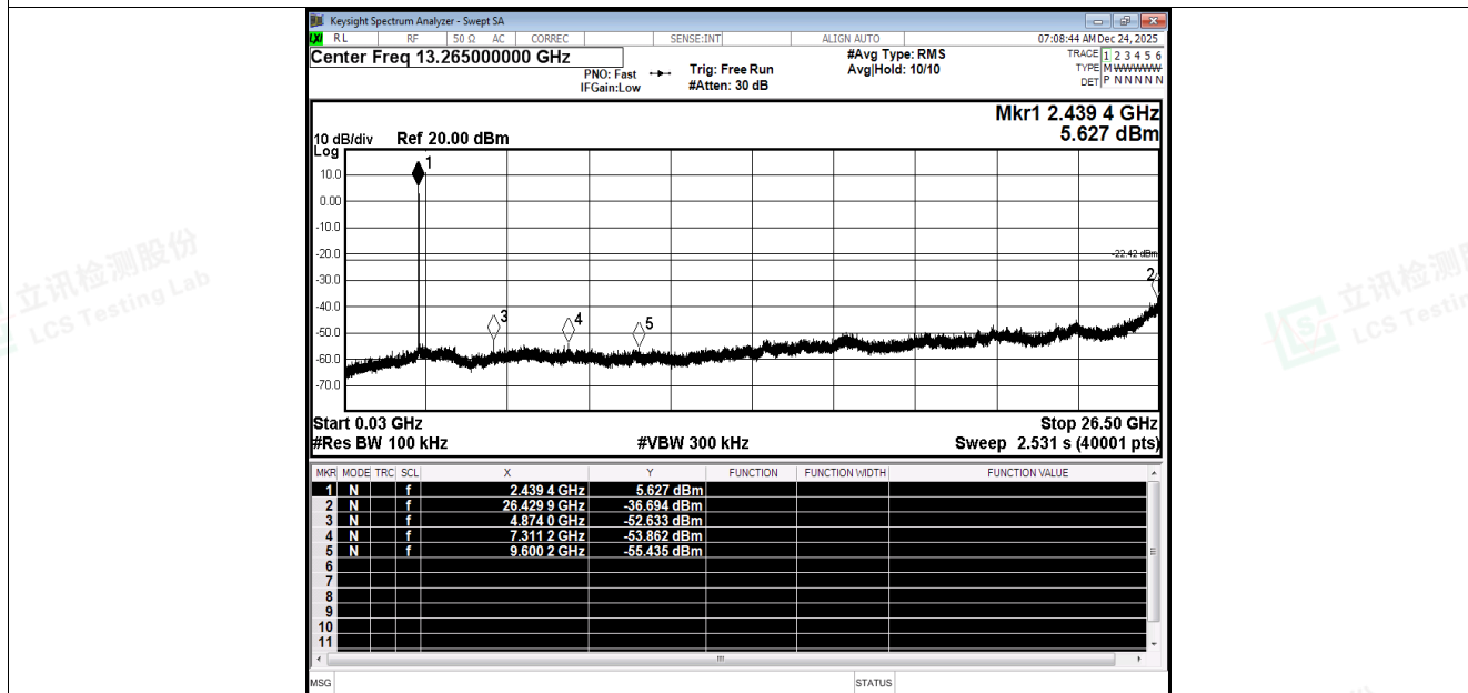
Tx. Spurious NVNT b 2437MHz Ant1 Emission
