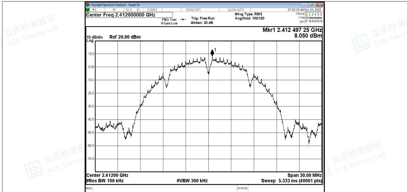
Tx. Spurious NVNT b 2412MHz Ant1 Ref
