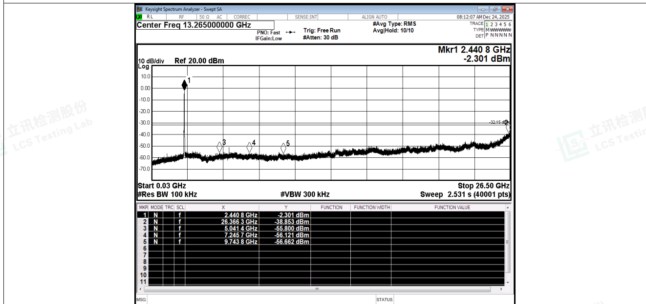
Tx. Spurious NVNT ax40 2437MHz Ant1 Emission
