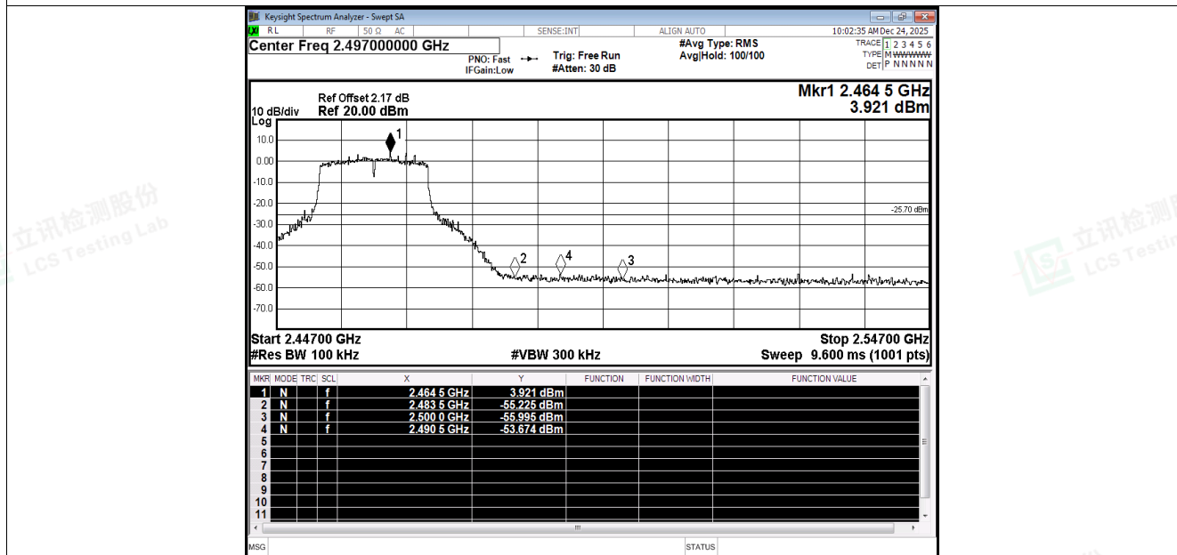
Band Edge NVNT g 2462MHz Ant3 Emission
