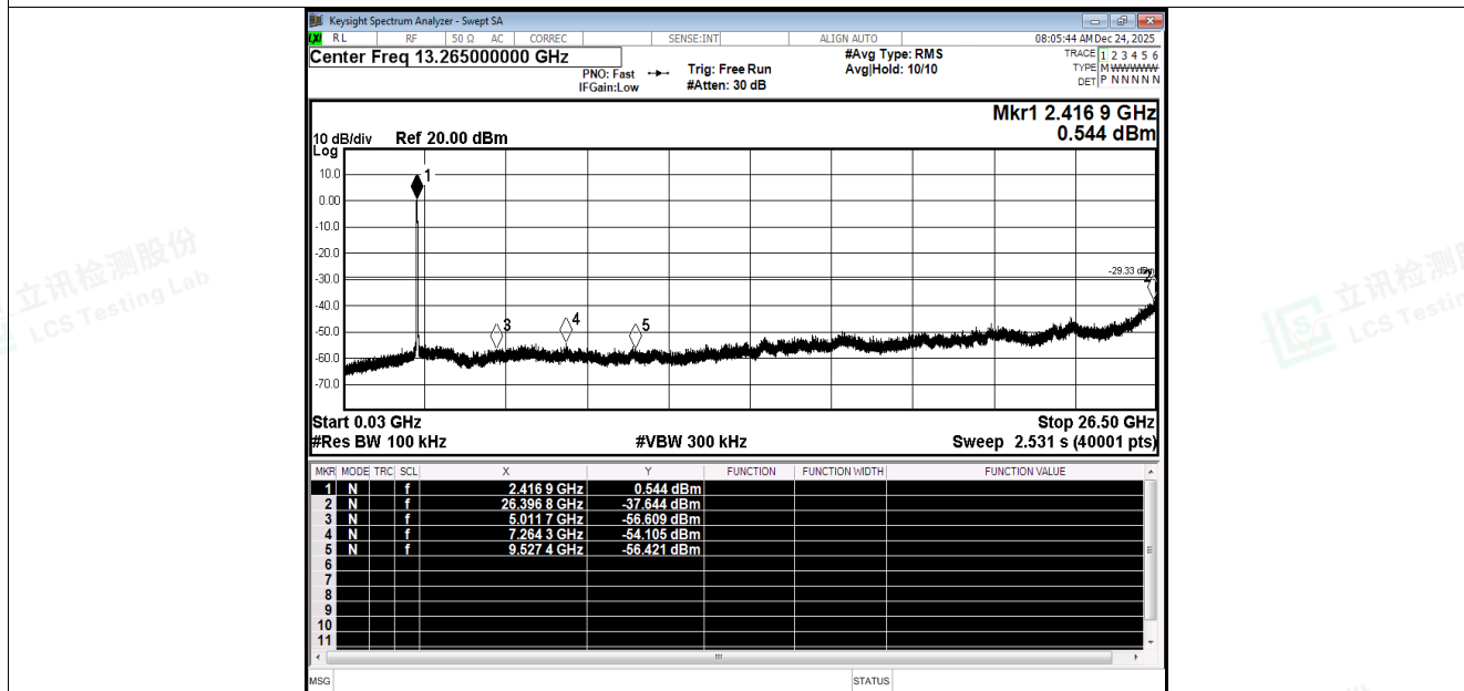
Tx. Spurious NVNT ax40 2422MHz Ant1 Emission
